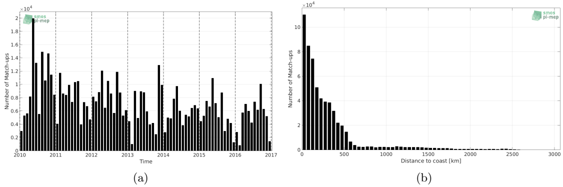
Figure 1: Number of match-ups between TSG-LEGOS-DM and SMOS-L3-CATDS-CECOS-LOCEAN-V3-18DAYS-25KM SSS as a function of time (a) and as function of the distance to coast (b) over the South Pacific Ocean Pi-MEP region and for the full satellite product period.
