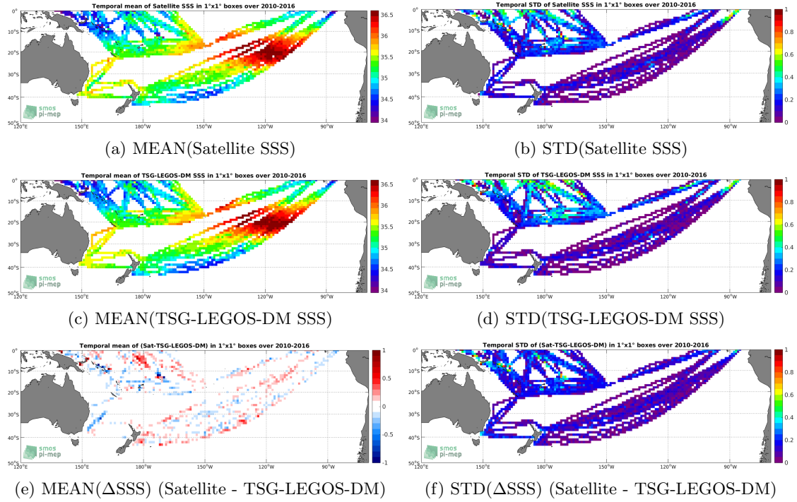
Figure 6: Temporal mean (left) and STD (right) of SSS from SMOS-L3-CATDS-CECOS-LOCEAN-V3-18DAYS-25KM (top), TSG-LEGOS-DM (middle), and of \Delta SSS (Satellite - TSG-LEGOS-DM). Only match-up pairs are used to generate these maps.
