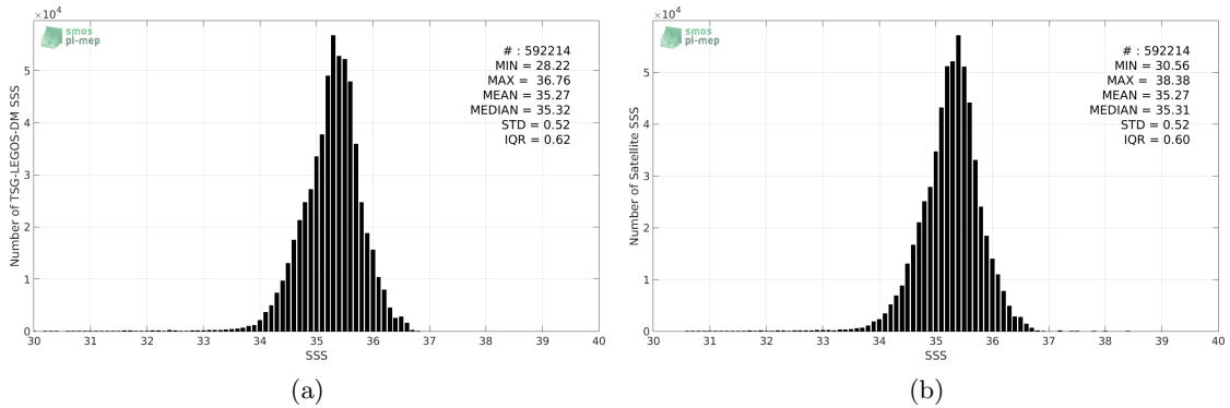
Figure 2: Histograms of SSS from TSG-LEGOS-DM (a) and SMOS-L3-CATDS-CECOS-LOCEAN-V3-18DAYS-25KM (b) considering all match-up pairs per bins of 0.1 over the South Pacific Ocean Pi-MEP region and for the full satellite product period.
