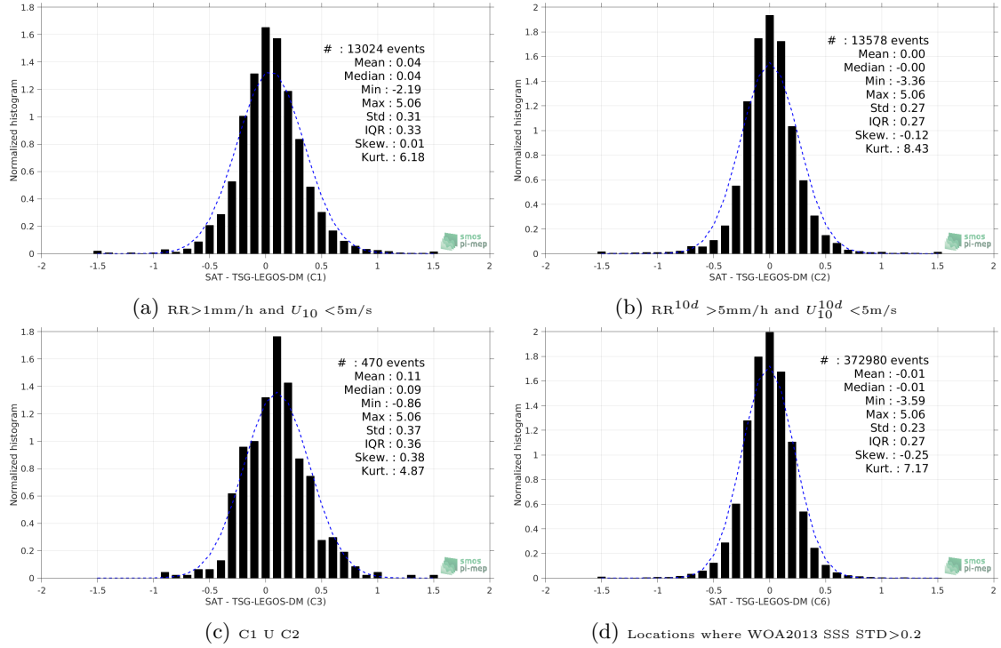
Figure 13: Normalized histogram of \Delta SSS (SMOS-L3-CATDS-CECOS-LOCEAN-V3-18DAYS-25KM - TSG-LEGOS-DM) for 6 different subdatasets corresponding to: RR > 1mm/h and U_{10} < 5 m/s (a), RR^{10d} > 5 mm/h and U_{10}^{10d} < 5 m/s (b), C1 U C2 (c), Locations where WOA2013 SSS STD > 0.2 (d).
