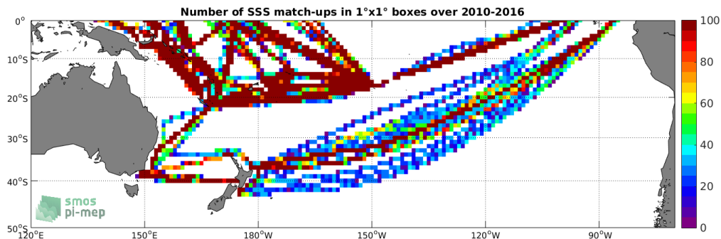
Figure 4: Number of SSS match-ups between TSG-LEGOS-DM SSS and the SMOS-L3-CATDS-CECOS-LOCEAN-V3-18DAYS-25KM SSS product for the South Pacific Ocean Pi-MEP region over 1^\circ \times 1^\circ boxes and for the full satellite product period.
