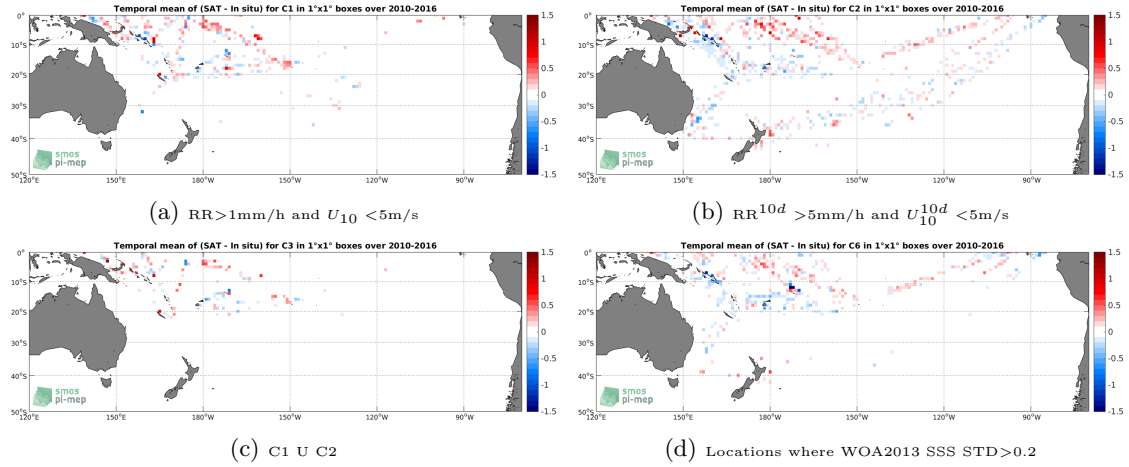
Figure 12: Temporal mean gridded over spatial boxes of size 1^\circ \times 1^\circ of \Delta SSS (SMOS-L3-CATDS-CECOS-LOCEAN-V3-18DAYS-25KM - TSG-LEGOS-DM) for 4 different subdatasets corresponding to: RR > 1\text{mm/h} and U_{10} < 5\text{m/s} (a), RR^{10d} > 5\text{mm/h} and U_{10}^{10d} < 5\text{m/s} (b), C1 U C2 (c), Locations where WOA2013 SSS STD > 0.2 (d).
