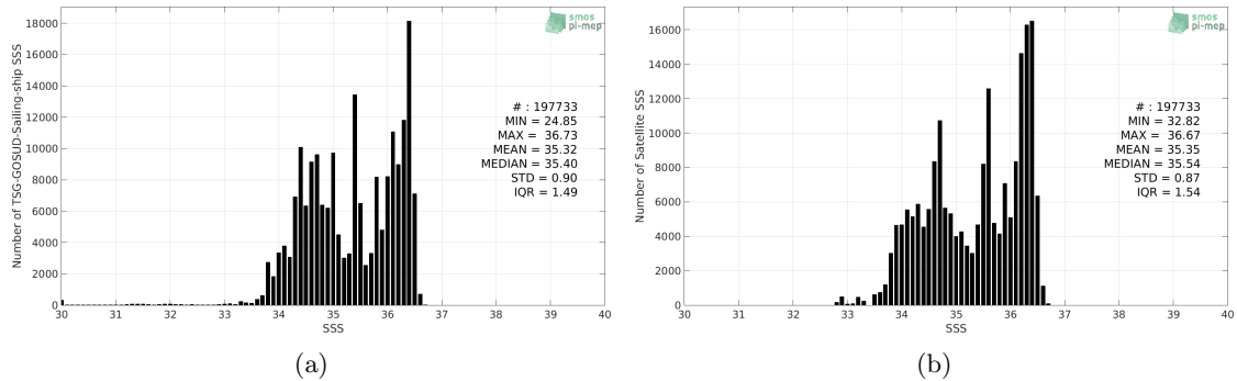
Figure 2: Histograms of SSS from TSG-GOSUD-Sailing-ship (a) and SMOS-L3-CATDS-CECOS-LOCEAN-V3-18DAYS-25KM (b) considering all match-up pairs per bins of 0.1 over the South Pacific Ocean Pi-MEP region and for the full satellite product period.
