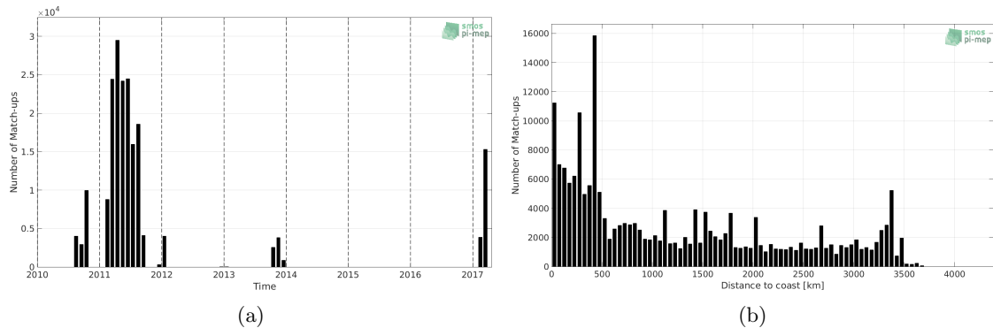
Figure 1: Number of match-ups between TSG-GOSUD-Sailing-ship and SMOS-L3-CATDS-CECOS-LOCEAN-V3-18DAYS-25KM SSS as a function of time (a) and as function of the distance to coast (b) over the South Pacific Ocean Pi-MEP region and for the full satellite product period.
