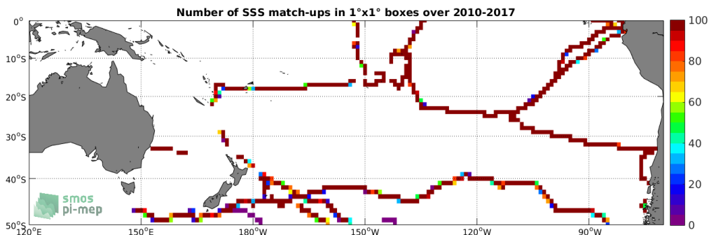
Figure 4: Number of SSS match-ups between TSG-GOSUD-Sailing-ship SSS and the SMOS-L3-CATDS-CECOS-LOCEAN-V3-18DAYS-25KM SSS product for the South Pacific Ocean Pi-MEP region over 1°x1° boxes and for the full satellite product period.
