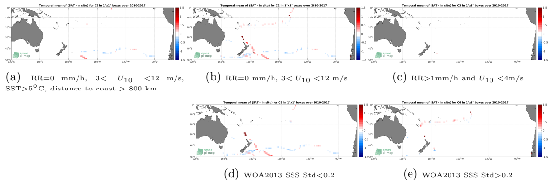
Figure 12: Temporal mean gridded over spatial boxes of size 1^\circ \times 1^\circ of \Delta SSS (SMOS-L3-CATDS-CECOS-LOCEAN-V3-18DAYS-25KM - TSG-GOSUD-Sailing-ship) for 5 different subdatasets corresponding to:RR=0 mm/h, 3 < U_{10} < 12 m/s, SST >5^\circ C, distance to coast > 800 km (a), RR=0 mm/h, 3 < U_{10} < 12 m/s (b), RR >1 mm/h and U_{10} < 4 m/s (c), WOA2013 SSS Std <0.2 (d), WOA2013 SSS Std >0.2 (e).
