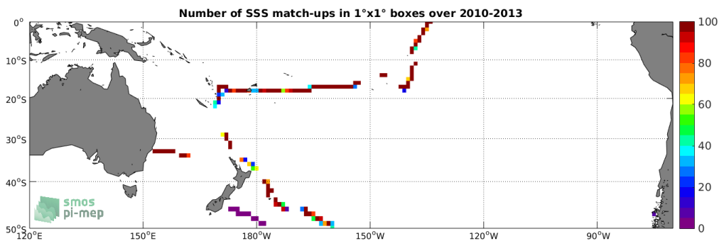
Figure 4: Number of SSS match-ups between TSG-GOSUD-Sailing-ship SSS and the SMOS-L3-CATDS-CECOS-LOCEAN-V3-18DAYS-25KM SSS product for the South Pacific Ocean Pi-MEP region over 1^\circ \times 1^\circ boxes and for the full satellite product period.
