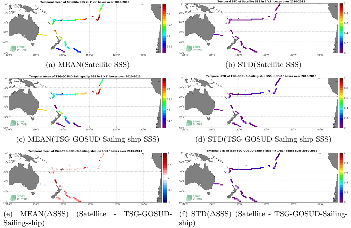
Figure 6: Temporal mean (left) and STD (right) of SSS from SMOS-L3-CATDS-CECOS-LOCEAN-V3-18DAYS-25KM (top), TSG-GOSUD-Sailing-ship (middle), and of \Delta SSS (Satellite - TSG-GOSUD-Sailing-ship). Only match-up pairs are used to generate these maps.
