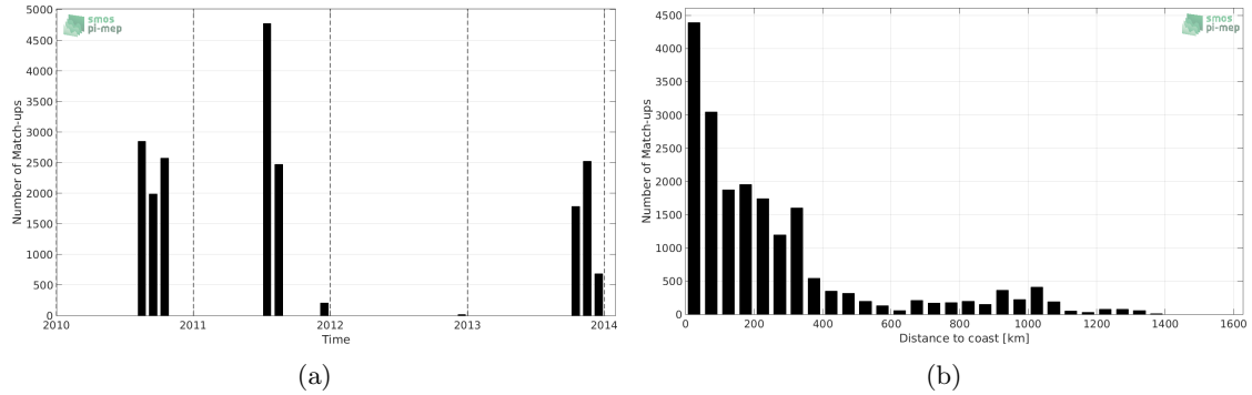
Figure 1: Number of match-ups between TSG-GOSUD-Sailing-ship and SMOS-L3-CATDS-CECOS-LOCEAN-V3-18DAYS-25KM SSS as a function of time (a) and as function of the distance to coast (b) over the South Pacific Ocean Pi-MEP region and for the full satellite product period.
