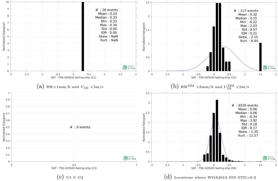
Figure 13: Normalized histogram of \Delta SSS (SMOS-L3-CATDS-CECOS-LOCEAN-V3-18DAYS-25KM - TSG-GOSUD-Sailing-ship) for 6 different subdatasets corresponding to: RR > 1mm/h and U_{10} < 5 m/s (a), RR 10d > 5mm/h and U_{10}^{10d} < 5 m/s (b), C1 U C2 (c), Locations where WOA2013 SSS STD > 0.2 (d).
