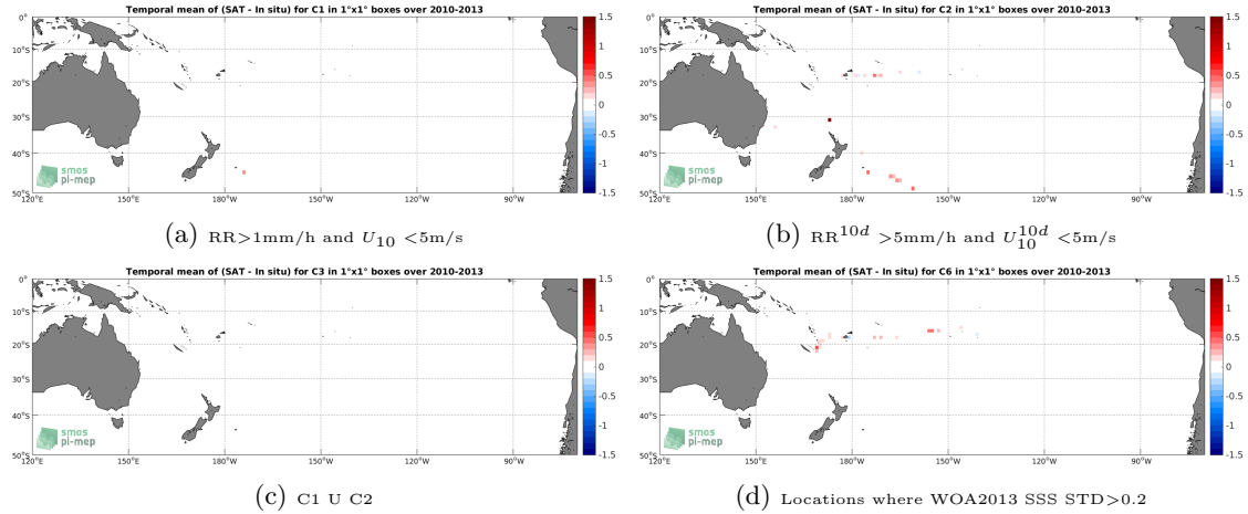
Figure 12: Temporal mean gridded over spatial boxes of size 1^\circ \times 1^\circ of \Delta SSS (SMOS-L3-CATDS-CECOS-LOCEAN-V3-18DAYS-25KM - TSG-GOSUD-Sailing-ship) for 4 different subdatasets corresponding to: RR > 1\text{mm/h} and U_{10} < 5\text{m/s} (a), RR^{10d} > 5\text{mm/h} and U_{10}^{10d} < 5\text{m/s} (b), C1 U C2 (c), Locations where WOA2013 SSS STD > 0.2 (d).
