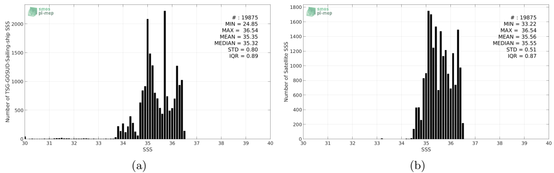
Figure 2: Histograms of SSS from TSG-GOSUD-Sailing-ship (a) and SMOS-L3-CATDS-CECOS-LOCEAN-V3-18DAYS-25KM (b) considering all match-up pairs per bins of 0.1 over the South Pacific Ocean Pi-MEP region and for the full satellite product period.
