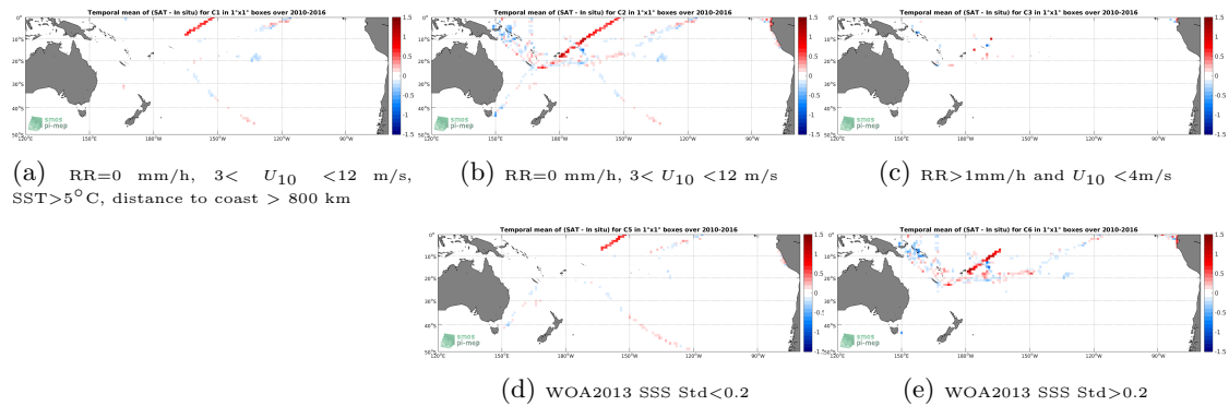
Figure 12: Temporal mean gridded over spatial boxes of size 1^\circ \times 1^\circ of \Delta SSS (SMOS-L3-CATDS-CECOS-LOCEAN-V3-18DAYS-25KM - TSG-GOSUD-Research-vessel) for 5 different subdatasets corresponding to:RR=0 mm/h, 3 < U_{10} < 12 m/s, SST >5^\circ C, distance to coast > 800 km (a), RR=0 mm/h, 3 < U_{10} < 12 m/s (b), RR >1 mm/h and U_{10} < 4 m/s (c), WOA2013 SSS Std <0.2 (d), WOA2013 SSS Std >0.2 (e).
