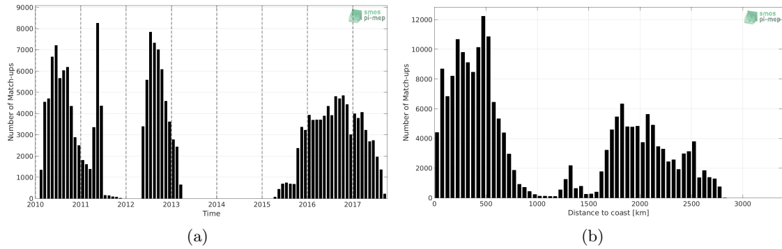
Figure 1: Number of match-ups between Surface drifters and SMOS-L3-CATDS-CECOS-LOCEAN-V3-18DAYS-25KM SSS as a function of time (a) and as function of the distance to coast (b) over the South Pacific Ocean Pi-MEP region and for the full satellite product period.
