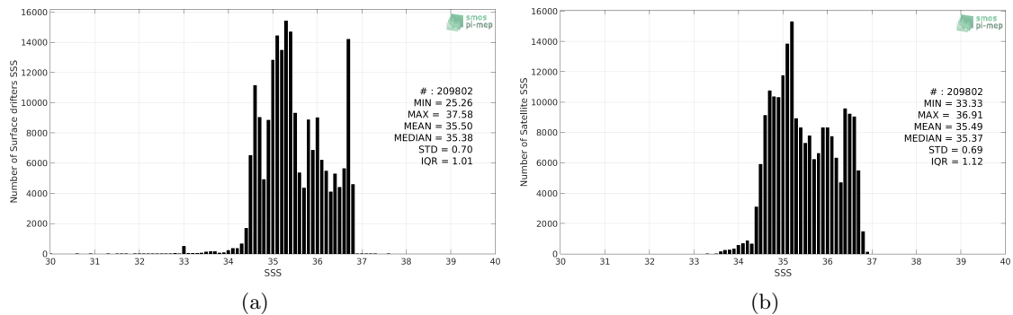
Figure 2: Histograms of SSS from Surface drifters (a) and SMOS-L3-CATDS-CECOS-LOCEAN-V3-18DAYS-25KM (b) considering all match-up pairs per bins of 0.1 over the South Pacific Ocean Pi-MEP region and for the full satellite product period.
