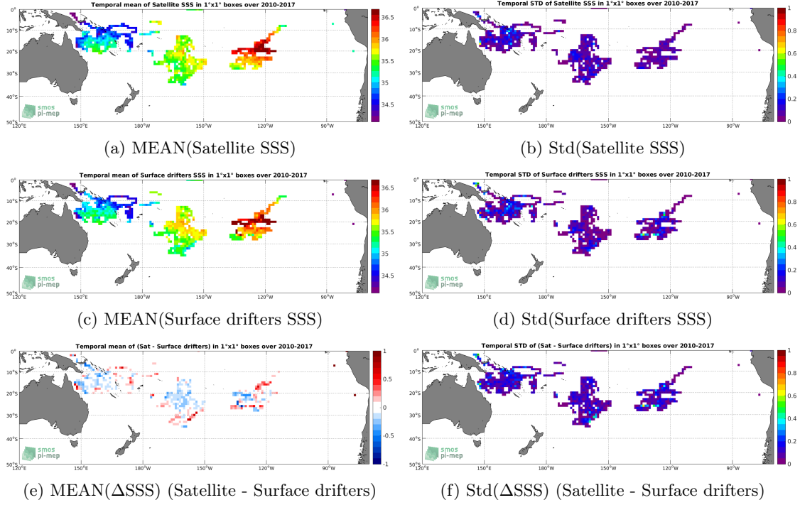
Figure 5: Temporal mean (left) and Std (right) of SSS from SMOS-L3-CATDS-CECOS-LOCEAN-V3-18DAYS-25KM (top), Surface drifters (middle), and of \Delta SSS (Satellite - Surface drifters). Only match-up pairs are used to generate these maps.
