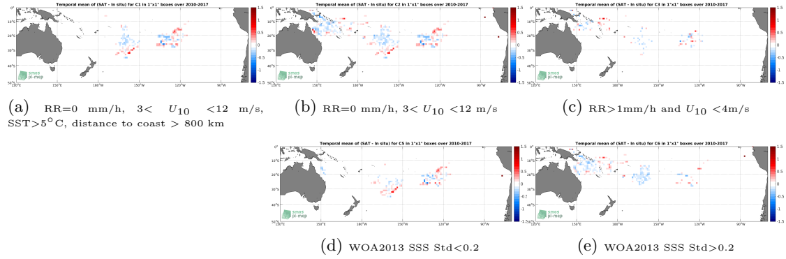
Figure 11: Temporal mean gridded over spatial boxes of size 1^\circ \times 1^\circ of \Delta SSS (SMOS-L3-CATDS-CECOS-LOCEAN-V3-18DAYS-25KM - Surface drifters) for 5 different subdatasets corresponding to: RR=0 mm/h, 3 < U_{10} < 12 m/s, SST > 5^\circ\text{C} , distance to coast > 800 km (a), RR=0 mm/h, 3 < U_{10} < 12 m/s (b), RR > 1 mm/h and U_{10} < 4 m/s (c), WOA2013 SSS Std < 0.2 (d), WOA2013 SSS Std > 0.2 (e).
