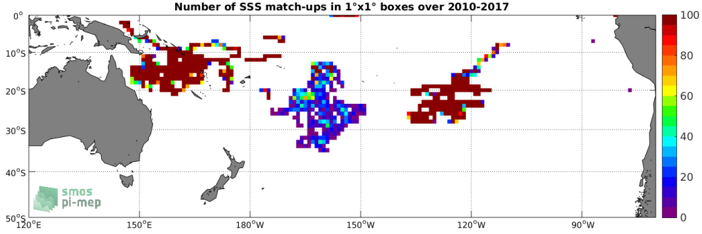
Figure 3: Number of SSS match-ups between Surface drifters SSS and the SMOS-L3-CATDS-CECOS-LOCEAN-V3-18DAYS-25KM SSS product for the South Pacific Ocean Pi-MEP region over 1^\circ \times 1^\circ boxes and for the full satellite product period.
