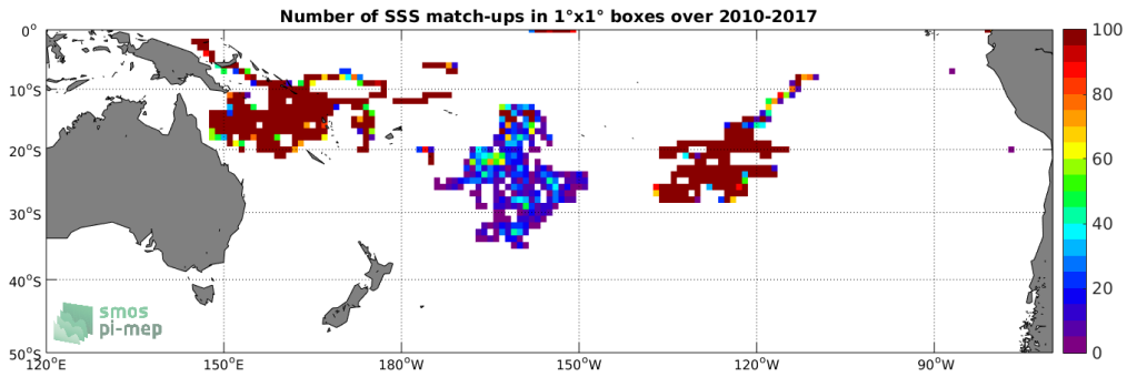
Figure 3: Number of SSS match-ups between Surface drifters SSS and the SMOS-L3-CATDS-CECOS-LOCEAN-V3-18DAYS-25KM SSS product for the South Pacific Ocean Pi-MEP region over 1°x1° boxes and for the full satellite product period.
