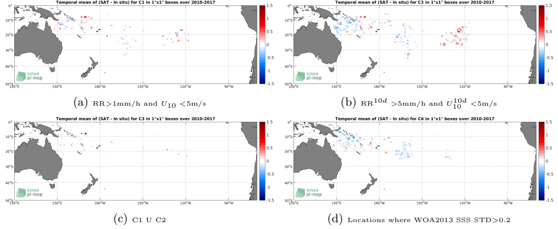
Figure 11: Temporal mean gridded over spatial boxes of size 1^\circ \times 1^\circ of \Delta SSS (SMOS-L3-CATDS-CECOS-LOCEAN-V3-18DAYS-25KM - Surface drifters) for 4 different subdatasets corresponding to: RR > 1\text{mm/h} and U_{10} < 5\text{m/s} (a), RR^{10d} > 5\text{mm/h} and U_{10}^{10d} < 5\text{m/s} (b), C1 U C2 (c), Locations where WOA2013 SSS STD > 0.2 (d).
