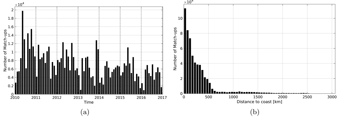
Figure 1: Number of match-ups between TSG-LEGOS-DM and SMOS-L3-CATDS-CECOS-LOCEAN-V2-9DAYS-25KM SSS as a function of time (a) and as function of the distance to coast (b) over the South Pacific Ocean Pi-MEP region and for the full satellite product period.
