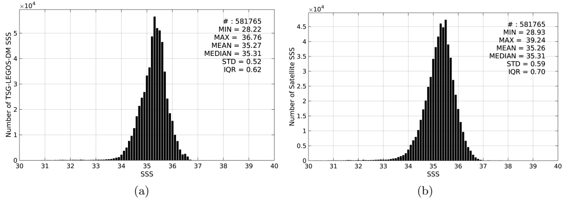
Figure 2: Histograms of SSS from TSG-LEGOS-DM (a) and SMOS-L3-CATDS-CECOS-LOCEAN-V2-9DAYS-25KM (b) considering all match-up pairs per bins of 0.1 over the South Pacific Ocean Pi-MEP region and for the full satellite product period.
