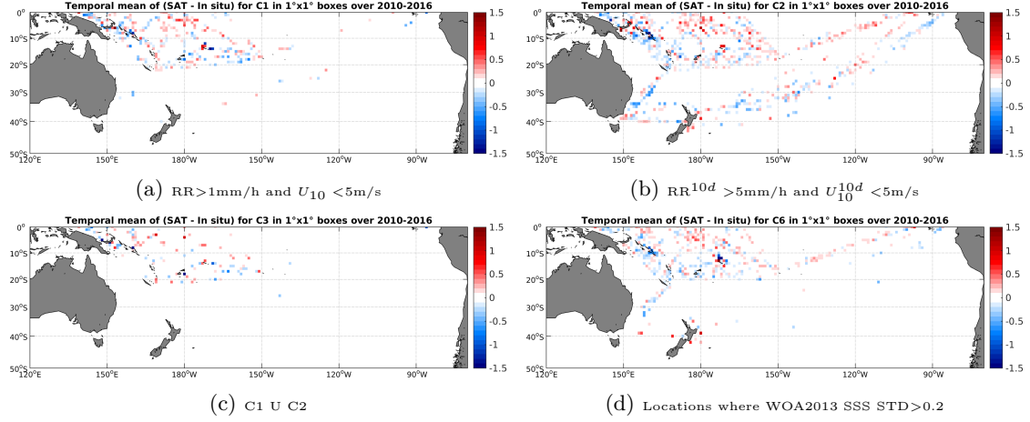
Figure 12: Temporal mean gridded over spatial boxes of size 1^\circ \times 1^\circ of \Delta SSS (SMOS-L3-CATDS-CECOS-LOCEAN-V2-9DAYS-25KM - TSG-LEGOS-DM) for 4 different subdatasets corresponding to: RR > 1mm/h and U_{10} < 5 m/s (a), RR^{10d} > 5 mm/h and U_{10}^{10d} < 5 m/s (b), C1 U C2 (c), Locations where WOA2013 SSS STD > 0.2 (d).
