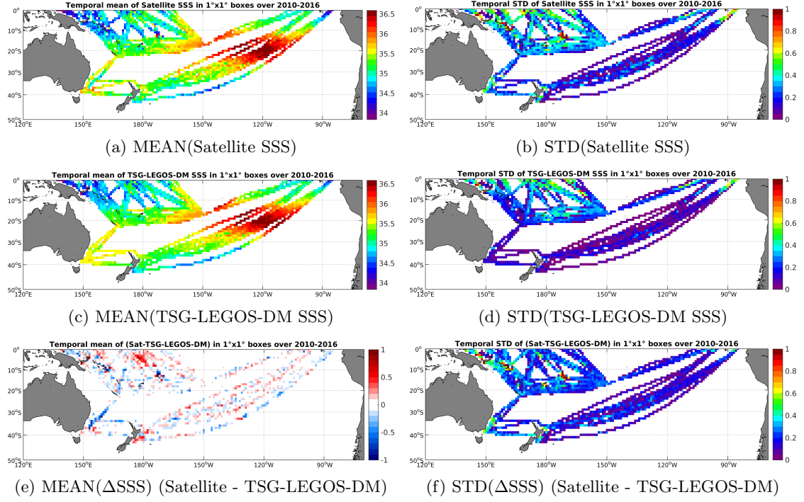
Figure 6: Temporal mean (left) and STD (right) of SSS from SMOS-L3-CATDS-CECOS-LOCEAN-V2-9DAYS-25KM (top), TSG-LEGOS-DM (middle), and of \Delta SSS (Satellite - TSG-LEGOS-DM). Only match-up pairs are used to generate these maps.
