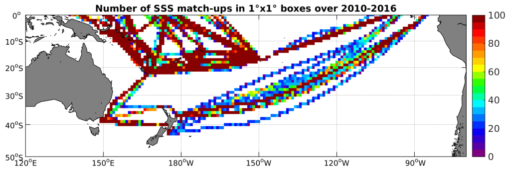
Figure 4: Number of SSS match-ups between TSG-LEGOS-DM SSS and the SMOS-L3-CATDS-CECOS-LOCEAN-V2-9DAYS-25KM SSS product for the South Pacific Ocean Pi-MEP region over 1^\circ \times 1^\circ boxes and for the full satellite product period.
