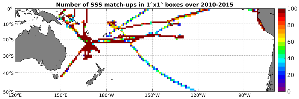
Figure 4: Number of SSS match-ups between TSG-GOSUD-Research-vessel SSS and the SMOS-L3-CATDS-CECOS-LOCEAN-V2-9DAYS-25KM SSS product for the South Pacific Ocean Pi-MEP region over 1^\circ \times 1^\circ boxes and for the full satellite product period.
