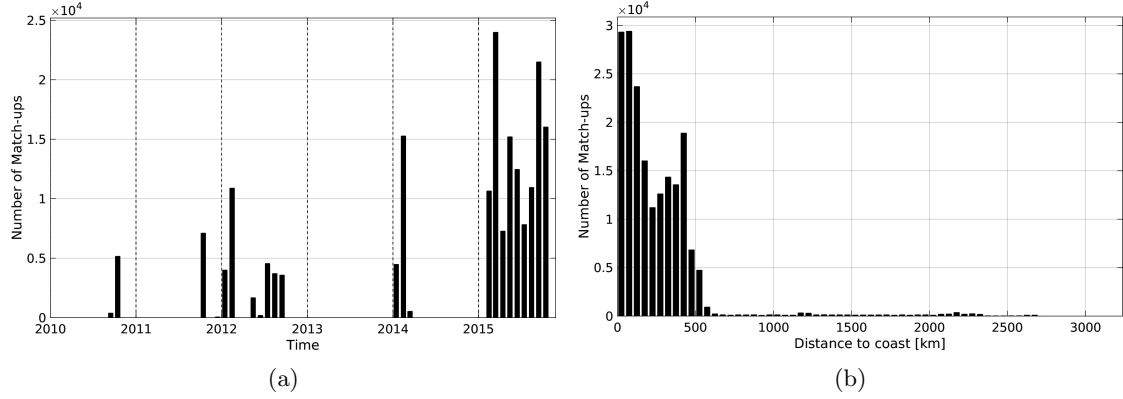
Figure 1: Number of match-ups between TSG-GOSUD-Research-vessel and SMOS-L3-CATDS-CECOS-LOCEAN-V2-9DAYS-25KM SSS as a function of time (a) and as function of the distance to coast (b) over the South Pacific Ocean Pi-MEP region and for the full satellite product period.
