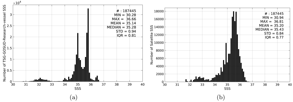
Figure 2: Histograms of SSS from TSG-GOSUD-Research-vessel (a) and SMOS-L3-CATDS-CECOS-LOCEAN-V2-9DAYS-25KM (b) considering all match-up pairs per bins of 0.1 over the South Pacific Ocean Pi-MEP region and for the full satellite product period.
