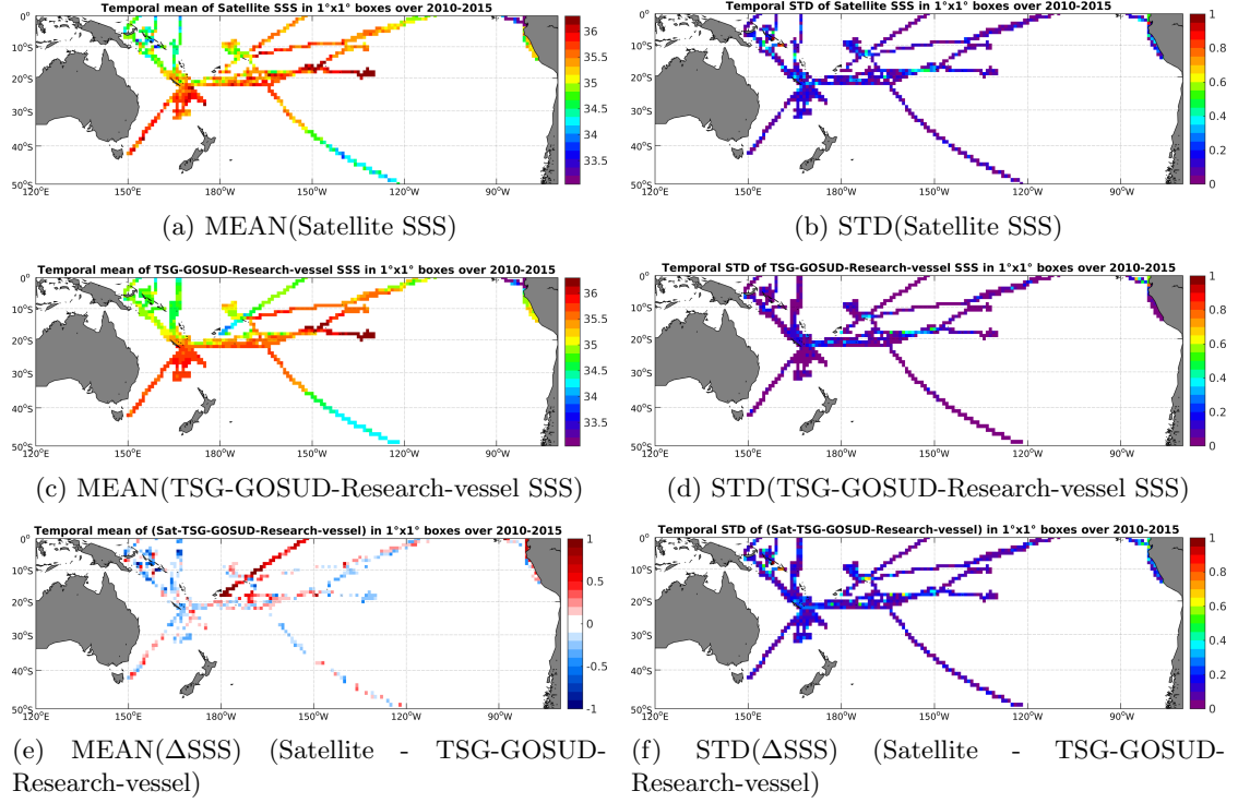
Figure 6: Temporal mean (left) and STD (right) of SSS from SMOS-L3-CATDS-CECOS-LOCEAN-V2-9DAYS-25KM (top), TSG-GOSUD-Research-vessel (middle), and of \Delta SSS (Satellite - TSG-GOSUD-Research-vessel). Only match-up pairs are used to generate these maps.
