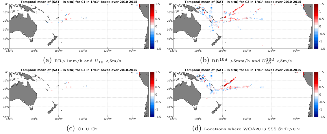
Figure 12: Temporal mean gridded over spatial boxes of size 1^\circ \times 1^\circ of \Delta SSS (SMOS-L3-CATDS-CECOS-LOCEAN-V2-9DAYS-25KM - TSG-GOSUD-Research-vessel) for 4 different subdatasets corresponding to: RR > 1 mm/h and U_{10} < 5 m/s (a), RR 10d > 5 mm/h and U_{10}^{10d} < 5 m/s (b), C1 U C2 (c), Locations where WOA2013 SSS STD > 0.2 (d).
