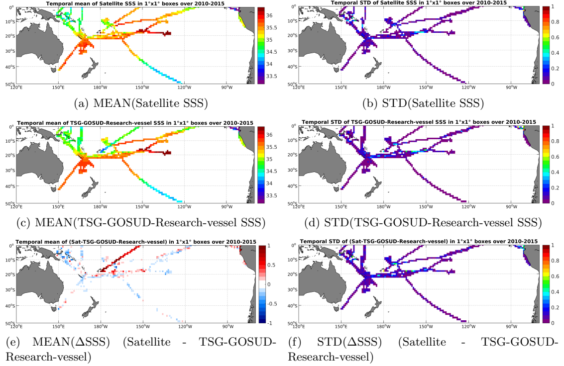
Figure 6: Temporal mean (left) and STD (right) of SSS from SMOS-L3-CATDS-CECOS-LOCEAN-V2-18DAYS-25KM (top), TSG-GOSUD-Research-vessel (middle), and of \Delta SSS (Satellite - TSG-GOSUD-Research-vessel). Only match-up pairs are used to generate these maps.
