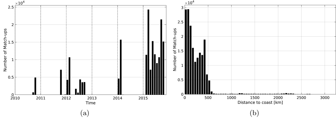
Figure 1: Number of match-ups between TSG-GOSUD-Research-vessel and SMOS-L3-CATDS-CECOS-LOCEAN-V2-18DAYS-25KM SSS as a function of time (a) and as function of the distance to coast (b) over the South Pacific Ocean Pi-MEP region and for the full satellite product period.
