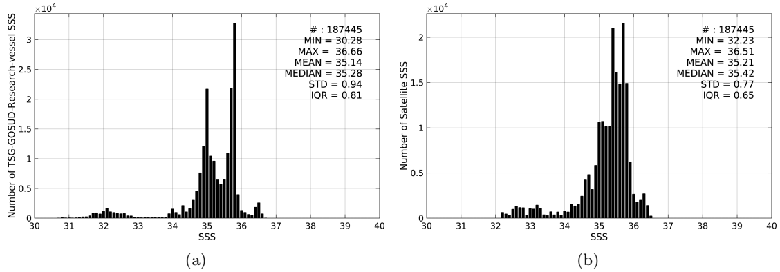
Figure 2: Histograms of SSS from TSG-GOSUD-Research-vessel (a) and SMOS-L3-CATDS-CECOS-LOCEAN-V2-18DAYS-25KM (b) considering all match-up pairs per bins of 0.1 over the South Pacific Ocean Pi-MEP region and for the full satellite product period.
