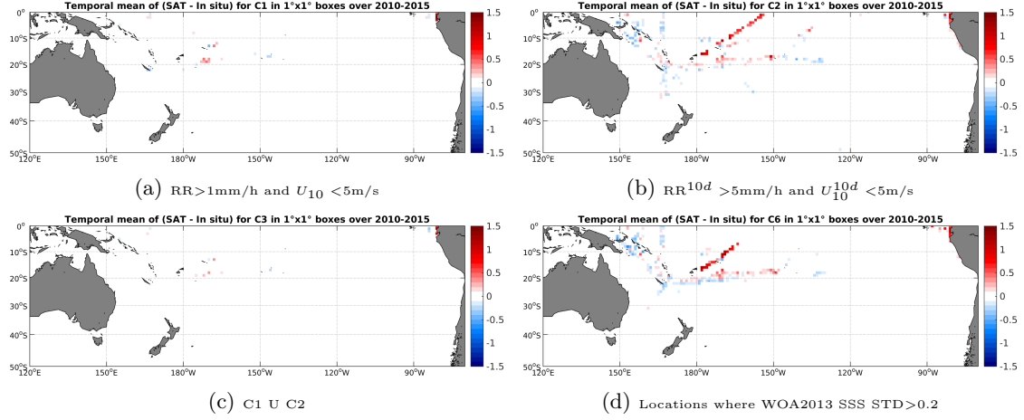
Figure 12: Temporal mean gridded over spatial boxes of size 1^\circ \times 1^\circ of \Delta SSS (SMOS-L3-CATDS-CECOS-LOCEAN-V2-18DAYS-25KM - TSG-GOSUD-Research-vessel) for 4 different subdatasets corresponding to: RR > 1mm/h and U_{10} < 5 m/s (a), RR 10d > 5mm/h and U_{10}^{10d} < 5 m/s (b), C1 U C2 (c), Locations where WOA2013 SSS STD > 0.2 (d).
