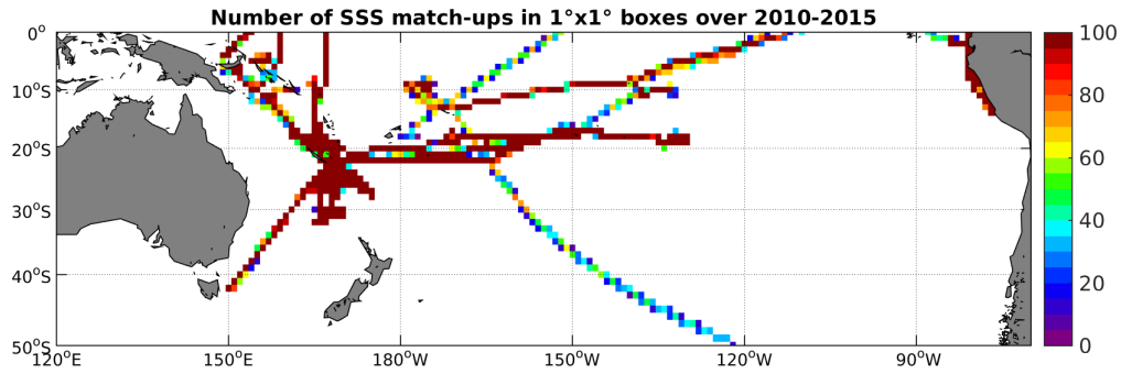
Figure 4: Number of SSS match-ups between TSG-GOSUD-Research-vessel SSS and the SMOS-L3-CATDS-CECOS-LOCEAN-V2-18DAYS-25KM SSS product for the South Pacific Ocean Pi-MEP region over 1^\circ \times 1^\circ boxes and for the full satellite product period.
