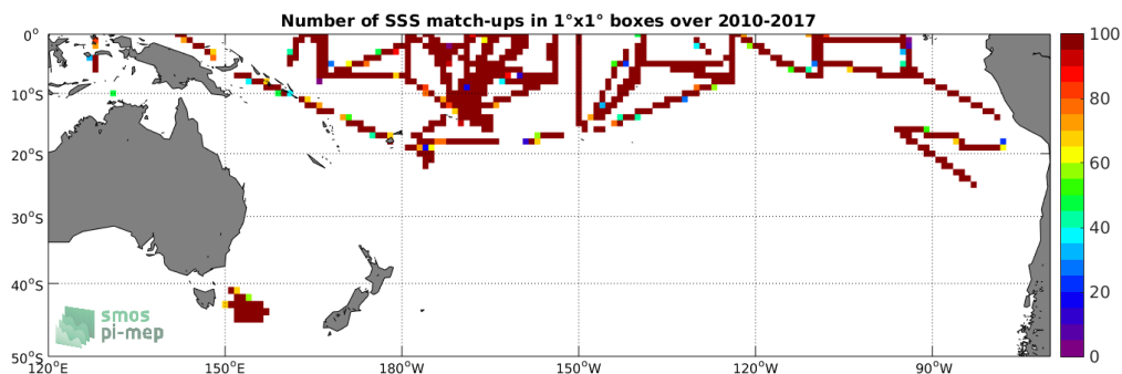
Figure 4: Number of SSS match-ups between TSG-SAMOS SSS and the SMOS L3 v2 - Monthly - 0.25 Deg (CATDS-CECOS-IFREMER) SSS product for the South Pacific Ocean Pi-MEP region over 1^\circ \times 1^\circ boxes and for the full satellite product period.
