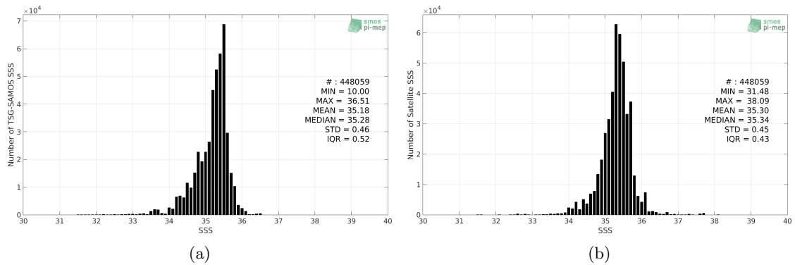
Figure 2: Histograms of SSS from TSG-SAMOS (a) and SMOS L3 v2 - Monthly - 0.25 Deg (CATDS-CECOS-IFREMER) (b) considering all match-up pairs per bins of 0.1 over the South Pacific Ocean Pi-MEP region and for the full satellite product period.
