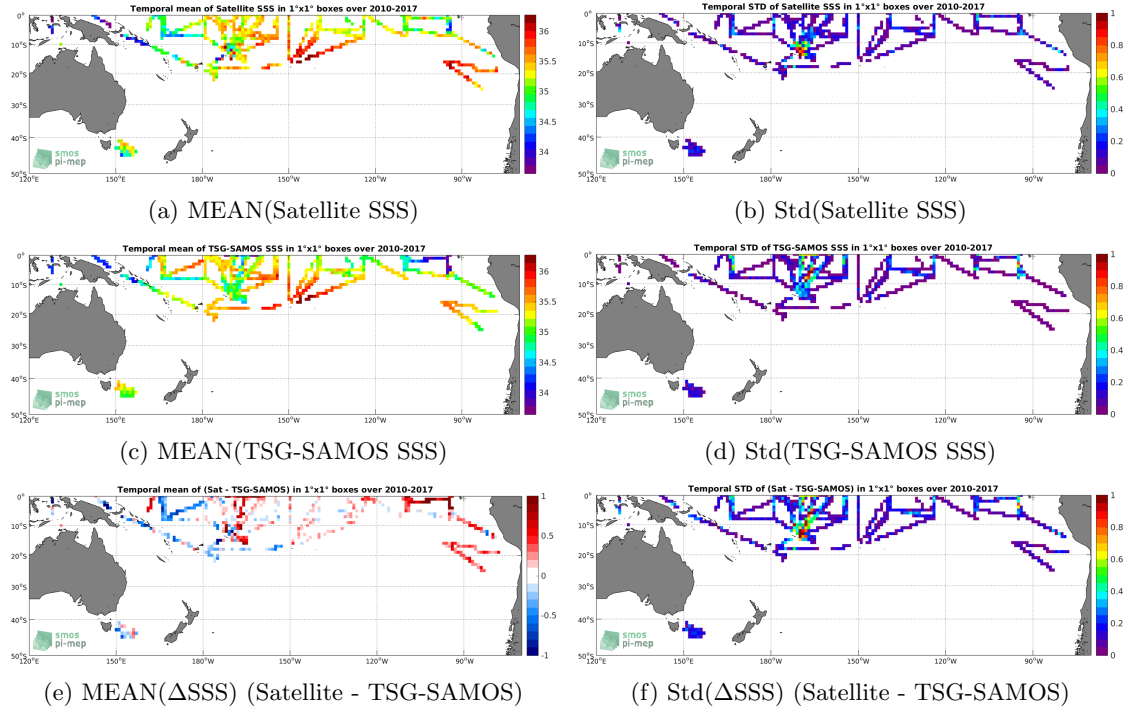
Figure 6: Temporal mean (left) and Std (right) of SSS from SMOS L3 v2 - Monthly - 0.25 Deg (CATDS-CECOS-IFREMER) (top), TSG-SAMOS (middle), and of \Delta SSS (Satellite - TSG-SAMOS). Only match-up pairs are used to generate these maps.
