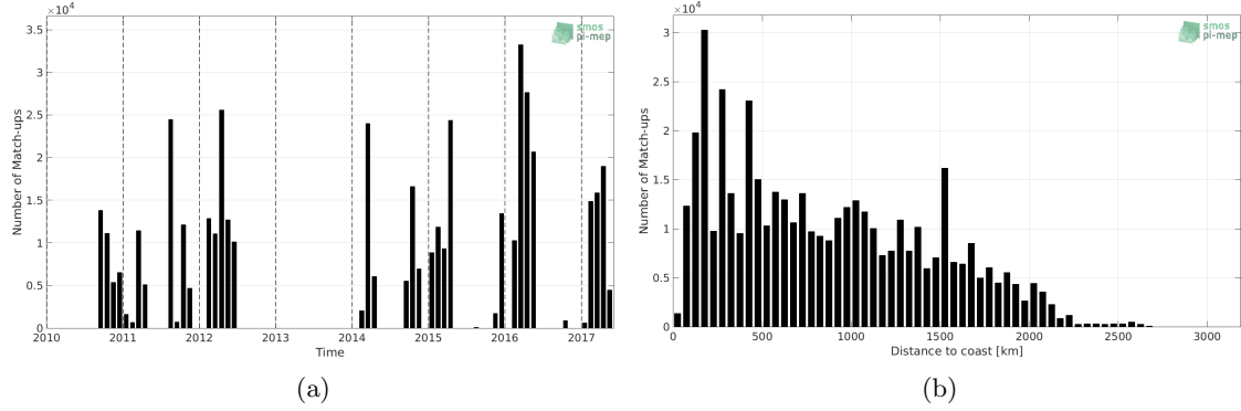
Figure 1: Number of match-ups between TSG-SAMOS and SMOS L3 v2 - Monthly - 0.25 Deg (CATDS-CECOS-IFREMER) SSS as a function of time (a) and as function of the distance to coast (b) over the South Pacific Ocean Pi-MEP region and for the full satellite product period.
