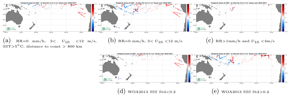
Figure 12: Temporal mean gridded over spatial boxes of size 1^\circ \times 1^\circ of \Delta SSS (SMOS L3 v2 - Monthly - 0.25 Deg (CATDS-CECOS-IFREMER) - TSG-SAMOS) for 5 different subdatasets corresponding to:RR=0 mm/h, 3 < U_{10} < 12 m/s, SST >5^\circ\text{C} , distance to coast > 800 km (a), RR=0 mm/h, 3 < U_{10} < 12 m/s (b), RR >1 mm/h and U_{10} < 4 m/s (c), WOA2013 SSS Std <0.2 (d), WOA2013 SSS Std >0.2 (e).
