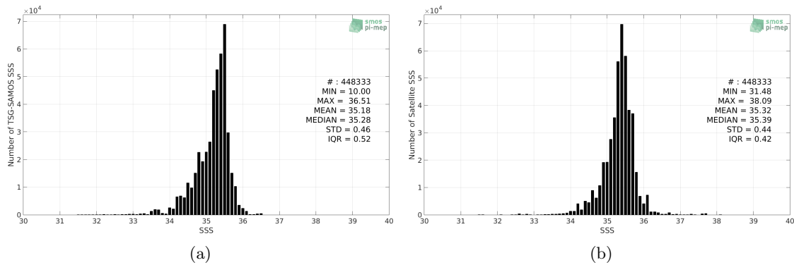
Figure 2: Histograms of SSS from TSG-SAMOS (a) and SMOS-L3-CATDS-IFREMER-CECOS-V2-MONTHLY-0.25DEG (b) considering all match-up pairs per bins of 0.1 over the South Pacific Ocean Pi-MEP region and for the full satellite product period.
