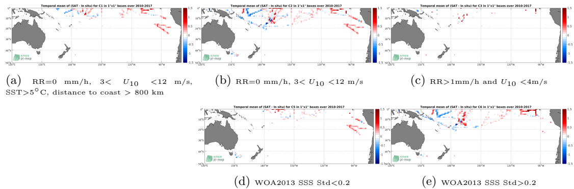
Figure 12: Temporal mean gridded over spatial boxes of size 1^\circ \times 1^\circ of \Delta SSS (SMOS-L3-CATDS-IFREMER-CECOS-V2-MONTHLY-0.25DEG - TSG-SAMOS) for 5 different subdatasets corresponding to:RR=0 mm/h, 3 < U_{10} < 12 m/s, SST >5^\circ C, distance to coast > 800 km (a), RR=0 mm/h, 3 < U_{10} < 12 m/s (b), RR >1 mm/h and U_{10} < 4 m/s (c), WOA2013 SSS Std <0.2 (d), WOA2013 SSS Std >0.2 (e).
