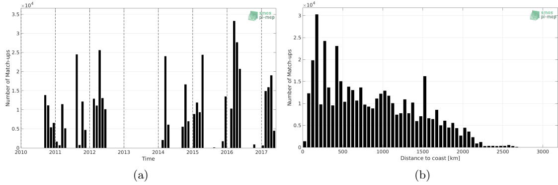
Figure 1: Number of match-ups between TSG-SAMOS and SMOS-L3-CATDS-IFREMER-CECOS-V2-MONTHLY-0.25DEG SSS as a function of time (a) and as function of the distance to coast (b) over the South Pacific Ocean Pi-MEP region and for the full satellite product period.
