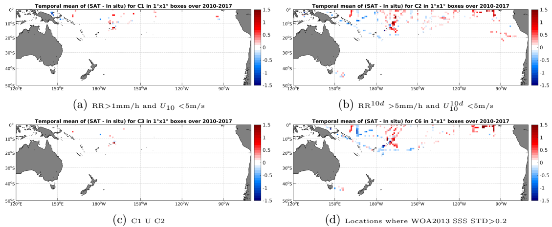
Figure 12: Temporal mean gridded over spatial boxes of size 1^\circ \times 1^\circ of \Delta SSS (SMOS-L3-CATDS-IFREMER-CECOS-V2-MONTHLY-0.25DEG - TSG-SAMOS) for 4 different subdatasets corresponding to:RR >1 mm/h and U_{10} < 5 m/s (a), RR 10d > 5 mm/h and U_{10}^{10d} < 5 m/s (b), C1 U C2 (c),Locations where WOA2013 SSS STD >0.2 (d).
