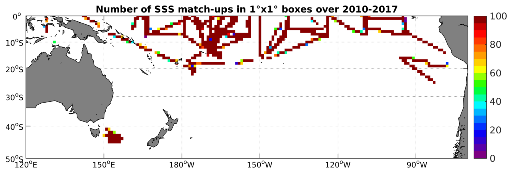
Figure 4: Number of SSS match-ups between TSG-SAMOS SSS and the SMOS-L3-CATDS-IFREMER-CECOS-V2-MONTHLY-0.25DEG SSS product for the South Pacific Ocean Pi-MEP region over 1^\circ \times 1^\circ boxes and for the full satellite product period.
