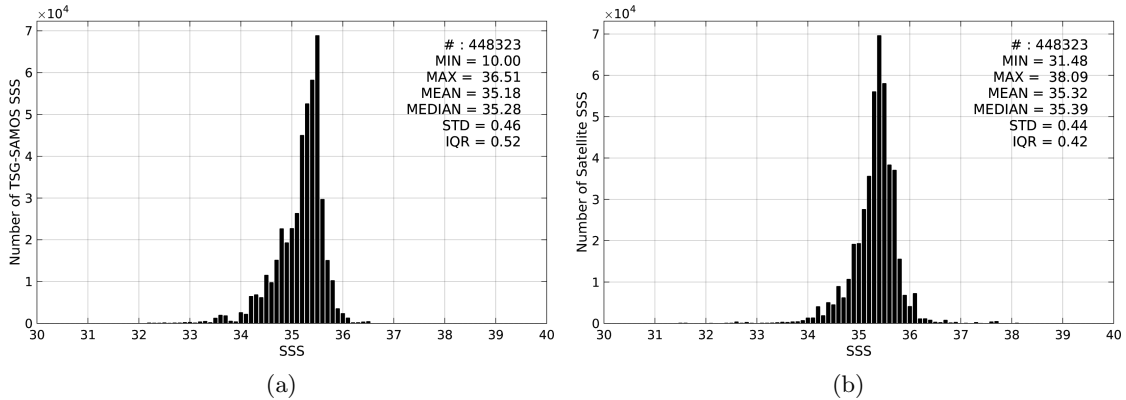
Figure 2: Histograms of SSS from TSG-SAMOS (a) and SMOS-L3-CATDS-IFREMER-CECOS-V2-MONTHLY-0.25DEG (b) considering all match-up pairs per bins of 0.1 over the South Pacific Ocean Pi-MEP region and for the full satellite product period.
