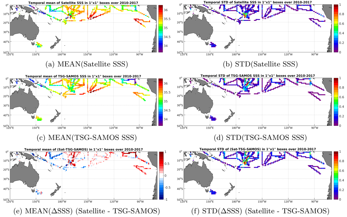
Figure 6: Temporal mean (left) and STD (right) of SSS from SMOS-L3-CATDS-IFREMER-CECOS-V2-MONTHLY-0.25DEG (top), TSG-SAMOS (middle), and of \Delta SSS (Satellite - TSG-SAMOS). Only match-up pairs are used to generate these maps.
