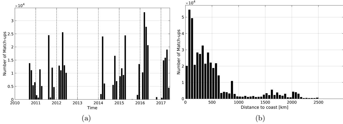
Figure 1: Number of match-ups between TSG-SAMOS and SMOS-L3-CATDS-IFREMER-CECOS-V2-MONTHLY-0.25DEG SSS as a function of time (a) and as function of the distance to coast (b) over the South Pacific Ocean Pi-MEP region and for the full satellite product period.
