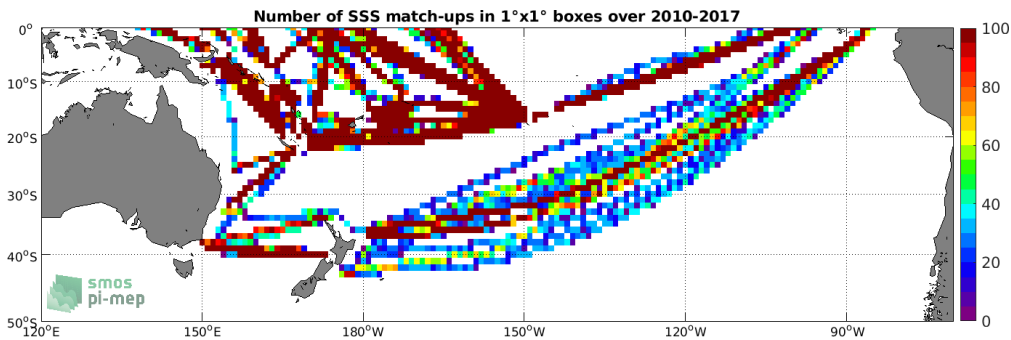
Figure 4: Number of SSS match-ups between TSG (LEGOS-DM) SSS and the SMOS SSS L3 v2 - Monthly - 0.25 Deg (CATDS-CECOS-IFREMER) SSS product for the South Pacific Ocean Pi-MEP region over 1^\circ \times 1^\circ boxes and for the full satellite product period.
