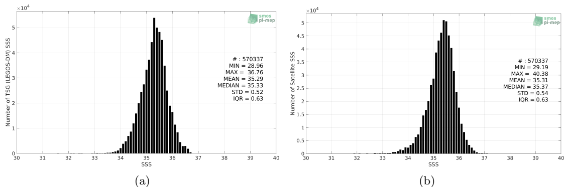
Figure 2: Histograms of SSS from TSG (LEGOS-DM) (a) and SMOS SSS L3 v2 - Monthly - 0.25 Deg (CATDS-CECOS-IFREMER) (b) considering all match-up pairs per bins of 0.1 over the South Pacific Ocean Pi-MEP region and for the full satellite product period.
