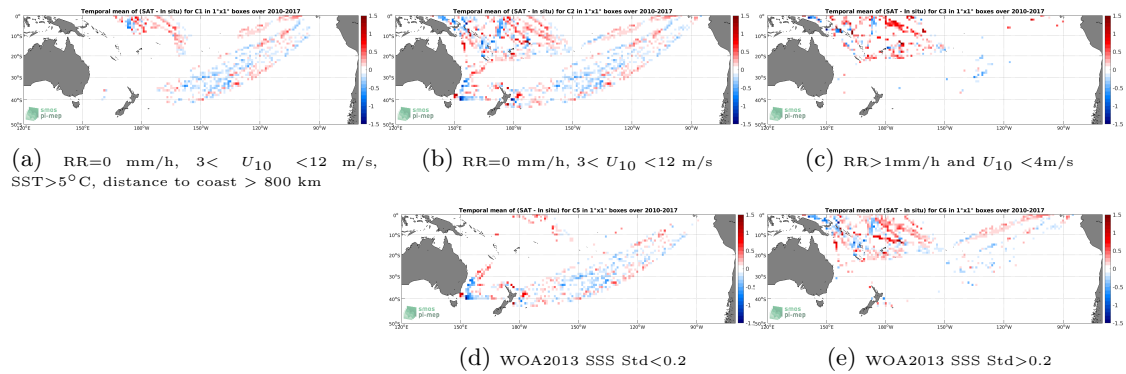
Figure 12: Temporal mean gridded over spatial boxes of size 1^\circ \times 1^\circ of \Delta SSS (SMOS SSS L3 v2 - Monthly - 0.25 Deg (CATDS-CECOS-IFREMER) - TSG (LEGOS-DM)) for 5 different subdatasets corresponding to:RR=0 mm/h, 3 < U_{10} < 12 m/s, SST >5^\circ C, distance to coast > 800 km (a), RR=0 mm/h, 3 < U_{10} < 12 m/s (b), RR >1 mm/h and U_{10} < 4 m/s (c), WOA2013 SSS Std <0.2 (d), WOA2013 SSS Std >0.2 (e).
