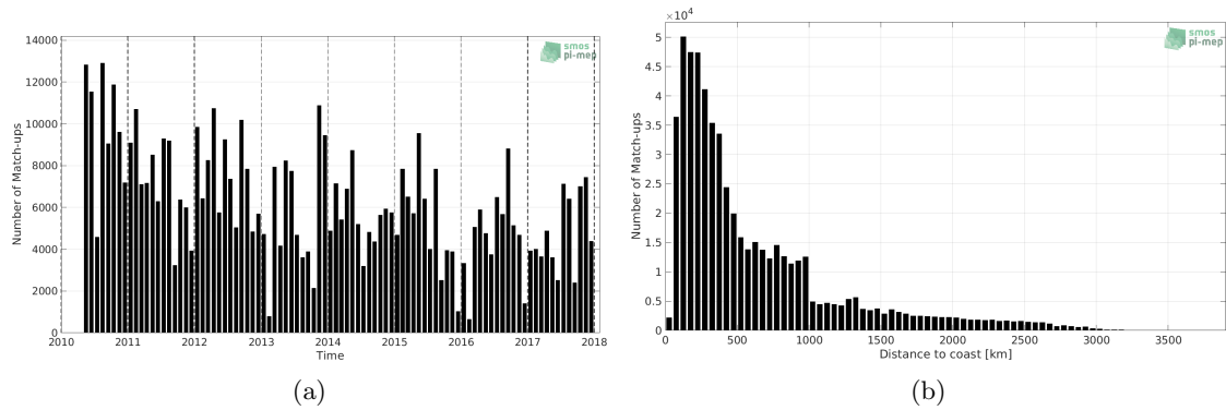
Figure 1: Number of match-ups between TSG (LEGOS-DM) and SMOS SSS L3 v2 - Monthly - 0.25 Deg (CATDS-CECOS-IFREMER) SSS as a function of time (a) and as function of the distance to coast (b) over the South Pacific Ocean Pi-MEP region and for the full satellite product period.
