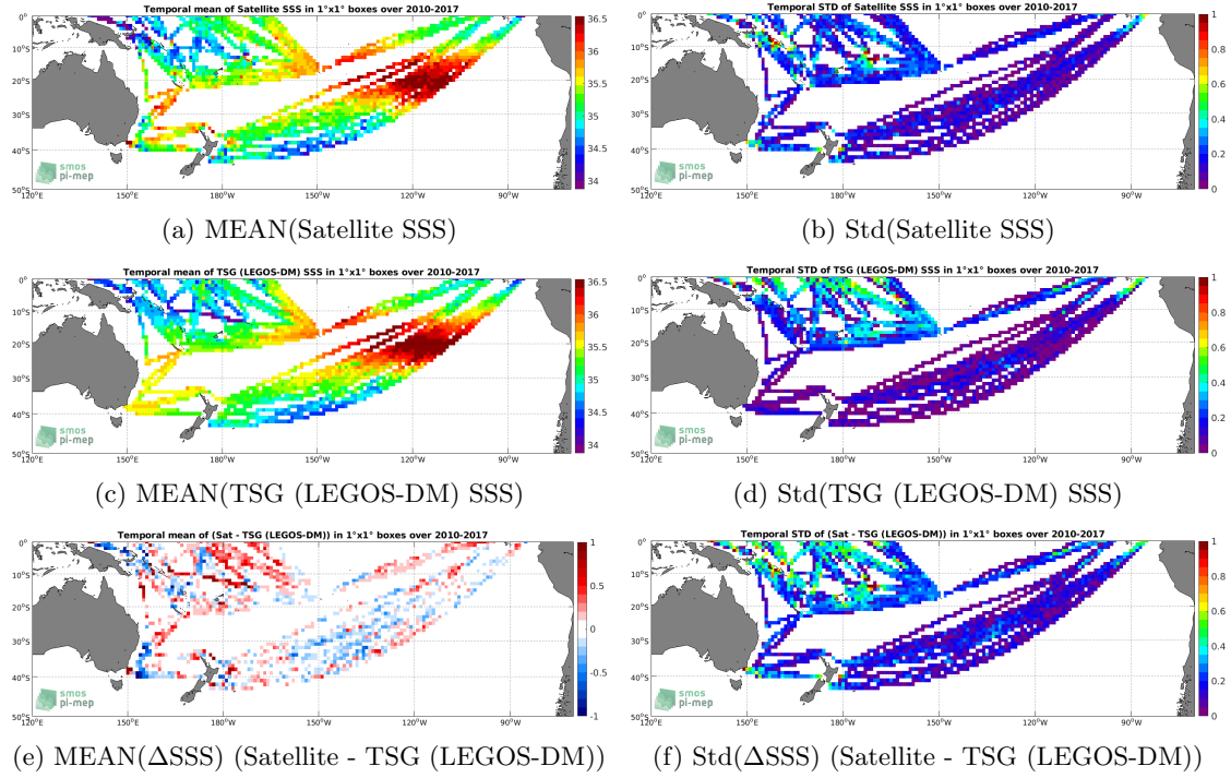
Figure 6: Temporal mean (left) and Std (right) of SSS from SMOS SSS L3 v2 - Monthly - 0.25 Deg (CATDS-CECOS-IFREMER) (top), TSG (LEGOS-DM) (middle), and of \Delta SSS (Satellite - TSG (LEGOS-DM)). Only match-up pairs are used to generate these maps.
