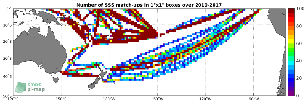
Figure 4: Number of SSS match-ups between TSG-LEGOS-DM SSS and the SMOS-L3-CATDS-IFREMER-CECOS-V2-MONTHLY-0.25DEG SSS product for the South Pacific Ocean Pi-MEP region over 1°x1° boxes and for the full satellite product period.
