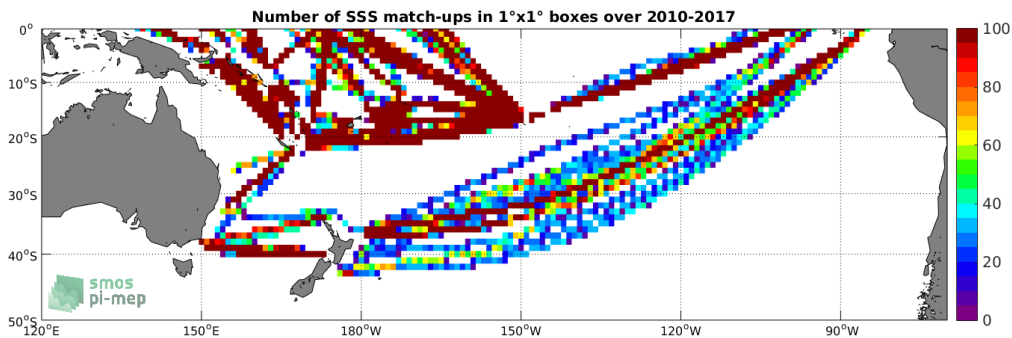
Figure 4: Number of SSS match-ups between TSG-LEGOS-DM SSS and the SMOS-L3-CATDS-IFREMER-CECOS-V2-MONTHLY-0.25DEG SSS product for the South Pacific Ocean Pi-MEP region over 1^\circ \times 1^\circ boxes and for the full satellite product period.
