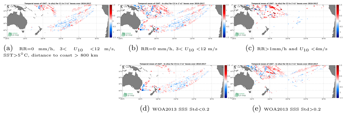
Figure 12: Temporal mean gridded over spatial boxes of size 1^\circ \times 1^\circ of \Delta SSS (SMOS-L3-CATDS-IFREMER-CECOS-V2-MONTHLY-0.25DEG - TSG-LEGOS-DM) for 5 different subdatasets corresponding to:RR=0 mm/h, 3 < U_{10} < 12 m/s, SST >5^\circ C, distance to coast > 800 km (a), RR=0 mm/h, 3 < U_{10} < 12 m/s (b), RR >1 mm/h and U_{10} < 4 m/s (c), WOA2013 SSS Std <0.2 (d), WOA2013 SSS Std >0.2 (e).
