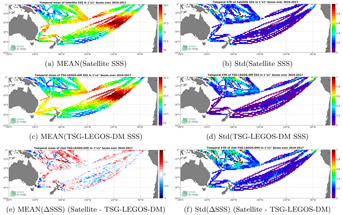
Figure 6: Temporal mean (left) and Std (right) of SSS from SMOS-L3-CATDS-IFREMER-CECOS-V2-MONTHLY-0.25DEG (top), TSG-LEGOS-DM (middle), and of \Delta SSS (Satellite - TSG-LEGOS-DM). Only match-up pairs are used to generate these maps.
