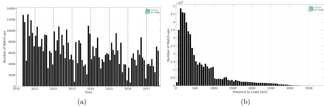
Figure 1: Number of match-ups between TSG-LEGOS-DM and SMOS-L3-CATDS-IFREMER-CECOS-V2-MONTHLY-0.25DEG SSS as a function of time (a) and as function of the distance to coast (b) over the South Pacific Ocean Pi-MEP region and for the full satellite product period.
