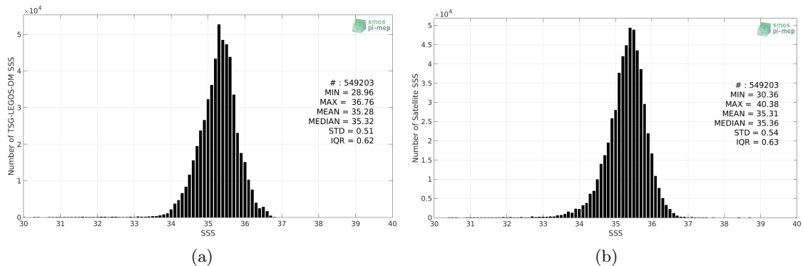
Figure 2: Histograms of SSS from TSG-LEGOS-DM (a) and SMOS-L3-CATDS-IFREMER-CECOS-V2-MONTHLY-0.25DEG (b) considering all match-up pairs per bins of 0.1 over the South Pacific Ocean Pi-MEP region and for the full satellite product period.
