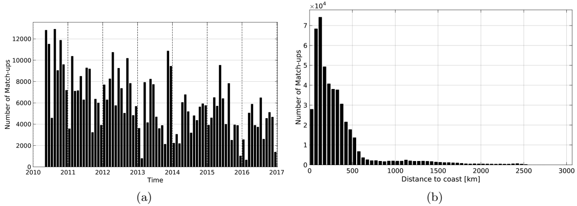
Figure 1: Number of match-ups between TSG-LEGOS-DM and SMOS-L3-CATDS-IFREMER-CECOS-V2-MONTHLY-0.25DEG SSS as a function of time (a) and as function of the distance to coast (b) over the South Pacific Ocean Pi-MEP region and for the full satellite product period.
