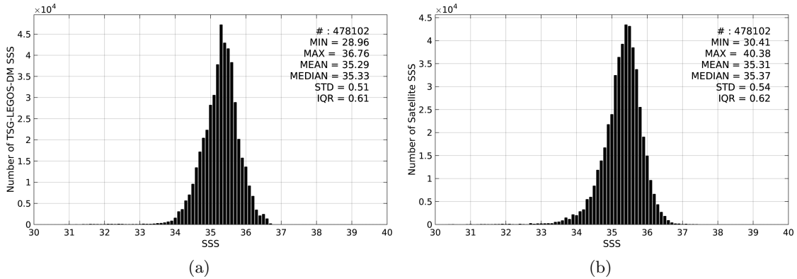
Figure 2: Histograms of SSS from TSG-LEGOS-DM (a) and SMOS-L3-CATDS-IFREMER-CECOS-V2-MONTHLY-0.25DEG (b) considering all match-up pairs per bins of 0.1 over the South Pacific Ocean Pi-MEP region and for the full satellite product period.
