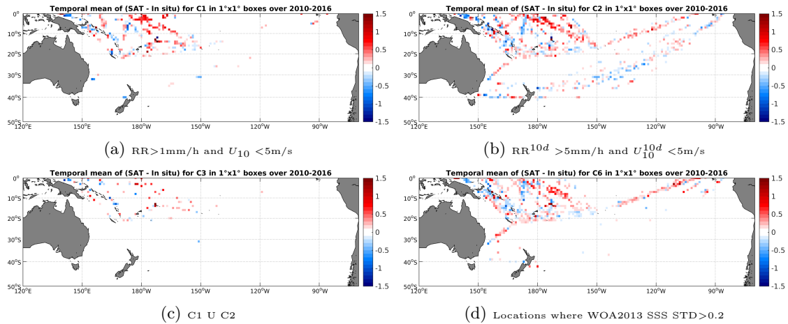
Figure 12: Temporal mean gridded over spatial boxes of size 1^\circ \times 1^\circ of \Delta SSS (SMOS-L3-CATDS-IFREMER-CECOS-V2-MONTHLY-0.25DEG - TSG-LEGOS-DM) for 4 different subdatasets corresponding to: RR > 1 mm/h and U_{10} < 5 m/s (a), RR 10d > 5 mm/h and U_{10d} < 5 m/s (b), C1 U C2 (c), Locations where WOA2013 SSS STD > 0.2 (d).
