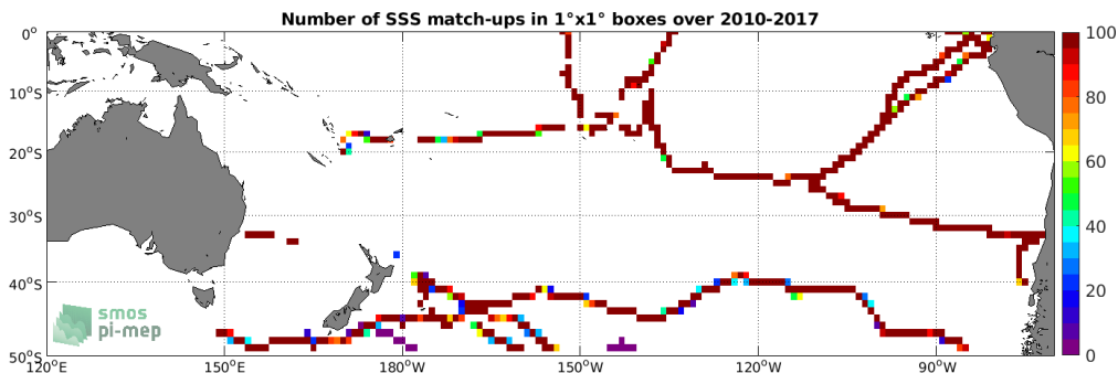
Figure 4: Number of SSS match-ups between TSG (GOSUD-Sailing-ship) SSS and the SMOS SSS L3 v2 - Monthly - 0.25 Deg (CATDS-CECOS-IFREMER) SSS product for the South Pacific Ocean Pi-MEP region over 1^\circ \times 1^\circ boxes and for the full satellite product period.
