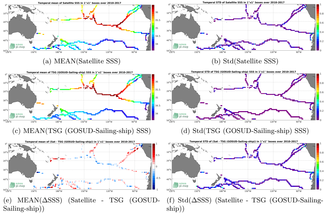
Figure 6: Temporal mean (left) and Std (right) of SSS from SMOS SSS L3 v2 - Monthly - 0.25 Deg (CATDS-CECOS-IFREMER) (top), TSG (GOSUD-Sailing-ship) (middle), and of \Delta SSS (Satellite - TSG (GOSUD-Sailing-ship)). Only match-up pairs are used to generate these maps.
