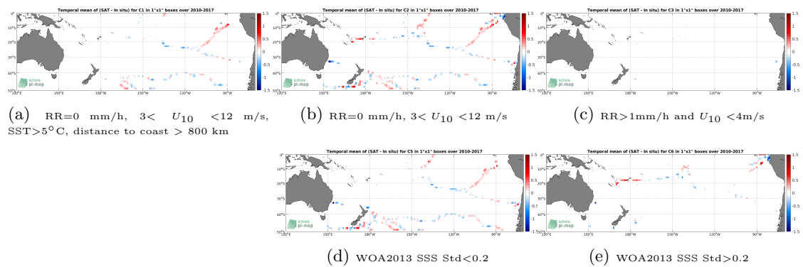
Figure 12: Temporal mean gridded over spatial boxes of size 1^\circ \times 1^\circ of \Delta SSS (SMOS SSS L3 v2 - Monthly - 0.25 Deg (CATDS-CECOS-IFREMER) - TSG (GOSUD-Sailing-ship)) for 5 different subdatasets corresponding to: RR=0 mm/h, 3 < U_{10} < 12 m/s, SST > 5°C, distance to coast > 800 km (a), RR=0 mm/h, 3 < U_{10} < 12 m/s (b), RR > 1mm/h and U_{10} < 4 m/s (c), WOA2013 SSS Std < 0.2 (d), WOA2013 SSS Std > 0.2 (e).
