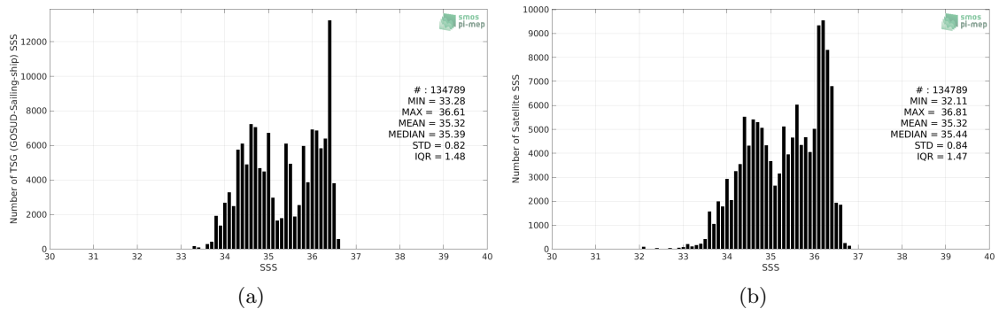
Figure 2: Histograms of SSS from TSG (GOSUD-Sailing-ship) (a) and SMOS SSS L3 v2 - Monthly - 0.25 Deg (CATDS-CECOS-IFREMER) (b) considering all match-up pairs per bins of 0.1 over the South Pacific Ocean Pi-MEP region and for the full satellite product period.
