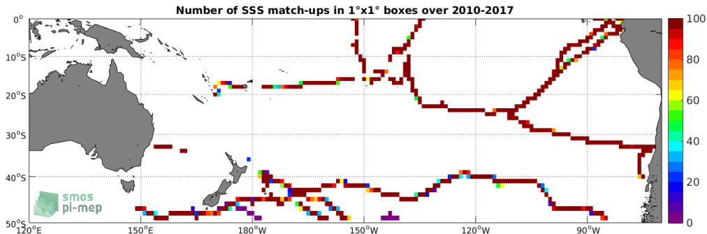
Figure 4: Number of SSS match-ups between TSG-GOSUD-Sailing-ship SSS and the SMOS L3 v2 - Monthly - 0.25 Deg (CATDS-CECOS-IFREMER) SSS product for the South Pacific Ocean Pi-MEP region over 1°x1° boxes and for the full satellite product period.
