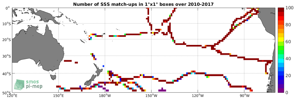
Figure 4: Number of SSS match-ups between TSG-GOSUD-Sailing-ship SSS and the SMOS-L3-CATDS-IFREMER-CECOS-V2-MONTHLY-0.25DEG SSS product for the South Pacific Ocean Pi-MEP region over 1°x1° boxes and for the full satellite product period.
