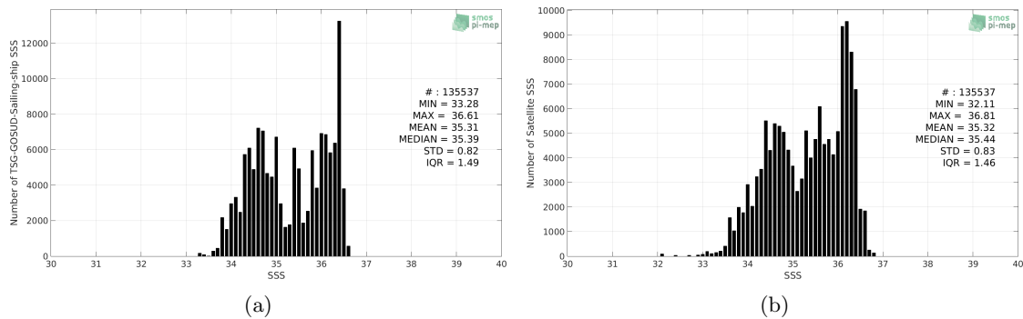
Figure 2: Histograms of SSS from TSG-GOSUD-Sailing-ship (a) and SMOS-L3-CATDS-IFREMER-CECOS-V2-MONTHLY-0.25DEG (b) considering all match-up pairs per bins of 0.1 over the South Pacific Ocean Pi-MEP region and for the full satellite product period.
