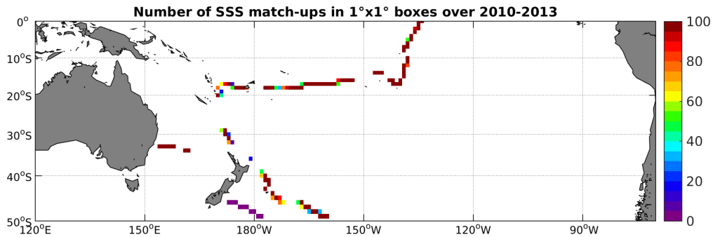
Figure 4: Number of SSS match-ups between TSG-GOSUD-Sailing-ship SSS and the SMOS-L3-CATDS-IFREMER-CECOS-V2-MONTHLY-0.25DEG SSS product for the South Pacific Ocean Pi-MEP region over 1^\circ \times 1^\circ boxes and for the full satellite product period.
