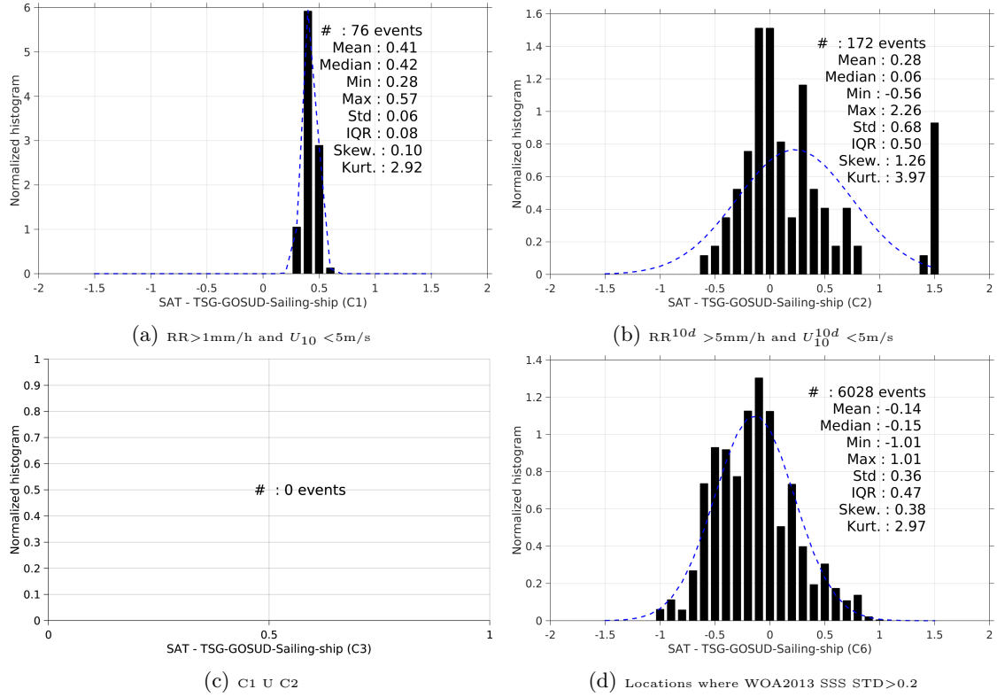
Figure 13: Normalized histogram of \Delta SSS (SMOS-L3-CATDS-IFREMER-CECOS-V2-MONTHLY-0.25DEG - TSG-GOSUD-Sailing-ship) for 6 different subdatasets corresponding to: RR > 1mm/h and U_{10} < 5 m/s (a), RR^{10d} > 5 mm/h and U_{10}^{10d} < 5 m/s (b), C1 U C2 (c), Locations where WOA2013 SSS STD > 0.2 (d).
