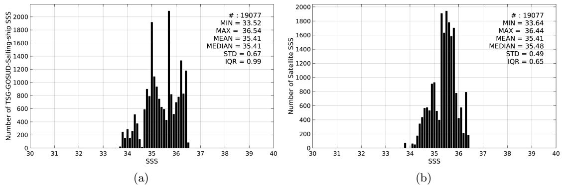
Figure 2: Histograms of SSS from TSG-GOSUD-Sailing-ship (a) and SMOS-L3-CATDS-IFREMER-CECOS-V2-MONTHLY-0.25DEG (b) considering all match-up pairs per bins of 0.1 over the South Pacific Ocean Pi-MEP region and for the full satellite product period.
