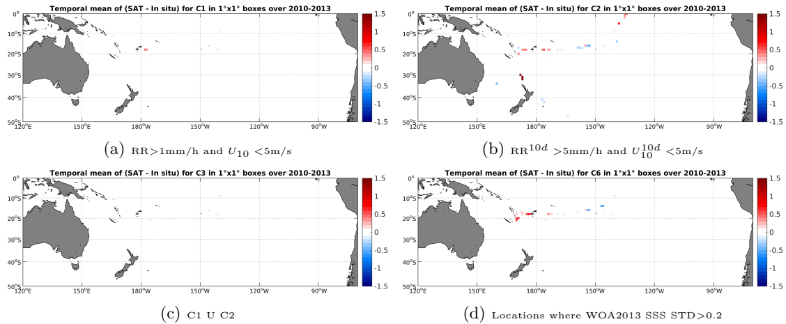
Figure 12: Temporal mean gridded over spatial boxes of size 1^\circ \times 1^\circ of \Delta SSS (SMOS-L3-CATDS-IFREMER-CECOS-V2-MONTHLY-0.25DEG - TSG-GOSUD-Sailing-ship) for 4 different sub-datasets corresponding to: RR > 1 mm/h and U_{10} < 5 m/s (a), RR 10d > 5 mm/h and U_{10}^{10d} < 5 m/s (b), C1 U C2 (c), Locations where WOA2013 SSS STD > 0.2 (d).
