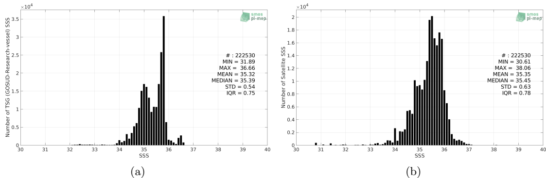
Figure 2: Histograms of SSS from TSG (GOSUD-Research-vessel) (a) and SMOS SSS L3 v2 - Monthly - 0.25 Deg (CATDS-CECOS-IFREMER) (b) considering all match-up pairs per bins of 0.1 over the South Pacific Ocean Pi-MEP region and for the full satellite product period.
