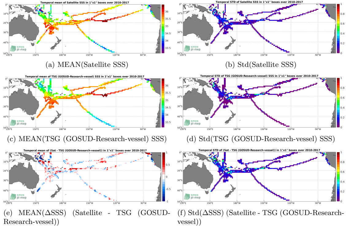
Figure 6: Temporal mean (left) and Std (right) of SSS from SMOS SSS L3 v2 - Monthly - 0.25 Deg (CATDS-CECOS-IFREMER) (top), TSG (GOSUD-Research-vessel) (middle), and of \Delta SSS (Satellite - TSG (GOSUD-Research-vessel)). Only match-up pairs are used to generate these maps.
