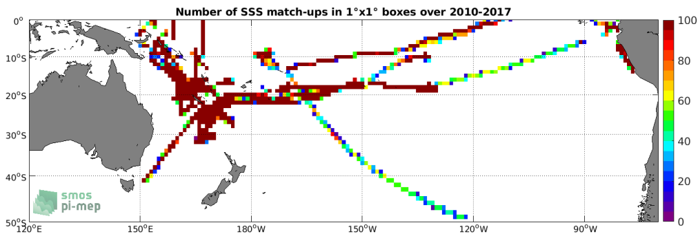
Figure 4: Number of SSS match-ups between TSG (GOSUD-Research-vessel) SSS and the SMOS SSS L3 v2 - Monthly - 0.25 Deg (CATDS-CECOS-IFREMER) SSS product for the South Pacific Ocean Pi-MEP region over 1°x1° boxes and for the full satellite product period.
