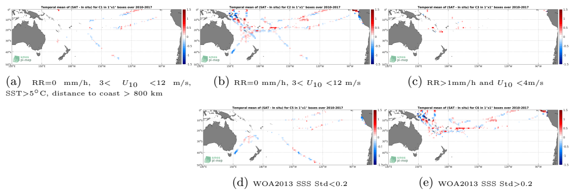
Figure 12: Temporal mean gridded over spatial boxes of size 1^\circ \times 1^\circ of \Delta SSS (SMOS SSS L3 v2 - Monthly - 0.25 Deg (CATDS-CECOS-IFREMER) - TSG (GOSUD-Research-vessel)) for 5 different subdatasets corresponding to:RR=0 mm/h, 3 < U_{10} < 12 m/s, SST>5°C, distance to coast > 800 km (a), RR=0 mm/h, 3 < U_{10} < 12 m/s (b), RR>1mm/h and U_{10} < 4 m/s (c), WOA2013 SSS Std<0.2 (d), WOA2013 SSS Std>0.2 (e).
