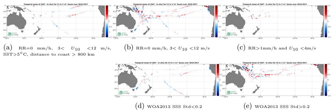
Figure 12: Temporal mean gridded over spatial boxes of size 1^\circ \times 1^\circ of \Delta\text{SSS} (SMOS SSS L3 v2 - Monthly - 0.25 Deg (CATDS-CECOS-IFREMER) - TSG (GOSUD-Research-vessel)) for 5 different subdatasets corresponding to:RR=0 mm/h, 3 < U_{10} < 12 m/s, SST>5°C, distance to coast > 800 km (a), RR=0 mm/h, 3 < U_{10} < 12 m/s (b), RR>1mm/h and U_{10} < 4 m/s (c), WOA2013 SSS Std<0.2 (d), WOA2013 SSS Std>0.2 (e).
