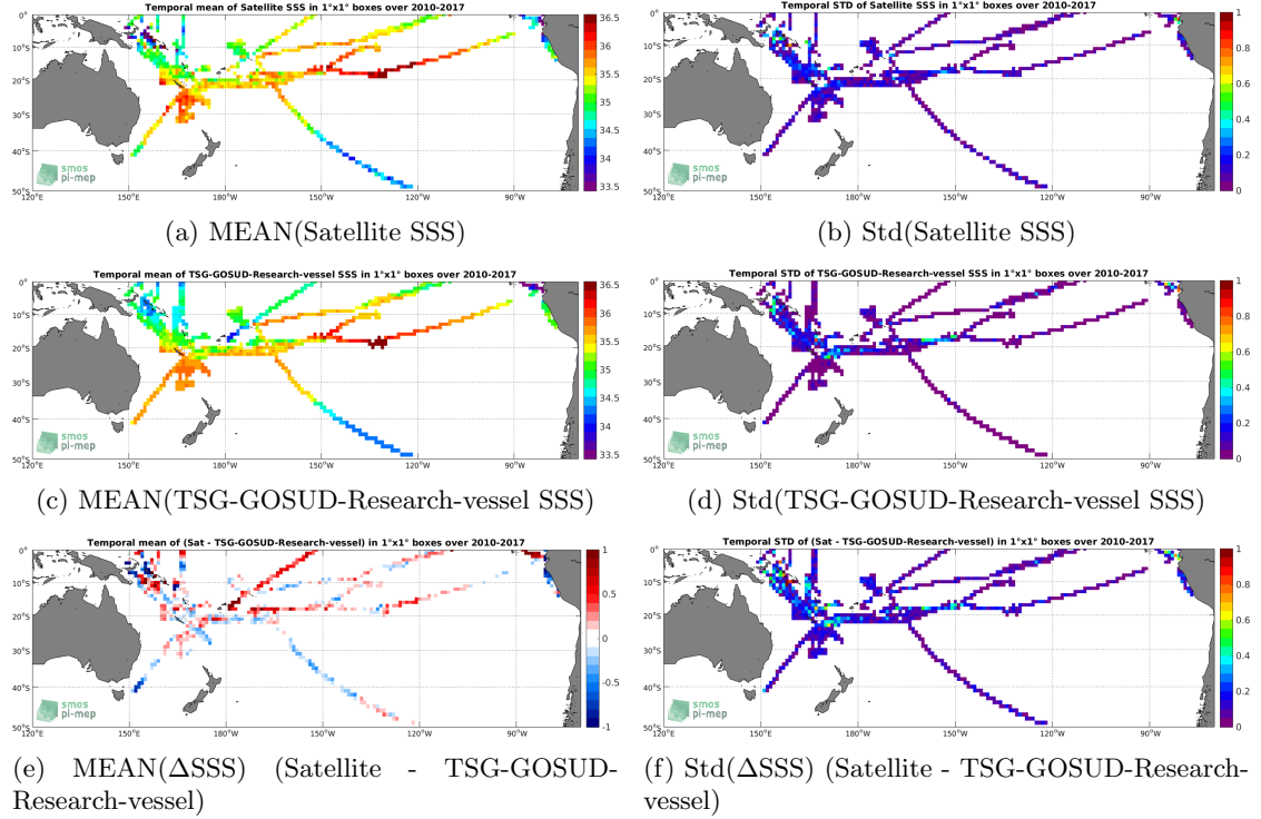
Figure 6: Temporal mean (left) and Std (right) of SSS from SMOS L3 v2 - Monthly - 0.25 Deg (CATDS-CECOS-IFREMER) (top), TSG-GOSUD-Research-vessel (middle), and of \Delta SSS (Satellite - TSG-GOSUD-Research-vessel). Only match-up pairs are used to generate these maps.
