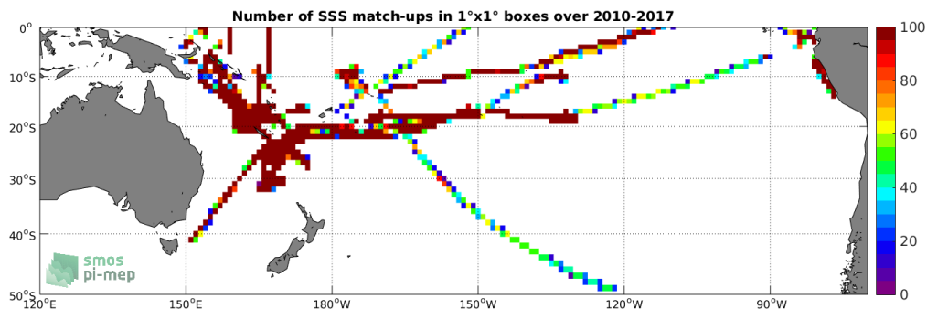
Figure 4: Number of SSS match-ups between TSG-GOSUD-Research-vessel SSS and the SMOS L3 v2 - Monthly - 0.25 Deg (CATDS-CECOS-IFREMER) SSS product for the South Pacific Ocean Pi-MEP region over 1^\circ \times 1^\circ boxes and for the full satellite product period.
