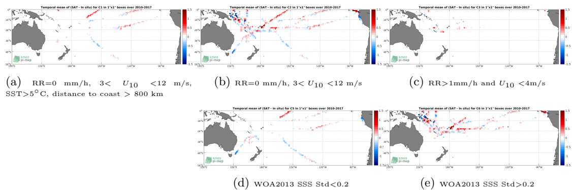
Figure 12: Temporal mean gridded over spatial boxes of size 1^\circ \times 1^\circ of \Delta SSS (SMOS L3 v2 - Monthly - 0.25 Deg (CATDS-CECOS-IFREMER) - TSG-GOSUD-Research-vessel) for 5 different subdatasets corresponding to: RR=0 mm/h, 3 < U_{10} < 12 m/s, SST > 5°C, distance to coast > 800 km (a), RR=0 mm/h, 3 < U_{10} < 12 m/s (b), RR > 1mm/h and U_{10} < 4 m/s (c), WOA2013 SSS Std < 0.2 (d), WOA2013 SSS Std > 0.2 (e).
