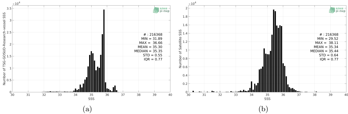
Figure 2: Histograms of SSS from TSG-GOSUD-Research-vessel (a) and SMOS L3 v2 - Monthly - 0.25 Deg (CATDS-CECOS-IFREMER) (b) considering all match-up pairs per bins of 0.1 over the South Pacific Ocean Pi-MEP region and for the full satellite product period.
