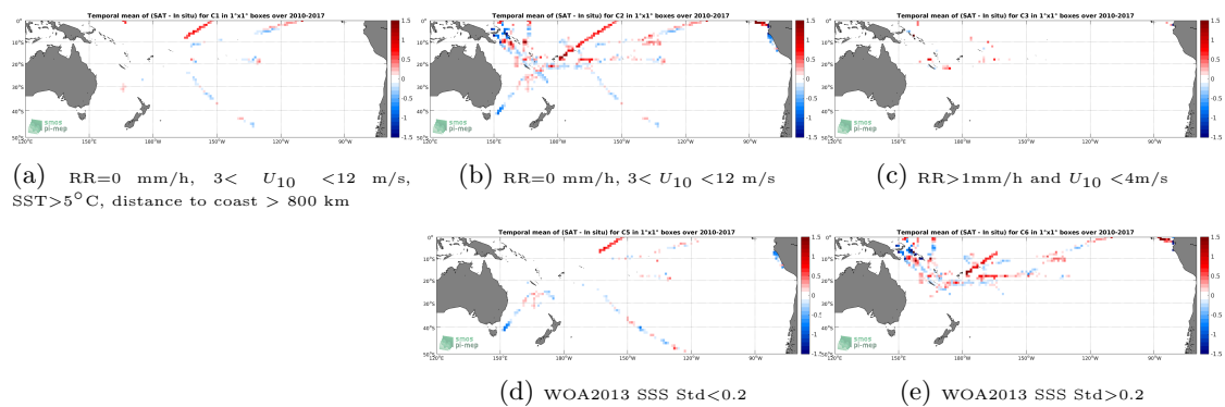
Figure 12: Temporal mean gridded over spatial boxes of size 1^\circ \times 1^\circ of \Delta SSS (SMOS-L3-CATDS-IFREMER-CECOS-V2-MONTHLY-0.25DEG - TSG-GOSUD-Research-vessel) for 5 different subdatasets corresponding to: RR=0 mm/h, 3 < U_{10} < 12 m/s, SST > 5°C, distance to coast > 800 km (a), RR=0 mm/h, 3 < U_{10} < 12 m/s (b), RR > 1mm/h and U_{10} < 4 m/s (c), WOA2013 SSS Std < 0.2 (d), WOA2013 SSS Std > 0.2 (e).
