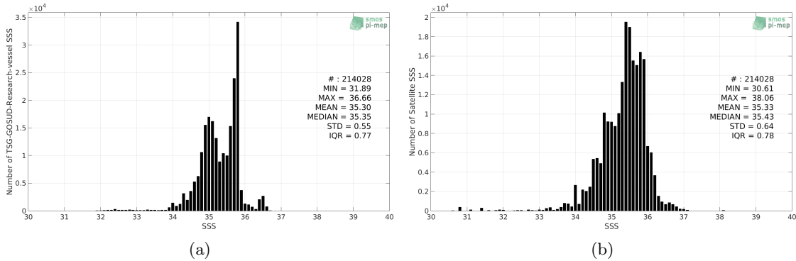
Figure 2: Histograms of SSS from TSG-GOSUD-Research-vessel (a) and SMOS-L3-CATDS-IFREMER-CECOS-V2-MONTHLY-0.25DEG (b) considering all match-up pairs per bins of 0.1 over the South Pacific Ocean Pi-MEP region and for the full satellite product period.
