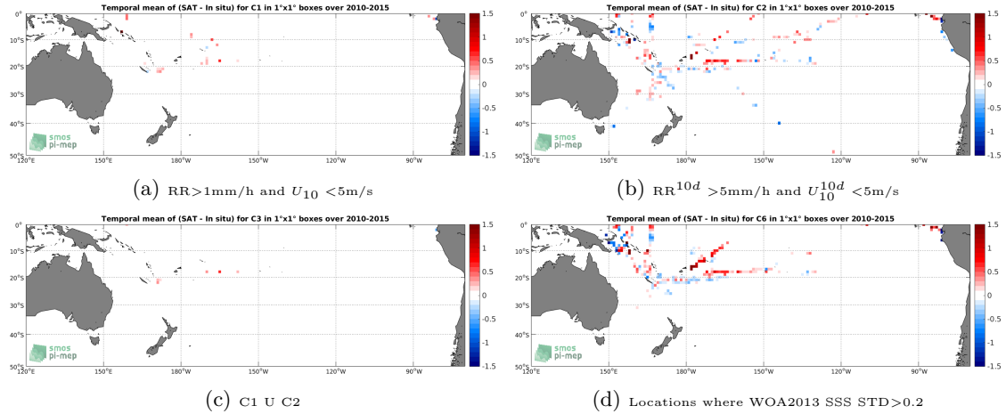
Figure 12: Temporal mean gridded over spatial boxes of size 1^\circ \times 1^\circ of \Delta SSS (SMOS-L3-CATDS-IFREMER-CECOS-V2-MONTHLY-0.25DEG - TSG-GOSUD-Research-vessel) for 4 different subdatasets corresponding to: RR > 1\text{mm/h} and U_{10} < 5\text{m/s} (a), RR^{10d} > 5\text{mm/h} and U_{10}^{10d} < 5\text{m/s} (b), C1 U C2 (c), Locations where WOA2013 SSS STD > 0.2 (d).
