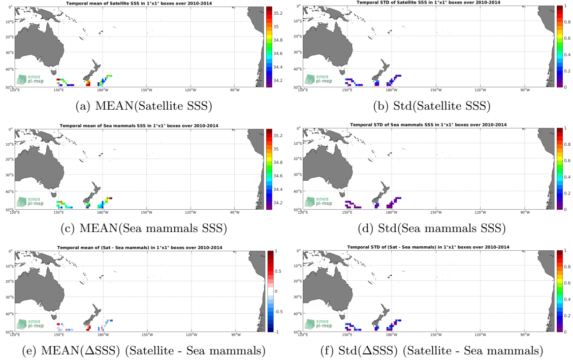
Figure 6: Temporal mean (left) and Std (right) of SSS from SMOS SSS L3 v2 - Monthly - 0.25 Deg (CATDS-CECOS-IFREMER) (top), Sea mammals ( in situ ) (middle), and of \Delta SSS (Satellite - Sea mammals). Only match-up pairs are used to generate these maps.
