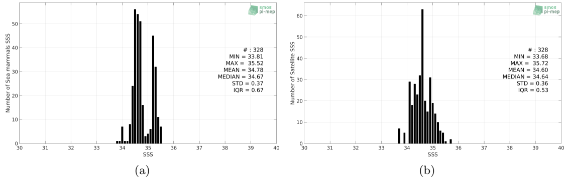
Figure 2: Histograms of SSS from Sea mammals (a) and SMOS SSS L3 v2 - Monthly - 0.25 Deg (CATDS-CECOS-IFREMER) (b) considering all match-up pairs per bins of 0.1 over the South Pacific Ocean Pi-MEP region and for the full satellite product period.
