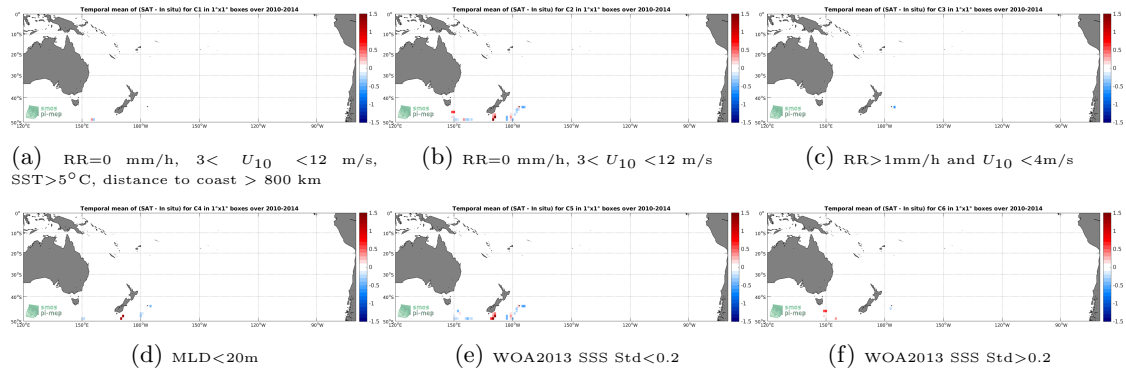
Figure 12: Temporal mean gridded over spatial boxes of size 1^{\circ}\times 1^{\circ} of \Delta\text{SSS} (SMOS SSS L3 v2 - Monthly - 0.25 Deg (CATDS-CECOS-IFREMER) - Sea mammals) for 6 different subdatasets corresponding to: RR=0 mm/h, 3 < U_{10} < 12 m/s, SST > 5^{\circ}\text{C} , distance to coast > 800 km (a), RR=0 mm/h, 3 < U_{10} < 12 m/s (b), RR > 1\text{mm/h} and U_{10} < 4\text{m/s} (c), MLD < 20\text{m} (d), WOA2013 SSS Std < 0.2 (e), WOA2013 SSS Std > 0.2 (f).
