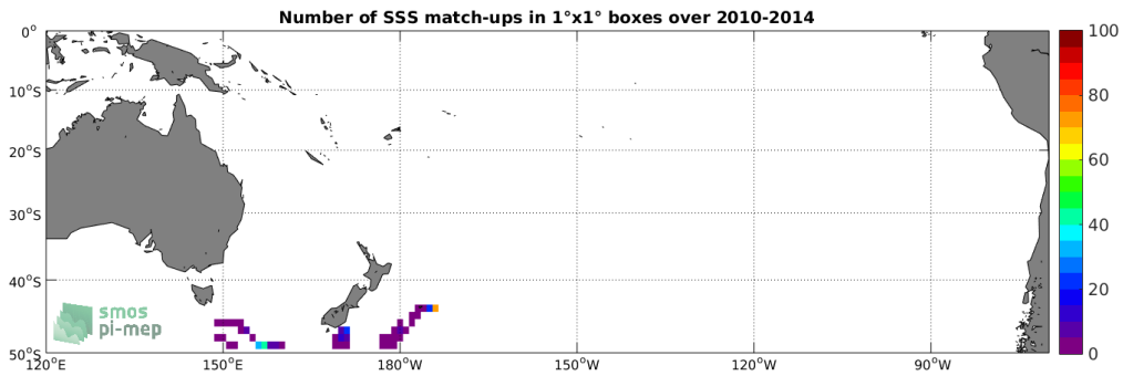
Figure 4: Number of SSS match-ups between Sea mammals SSS and the SMOS SSS L3 v2 - Monthly - 0.25 Deg (CATDS-CECOS-IFREMER) SSS product for the South Pacific Ocean Pi-MEP region over 1°x1° boxes and for the full satellite product period.
