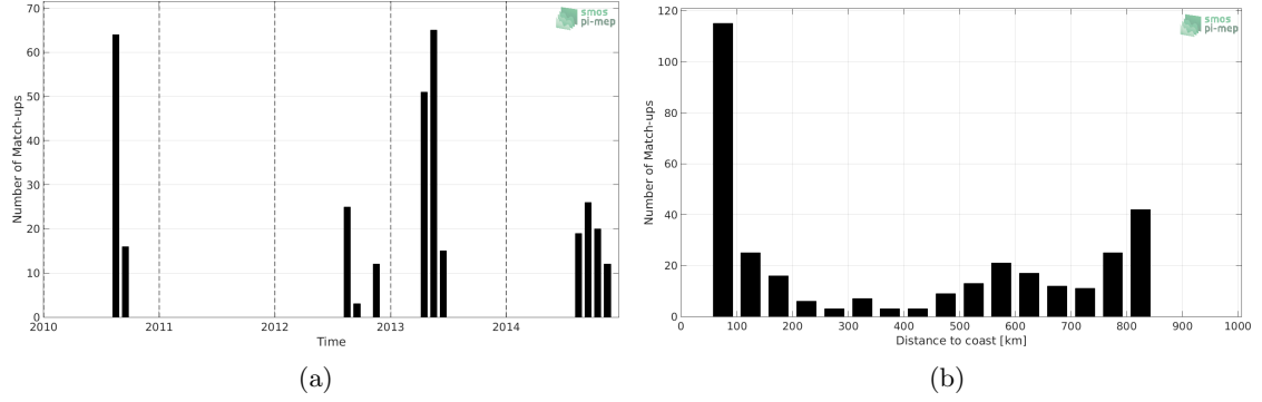
Figure 1: Number of match-ups between Sea mammals and SMOS-L3-CATDS-IFREMER-CECOS-V2-MONTHLY-0.25DEG SSS as a function of time (a) and as function of the distance to coast (b) over the South Pacific Ocean Pi-MEP region and for the full satellite product period.
