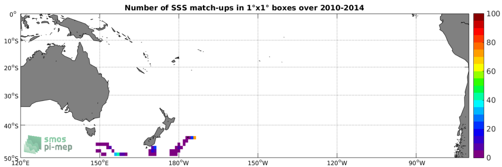
Figure 4: Number of SSS match-ups between Sea mammals SSS and the SMOS-L3-CATDS-IFREMER-CECOS-V2-MONTHLY-0.25DEG SSS product for the South Pacific Ocean Pi-MEP region over 1^\circ \times 1^\circ boxes and for the full satellite product period.
