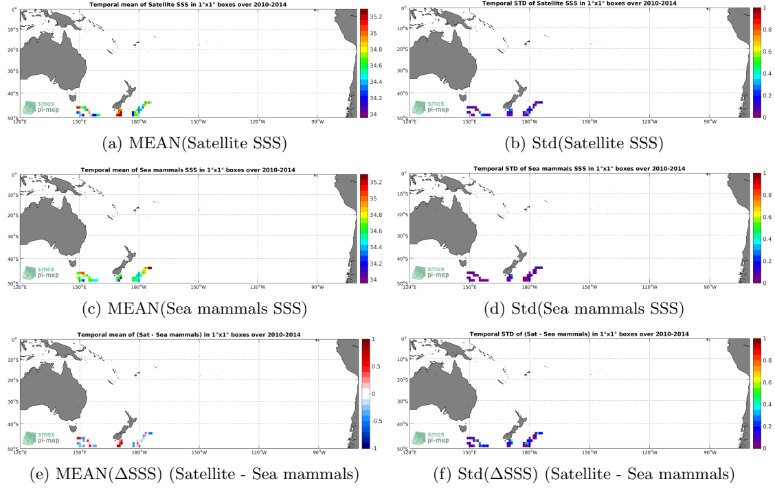
Figure 6: Temporal mean (left) and Std (right) of SSS from SMOS-L3-CATDS-IFREMER-CECOS-V2-MONTHLY-0.25DEG (top), Sea mammals (middle), and of \Delta SSS (Satellite - Sea mammals). Only match-up pairs are used to generate these maps.
