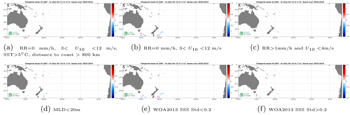
Figure 12: Temporal mean gridded over spatial boxes of size 1^\circ \times 1^\circ of \Delta SSS (SMOS-L3-CATDS-IFREMER-CECOS-V2-MONTHLY-0.25DEG - Sea mammals) for 6 different subdatasets corresponding to: RR=0 mm/h, 3 < U_{10} < 12 m/s, SST > 5^\circ C , distance to coast > 800 km (a), RR=0 mm/h, 3 < U_{10} < 12 m/s (b), RR > 1 mm/h and U_{10} < 4 m/s (c), MLD < 20 m (d), WOA2013 SSS Std < 0.2 (e), WOA2013 SSS Std > 0.2 (f).
