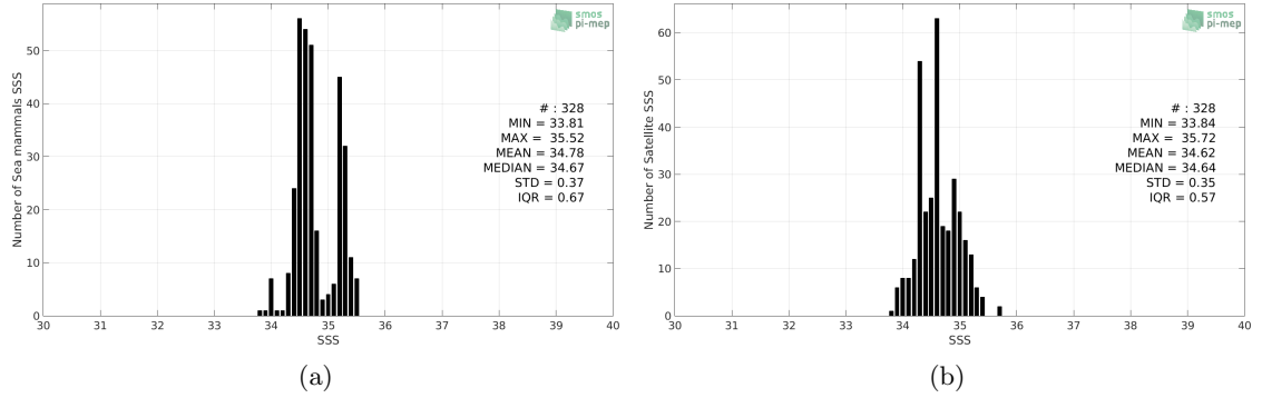
Figure 2: Histograms of SSS from Sea mammals (a) and SMOS-L3-CATDS-IFREMER-CECOS-V2-MONTHLY-0.25DEG (b) considering all match-up pairs per bins of 0.1 over the South Pacific Ocean Pi-MEP region and for the full satellite product period.
