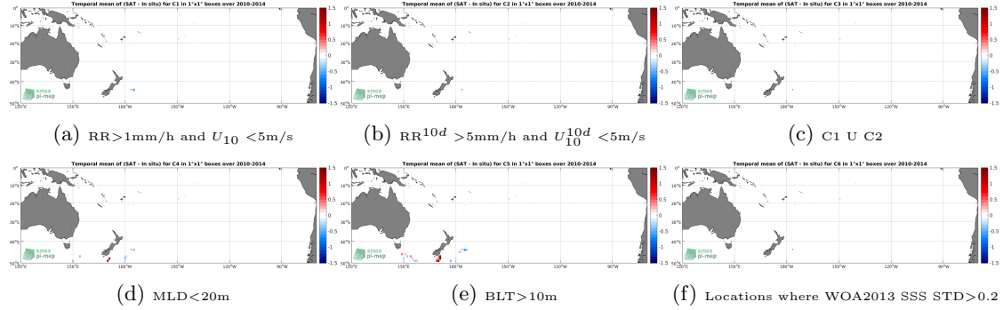
Figure 12: Temporal mean gridded over spatial boxes of size 1^\circ \times 1^\circ of \Delta\text{SSS} (SMOS-L3-CATDS-IFREMER-CECOS-V2-MONTHLY-0.25DEG - Sea mammals) for 6 different subdatasets corresponding to: \text{RR}>1\text{mm/h} and U_{10}<5\text{m/s} (a), \text{RR}^{10d}>5\text{mm/h} and U_{10}^{10d}<5\text{m/s} (b), C1 U C2 (c), \text{MLD}<20\text{m} (d), \text{BLT}>10\text{m} (e), Locations where WOA2013 SSS STD >0.2 (f).
