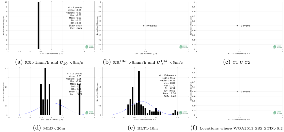
Figure 13: Normalized histogram of \Delta\text{SSS} (SMOS-L3-CATDS-IFREMER-CECOS-V2-MONTHLY-0.25DEG - Sea mammals) for 6 different subdatasets corresponding to: \text{RR}>1\text{mm/h} and U_{10}<5\text{m/s} (a), \text{RR}^{10d}>5\text{mm/h} and U_{10}^{10d}<5\text{m/s} (b), C1 U C2 (c), \text{MLD}<20\text{m} (d), \text{BLT}>10\text{m} (e), Locations where WOA2013 SSS STD >0.2 (f).
