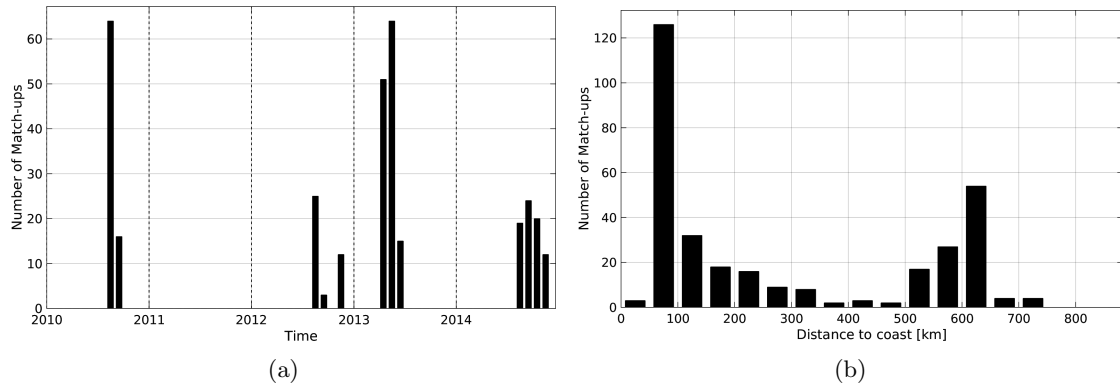
Figure 1: Number of match-ups between Sea mammals and SMOS-L3-CATDS-IFREMER-CECOS-V2-MONTHLY-0.25DEG SSS as a function of time (a) and as function of the distance to coast (b) over the South Pacific Ocean Pi-MEP region and for the full satellite product period.
