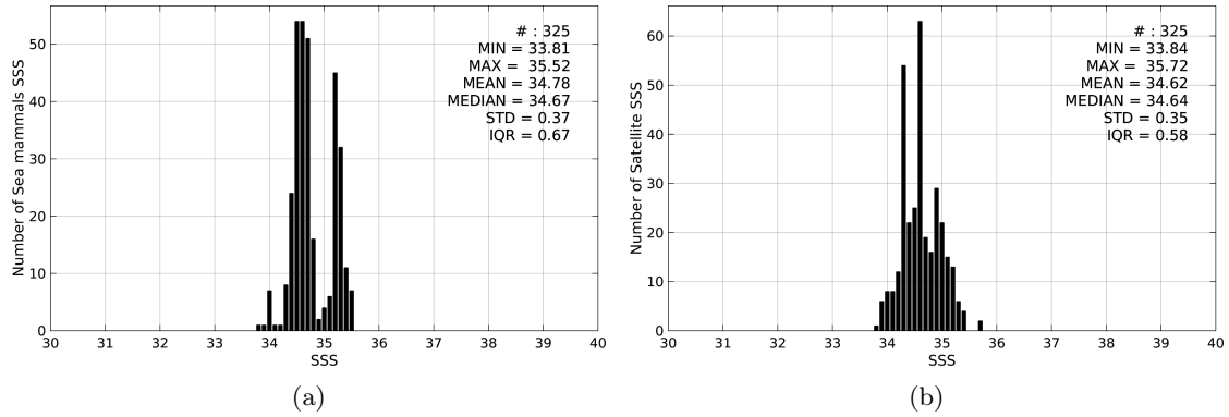
Figure 2: Histograms of SSS from Sea mammals (a) and SMOS-L3-CATDS-IFREMER-CECOS-V2-MONTHLY-0.25DEG (b) considering all match-up pairs per bins of 0.1 over the South Pacific Ocean Pi-MEP region and for the full satellite product period.
