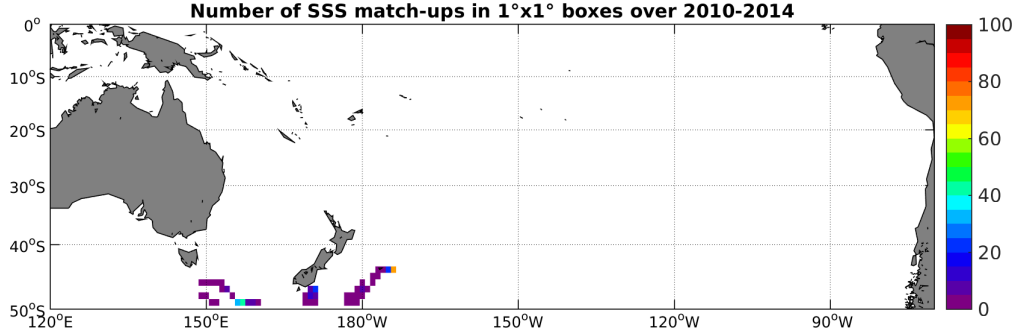
Figure 4: Number of SSS match-ups between Sea mammals SSS and the SMOS-L3-CATDS-IFREMER-CECOS-V2-MONTHLY-0.25DEG SSS product for the South Pacific Ocean Pi-MEP region over 1°x1° boxes and for the full satellite product period.
