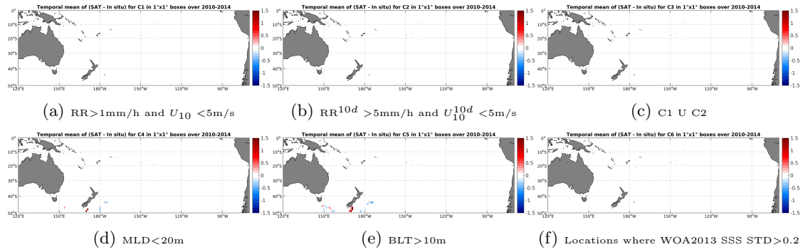
Figure 12: Temporal mean gridded over spatial boxes of size 1^\circ \times 1^\circ of \Delta SSS (SMOS-L3-CATDS-IFREMER-CECOS-V2-MONTHLY-0.25DEG - Sea mammals) for 6 different subdatasets corresponding to: RR > 1\text{mm/h} and U_{10} < 5\text{m/s} (a), RR^{10d} > 5\text{mm/h} and U_{10}^{10d} < 5\text{m/s} (b), C1 U C2 (c), MLD < 20\text{m} (d), BLT > 10\text{m} (e), Locations where WOA2013 SSS STD > 0.2 (f).
