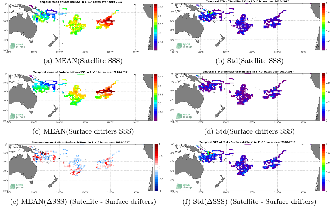
Figure 5: Temporal mean (left) and Std (right) of SSS from SMOS L3 v2 - Monthly - 0.25 Deg (CATDS-CECOS-IFREMER) (top), Surface drifters (middle), and of \Delta SSS (Satellite - Surface drifters). Only match-up pairs are used to generate these maps.
