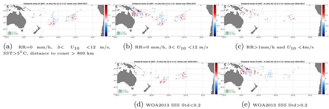
Figure 11: Temporal mean gridded over spatial boxes of size 1^{\circ}\times 1^{\circ} of \Delta\text{SSS} (SMOS L3 v2 - Monthly - 0.25 Deg (CATDS-CECOS-IFREMER) - Surface drifters) for 5 different subdatasets corresponding to: \text{RR}=0 mm/h, 3 < U_{10} < 12 m/s, \text{SST} > 5^{\circ}\text{C} , distance to coast > 800 km (a), \text{RR}=0 mm/h, 3 < U_{10} < 12 m/s (b), \text{RR} > 1\text{mm/h} and U_{10} < 4\text{m/s} (c), WOA2013 SSS Std < 0.2 (d), WOA2013 SSS Std > 0.2 (e).
