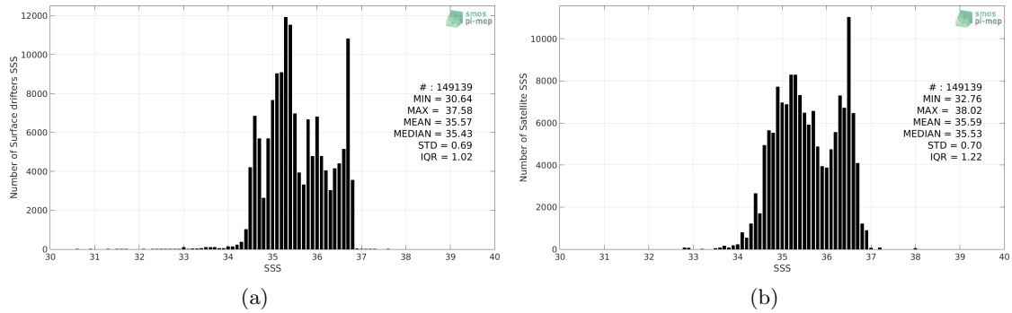
Figure 2: Histograms of SSS from Surface drifters (a) and SMOS L3 v2 - Monthly - 0.25 Deg (CATDS-CECOS-IFREMER) (b) considering all match-up pairs per bins of 0.1 over the South Pacific Ocean Pi-MEP region and for the full satellite product period.
