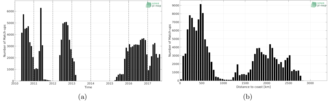
Figure 1: Number of match-ups between Surface drifters and SMOS L3 v2 - Monthly - 0.25 Deg (CATDS-CECOS-IFREMER) SSS as a function of time (a) and as function of the distance to coast (b) over the South Pacific Ocean Pi-MEP region and for the full satellite product period.
