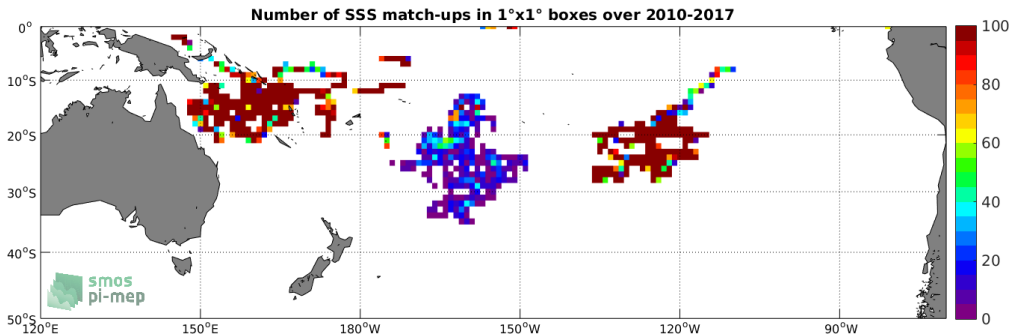
Figure 3: Number of SSS match-ups between Surface drifters SSS and the SMOS L3 v2 - Monthly - 0.25 Deg (CATDS-CECOS-IFREMER) SSS product for the South Pacific Ocean Pi-MEP region over 1^\circ \times 1^\circ boxes and for the full satellite product period.
