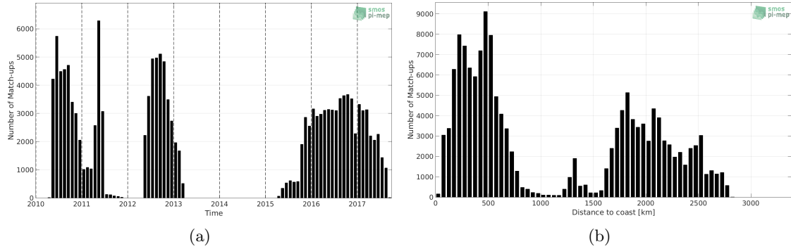
Figure 1: Number of match-ups between Surface drifters and SMOS-L3-CATDS-IFREMER-CECOS-V2-MONTHLY-0.25DEG SSS as a function of time (a) and as function of the distance to coast (b) over the South Pacific Ocean Pi-MEP region and for the full satellite product period.
