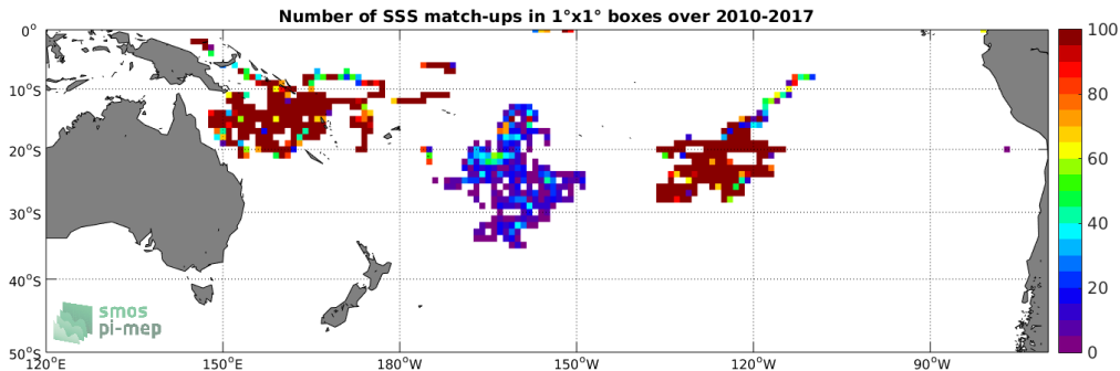
Figure 3: Number of SSS match-ups between Surface drifters SSS and the SMOS-L3-CATDS-IFREMER-CECOS-V2-MONTHLY-0.25DEG SSS product for the South Pacific Ocean Pi-MEP region over 1^{\circ} \times 1^{\circ} boxes and for the full satellite product period.
