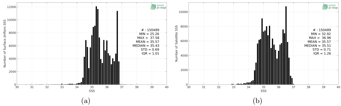
Figure 2: Histograms of SSS from Surface drifters (a) and SMOS-L3-CATDS-IFREMER-CECOS-V2-MONTHLY-0.25DEG (b) considering all match-up pairs per bins of 0.1 over the South Pacific Ocean Pi-MEP region and for the full satellite product period.
