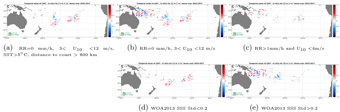
Figure 11: Temporal mean gridded over spatial boxes of size 1^\circ \times 1^\circ of \Delta SSS (SMOS-L3-CATDS-IFREMER-CECOS-V2-MONTHLY-0.25DEG - Surface drifters) for 5 different subdatasets corresponding to:RR=0 mm/h, 3 < U_{10} < 12 m/s, SST >5^\circ C, distance to coast > 800 km (a), RR=0 mm/h, 3 < U_{10} < 12 m/s (b), RR >1 mm/h and U_{10} < 4 m/s (c), WOA2013 SSS Std <0.2 (d), WOA2013 SSS Std >0.2 (e).
