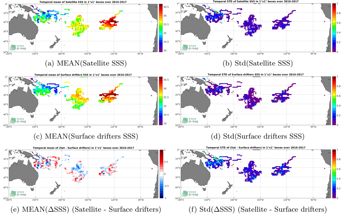
Figure 5: Temporal mean (left) and Std (right) of SSS from SMOS-L3-CATDS-IFREMER-CECOS-V2-MONTHLY-0.25DEG (top), Surface drifters (middle), and of \Delta SSS (Satellite - Surface drifters). Only match-up pairs are used to generate these maps.
