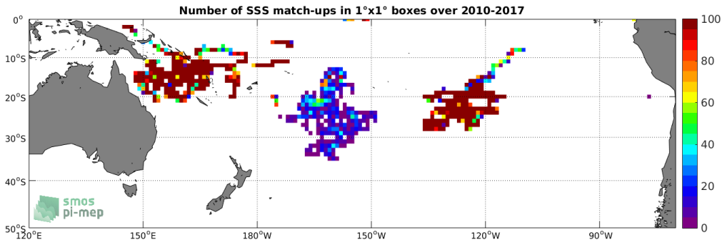
Figure 3: Number of SSS match-ups between Surface drifters SSS and the SMOS-L3-CATDS-IFREMER-CECOS-V2-MONTHLY-0.25DEG SSS product for the South Pacific Ocean Pi-MEP region over 1^\circ \times 1^\circ boxes and for the full satellite product period.
