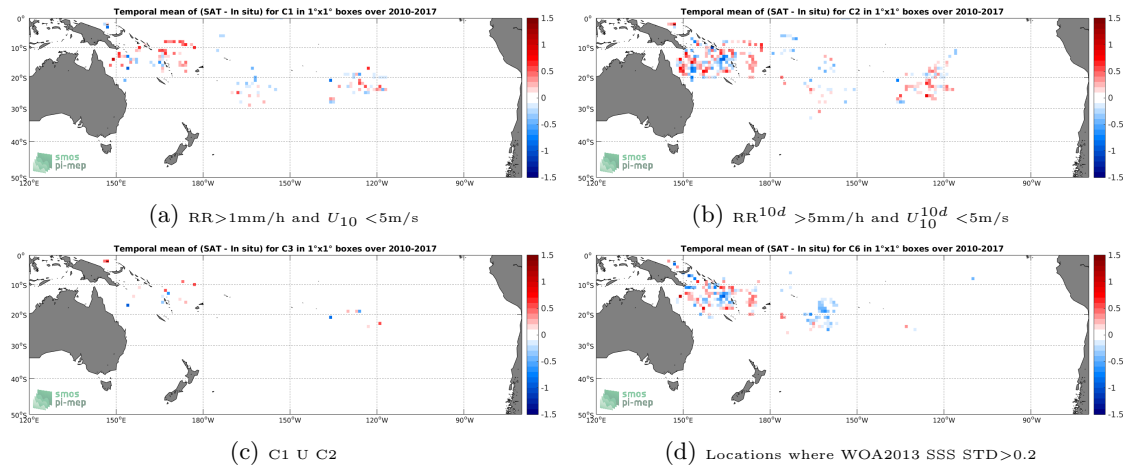
Figure 11: Temporal mean gridded over spatial boxes of size 1^\circ \times 1^\circ of \Delta SSS (SMOS-L3-CATDS-IFREMER-CECOS-V2-MONTHLY-0.25DEG - Surface drifters) for 4 different subdatasets corresponding to: RR > 1\text{mm/h} and U_{10} < 5\text{m/s} (a), RR^{10d} > 5\text{mm/h} and U_{10}^{10d} < 5\text{m/s} (b), C1 U C2 (c), Locations where WOA2013 SSS STD > 0.2 (d).
