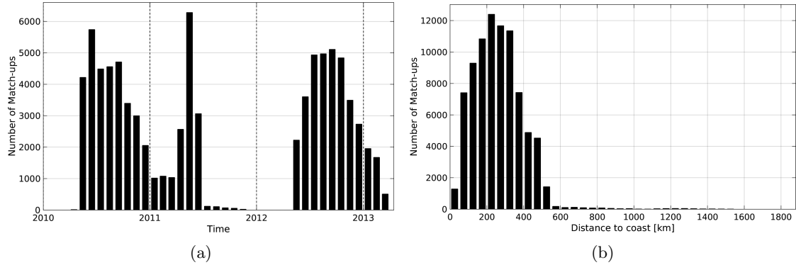
Figure 1: Number of match-ups between Surface drifters and SMOS-L3-CATDS-IFREMER-CECOS-V2-MONTHLY-0.25DEG SSS as a function of time (a) and as function of the distance to coast (b) over the South Pacific Ocean Pi-MEP region and for the full satellite product period.
