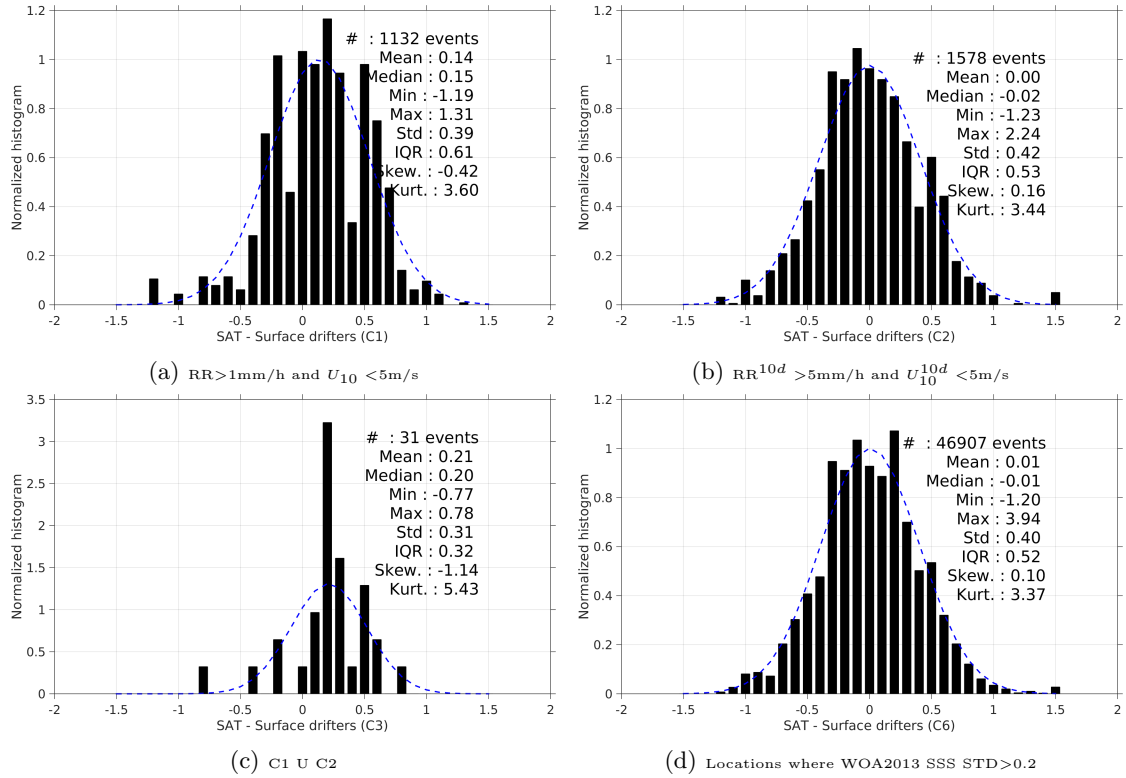
Figure 12: Normalized histogram of \Delta\text{SSS} (SMOS-L3-CATDS-IFREMER-CECOS-V2-MONTHLY-0.25DEG - Surface drifters) for 6 different subdatasets corresponding to: RR > 1mm/h and U_{10} < 5\text{m/s} (a), RR^{10d} > 5\text{mm/h} and U_{10}^{10d} < 5\text{m/s} (b), C1 U C2 (c), Locations where WOA2013 SSS STD > 0.2 (d).
