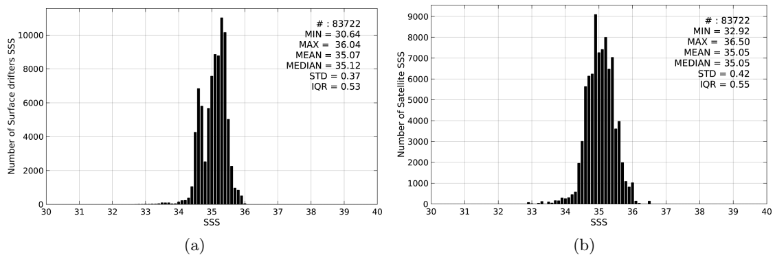
Figure 2: Histograms of SSS from Surface drifters (a) and SMOS-L3-CATDS-IFREMER-CECOS-V2-MONTHLY-0.25DEG (b) considering all match-up pairs per bins of 0.1 over the South Pacific Ocean Pi-MEP region and for the full satellite product period.
