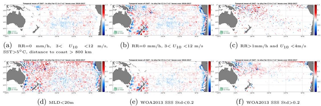
Figure 12: Temporal mean gridded over spatial boxes of size 1^\circ \times 1^\circ of \Delta SSS (SMOS-L3-CATDS-IFREMER-CECOS-V2-MONTHLY-0.25DEG - Argo) for 6 different subdatasets corresponding to:RR=0 mm/h, 3 < U_{10} < 12 m/s, SST >5^\circ\text{C} , distance to coast > 800 km (a), RR=0 mm/h, 3 < U_{10} < 12 m/s (b), RR >1 mm/h and U_{10} < 4 m/s (c),MLD <20 m (d),WOA2013 SSS Std <0.2 (e),WOA2013 SSS Std >0.2 (f).
