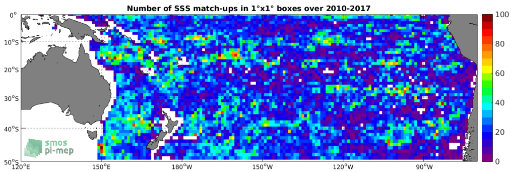
Figure 4: Number of SSS match-ups between Argos SSS and the SMOS-L3-CATDS-IFREMER-CECOS-V2-MONTHLY-0.25DEG SSS product for the South Pacific Ocean Pi-MEP region over 1^\circ \times 1^\circ boxes and for the full satellite product period.
