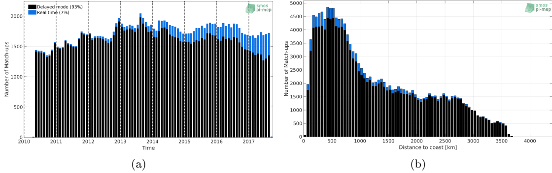
Figure 1: Number of match-ups between Argo and SMOS-L3-CATDS-IFREMER-CECOS-V2-MONTHLY-0.25DEG SSS as a function of time (a) and as function of the distance to coast (b) over the South Pacific Ocean Pi-MEP region and for the full satellite product period.
