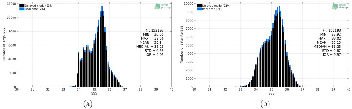
Figure 2: Histograms of SSS from Argo (a) and SMOS-L3-CATDS-IFREMER-CECOS-V2-MONTHLY-0.25DEG (b) considering all match-up pairs per bins of 0.1 over the South Pacific Ocean Pi-MEP region and for the full satellite product period.
