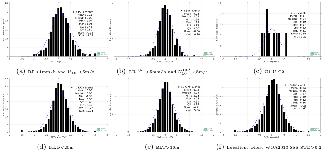
Figure 13: Normalized histogram of \Delta SSS (SMOS-L3-CATDS-IFREMER-CECOS-V2-MONTHLY-0.25DEG - Argo) for 6 different subdatasets corresponding to: RR>1mm/h and U_{10} < 5m/s (a), RR^{10d} > 5mm/h and U_{10}^{10d} < 5m/s (b), C1 U C2 (c),MLD<20m (d),BLT>10m (e),Locations where WOA2013 SSS STD>0.2 (f).
