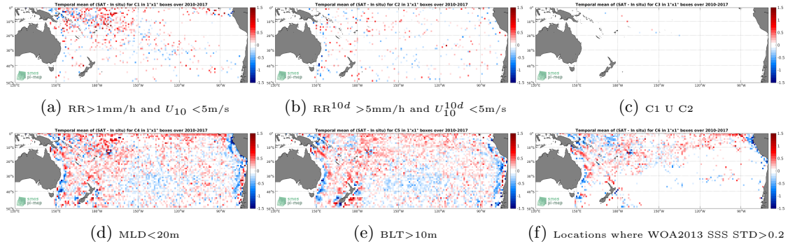
Figure 12: Temporal mean gridded over spatial boxes of size 1°x1° of \Delta SSS (SMOS-L3-CATDS-IFREMER-CECOS-V2-MONTHLY-0.25DEG - Argo) for 6 different subdatasets corresponding to:RR>1mm/h and U_{10} < 5m/s (a), RR^{10d} > 5mm/h and U_{10}^{10d} < 5m/s (b), C1 U C2 (c),MLD<20m (d),BLT>10m (e),Locations where WOA2013 SSS STD>0.2 (f).
