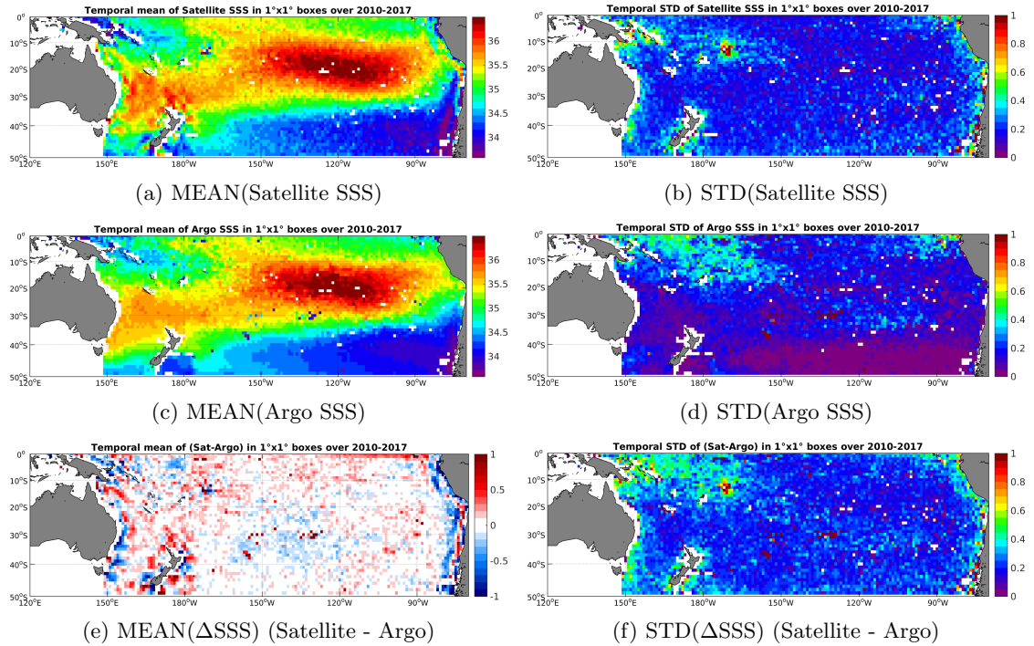
Figure 6: Temporal mean (left) and STD (right) of SSS from SMOS-L3-CATDS-IFREMER-CECOS-V2-MONTHLY-0.25DEG (top), Argo (middle), and of \Delta SSS (Satellite - Argo). Only match-up pairs are used to generate these maps.
