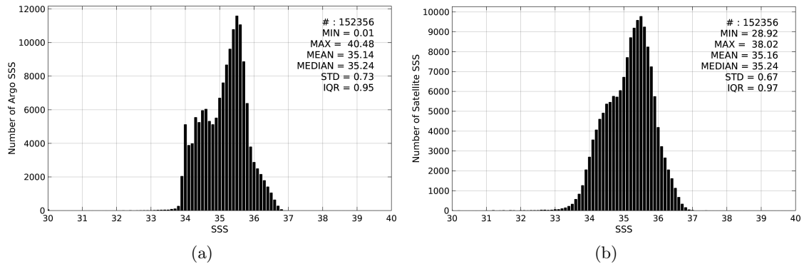
Figure 2: Histograms of SSS from Argo (a) and SMOS-L3-CATDS-IFREMER-CECOS-V2-MONTHLY-0.25DEG (b) considering all match-up pairs per bins of 0.1 over the South Pacific Ocean Pi-MEP region and for the full satellite product period.
