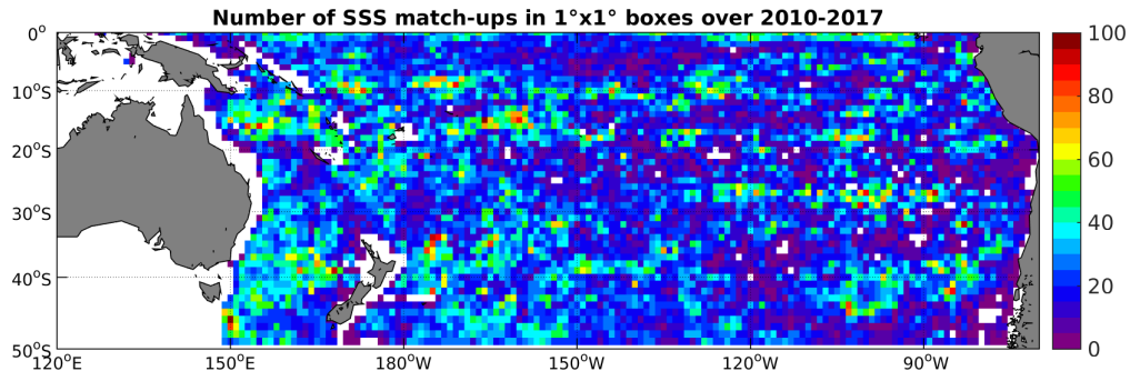
Figure 4: Number of SSS match-ups between Argo SSS and the SMOS-L3-CATDS-IFREMER-CECOS-V2-MONTHLY-0.25DEG SSS product for the South Pacific Ocean Pi-MEP region over 1^\circ \times 1^\circ boxes and for the full satellite product period.
