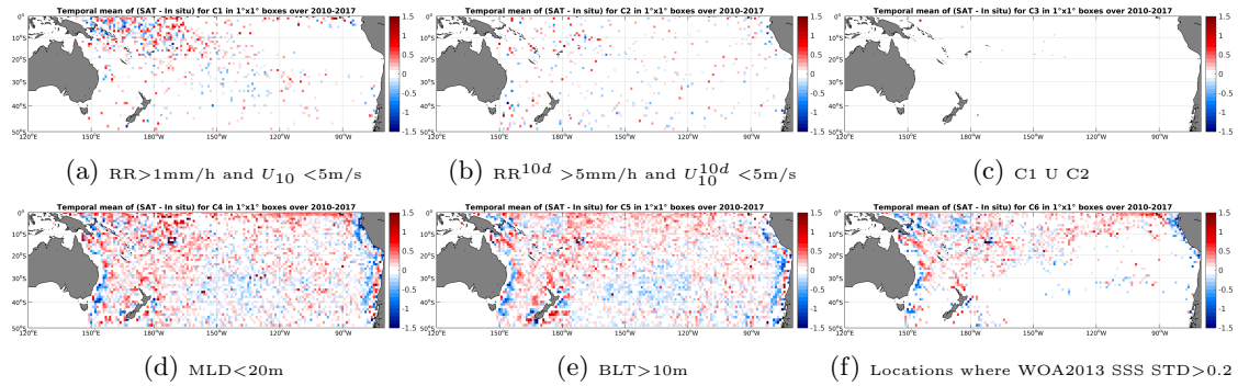
Figure 12: Temporal mean gridded over spatial boxes of size 1^\circ \times 1^\circ of \Delta SSS (SMOS-L3-CATDS-IFREMER-CECOS-V2-MONTHLY-0.25DEG - Argo) for 6 different subdatasets corresponding to:RR >1 mm/h and U_{10} < 5 m/s (a), RR ^{10d} > 5 mm/h and U_{10}^{10d} < 5 m/s (b), C1 U C2 (c),MLD <20 m (d),BLT >10 m (e),Locations where WOA2013 SSS STD >0.2 (f).
