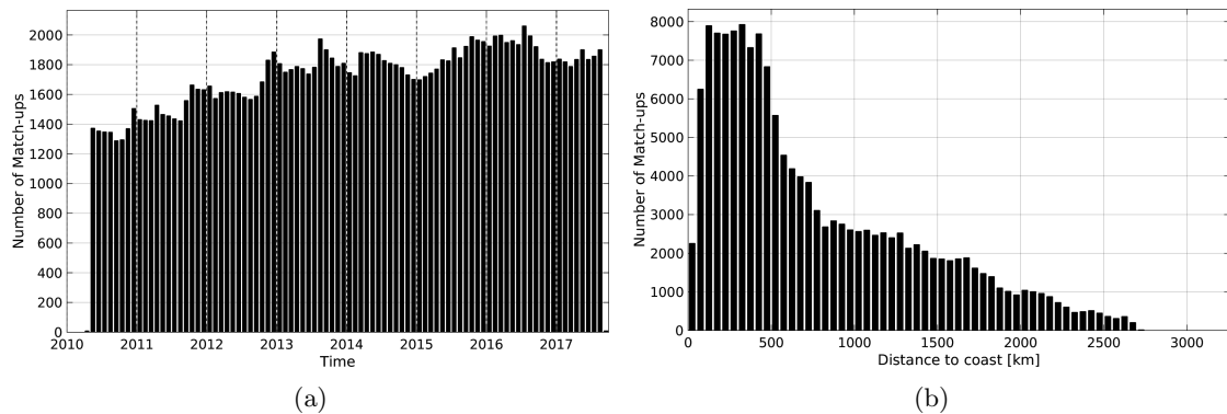
Figure 1: Number of match-ups between Argo and SMOS-L3-CATDS-IFREMER-CECOS-V2-MONTHLY-0.25DEG SSS as a function of time (a) and as function of the distance to coast (b) over the South Pacific Ocean Pi-MEP region and for the full satellite product period.
