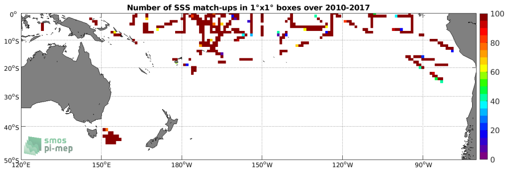
Figure 4: Number of SSS match-ups between TSG (SAMOS) SSS and the SMOS SSS L3 v2 - Daily - 0.5 Deg (CATDS-CECOS-IFREMER) SSS product for the South Pacific Ocean Pi-MEP region over 1^\circ \times 1^\circ boxes and for the full satellite product period.
