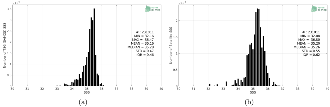
Figure 2: Histograms of SSS from TSG (SAMOS) (a) and SMOS SSS L3 v2 - Daily - 0.5 Deg (CATDS-CECOS-IFREMER) (b) considering all match-up pairs per bins of 0.1 over the South Pacific Ocean Pi-MEP region and for the full satellite product period.
