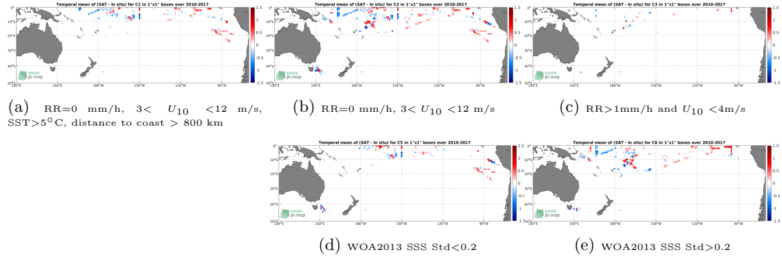
Figure 12: Temporal mean gridded over spatial boxes of size 1^\circ \times 1^\circ of \Delta SSS (SMOS SSS L3 v2 - Daily - 0.5 Deg (CATDS-CECOS-IFREMER) - TSG (SAMOS)) for 5 different subdatasets corresponding to: RR=0 mm/h, 3 < U_{10} < 12 m/s, SST > 5^\circ C , distance to coast > 800 km (a), RR=0 mm/h, 3 < U_{10} < 12 m/s (b), RR > 1 mm/h and U_{10} < 4 m/s (c), WOA2013 SSS Std < 0.2 (d), WOA2013 SSS Std > 0.2 (e).
