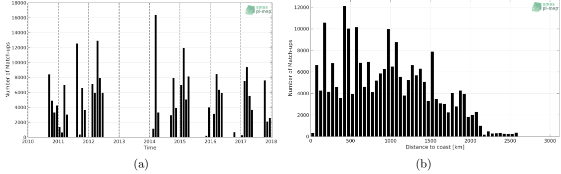
Figure 1: Number of match-ups between TSG (SAMOS) and SMOS SSS L3 v2 - Daily - 0.5 Deg (CATDS-CECOS-IFREMER) SSS as a function of time (a) and as function of the distance to coast (b) over the South Pacific Ocean Pi-MEP region and for the full satellite product period.
