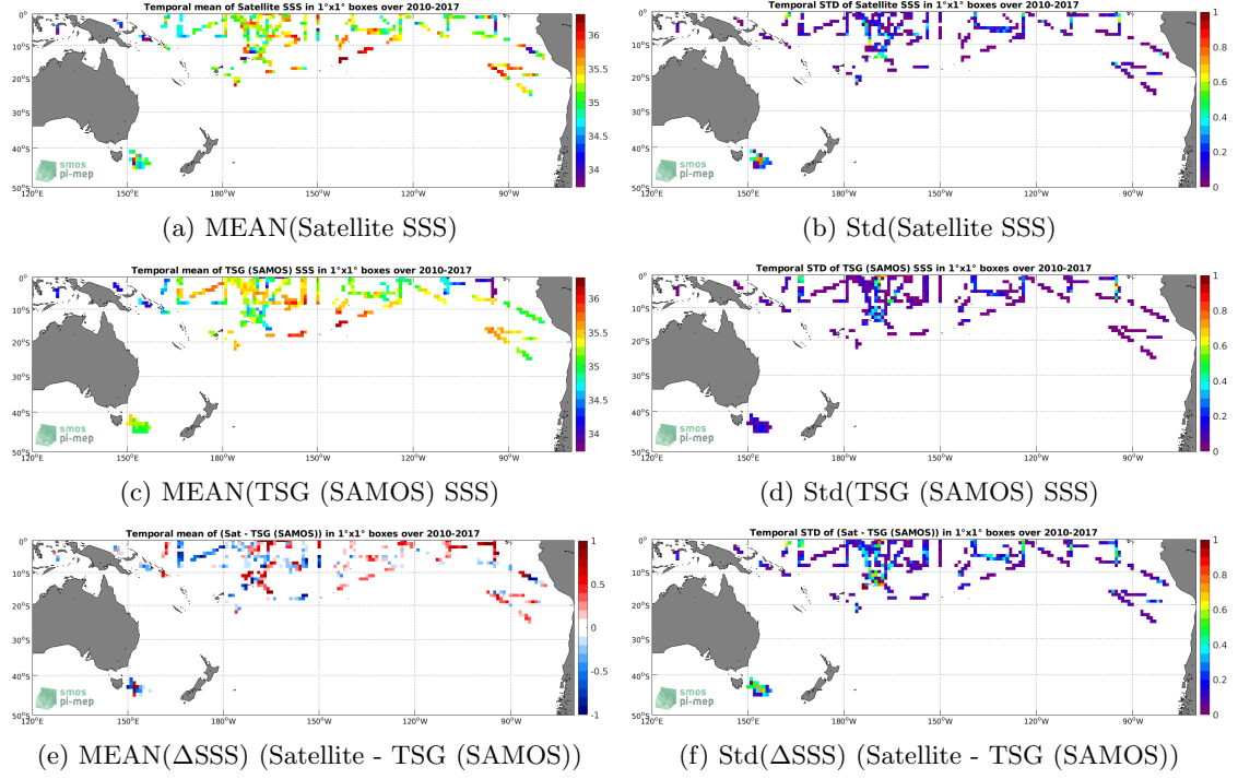
Figure 6: Temporal mean (left) and Std (right) of SSS from SMOS SSS L3 v2 - Daily - 0.5 Deg (CATDS-CECOS-IFREMER) (top), TSG (SAMOS) (middle), and of \Delta SSS (Satellite - TSG (SAMOS)). Only match-up pairs are used to generate these maps.
