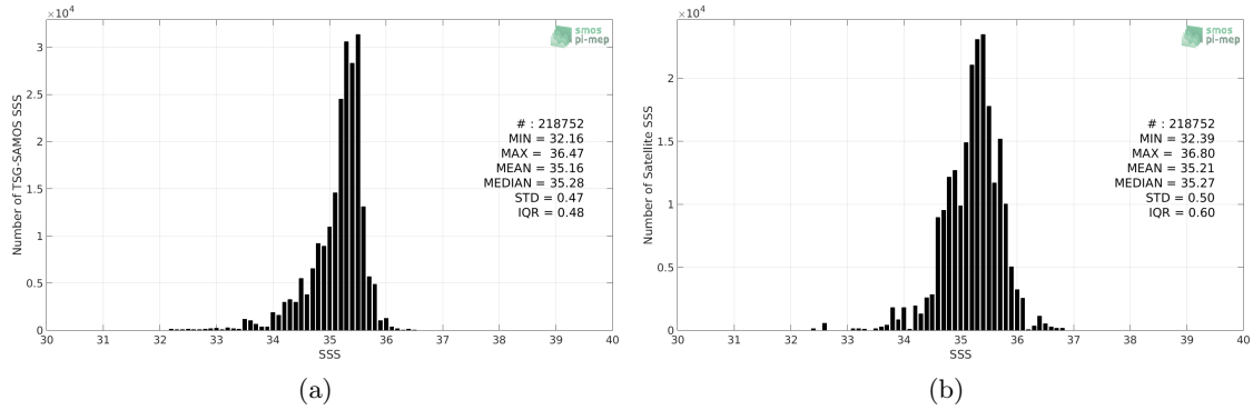
Figure 2: Histograms of SSS from TSG-SAMOS (a) and SMOS L3 v2 - Daily - 0.5 Deg (CATDS-CECOS-IFREMER) (b) considering all match-up pairs per bins of 0.1 over the South Pacific Ocean Pi-MEP region and for the full satellite product period.
