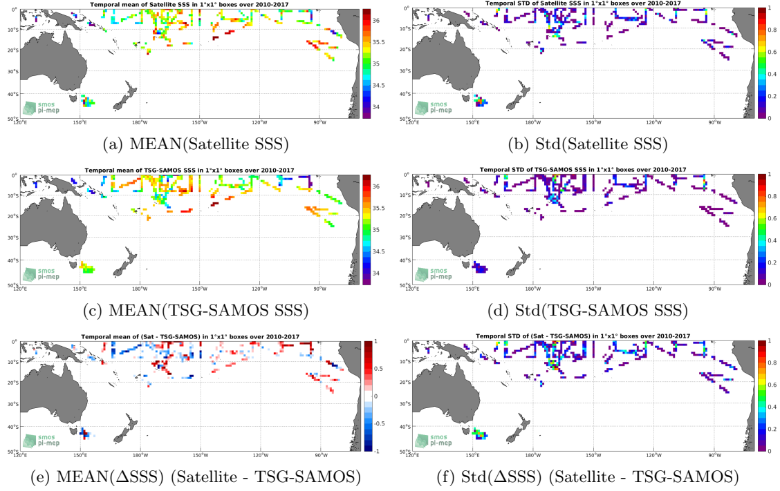
Figure 6: Temporal mean (left) and Std (right) of SSS from SMOS L3 v2 - Daily - 0.5 Deg (CATDS-CECOS-IFREMER) (top), TSG-SAMOS (middle), and of \Delta SSS (Satellite - TSG-SAMOS). Only match-up pairs are used to generate these maps.
