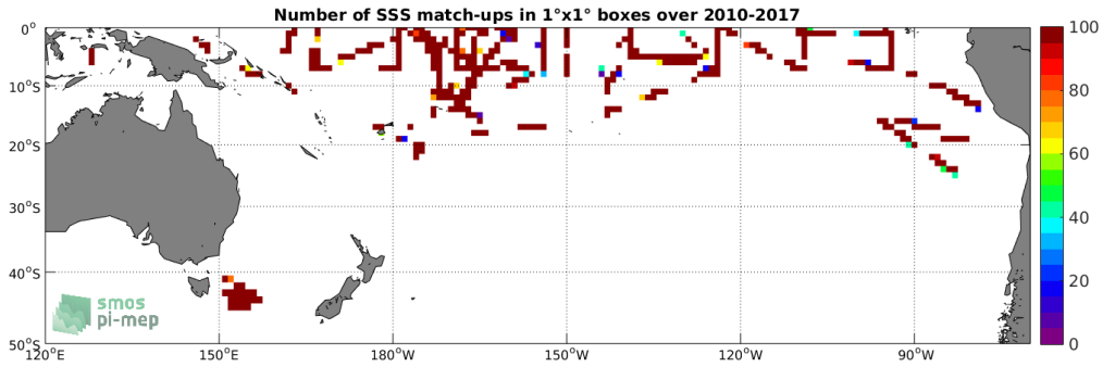
Figure 4: Number of SSS match-ups between TSG-SAMOS SSS and the SMOS-L3-CATDS-CECOS-IFREMER-V2-1DAY-0.5DEG SSS product for the South Pacific Ocean Pi-MEP region over 1°x1° boxes and for the full satellite product period.
