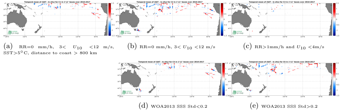
Figure 12: Temporal mean gridded over spatial boxes of size 1^\circ \times 1^\circ of \Delta SSS (SMOS-L3-CATDS-CECOS-IFREMER-V2-1DAY-0.5DEG - TSG-SAMOS) for 5 different subdatasets corresponding to: RR=0 mm/h, 3 < U_{10} < 12 m/s, SST > 5^\circ C , distance to coast > 800 km (a), RR=0 mm/h, 3 < U_{10} < 12 m/s (b), RR > 1 mm/h and U_{10} < 4 m/s (c), WOA2013 SSS Std < 0.2 (d), WOA2013 SSS Std > 0.2 (e).
