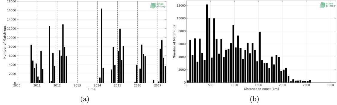
Figure 1: Number of match-ups between TSG-SAMOS and SMOS-L3-CATDS-CECOS-IFREMER-V2-1DAY-0.5DEG SSS as a function of time (a) and as function of the distance to coast (b) over the South Pacific Ocean Pi-MEP region and for the full satellite product period.
