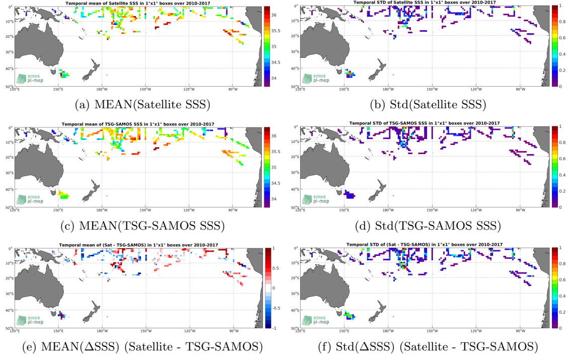
Figure 6: Temporal mean (left) and Std (right) of SSS from SMOS-L3-CATDS-CECOS-IFREMER-V2-1DAY-0.5DEG (top), TSG-SAMOS (middle), and of \Delta SSS (Satellite - TSG-SAMOS). Only match-up pairs are used to generate these maps.
