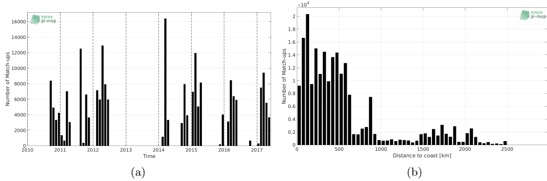
Figure 1: Number of match-ups between TSG-SAMOS and SMOS-L3-CATDS-CECOS-IFREMER-V2-1DAY-0.5DEG SSS as a function of time (a) and as function of the distance to coast (b) over the South Pacific Ocean Pi-MEP region and for the full satellite product period.
