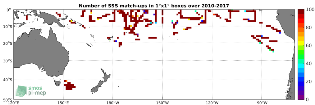
Figure 4: Number of SSS match-ups between TSG-SAMOS SSS and the SMOS-L3-CATDS-CECOS-IFREMER-V2-1DAY-0.5DEG SSS product for the South Pacific Ocean Pi-MEP region over 1^\circ \times 1^\circ boxes and for the full satellite product period.
