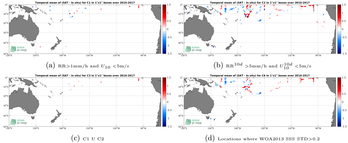
Figure 12: Temporal mean gridded over spatial boxes of size 1^\circ \times 1^\circ of \Delta SSS (SMOS-L3-CATDS-CECOS-IFREMER-V2-1DAY-0.5DEG - TSG-SAMOS) for 4 different subdatasets corresponding to: RR > 1\text{mm/h} and U_{10} < 5\text{m/s} (a), RR^{10d} > 5\text{mm/h} and U_{10}^{10d} < 5\text{m/s} (b), C1 U C2 (c), Locations where WOA2013 SSS STD > 0.2 (d).
