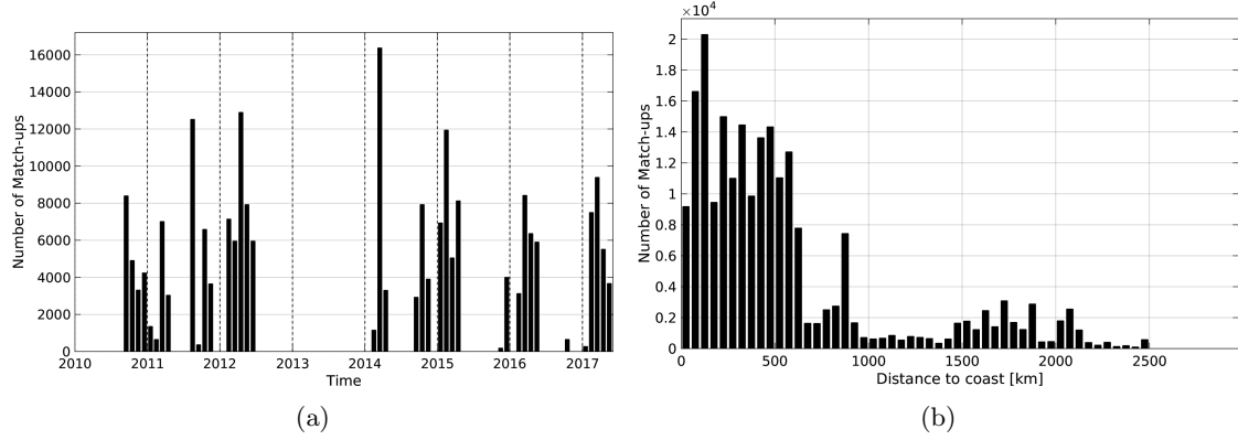
Figure 1: Number of match-ups between TSG-SAMOS and SMOS-L3-CATDS-CECOS-IFREMER-V2-1DAY-0.5DEG SSS as a function of time (a) and as function of the distance to coast (b) over the South Pacific Ocean Pi-MEP region and for the full satellite product period.
