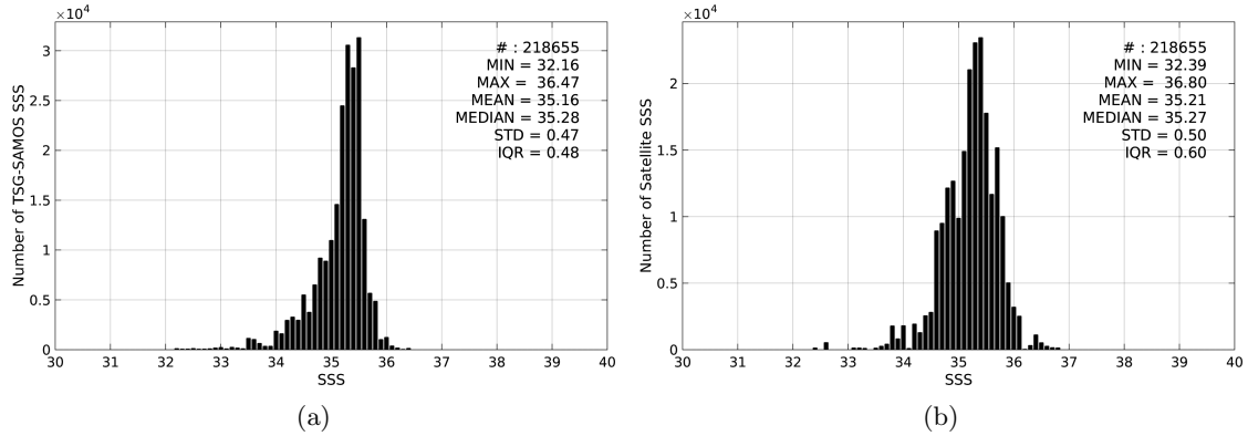
Figure 2: Histograms of SSS from TSG-SAMOS (a) and SMOS-L3-CATDS-CECOS-IFREMER-V2-1DAY-0.5DEG (b) considering all match-up pairs per bins of 0.1 over the South Pacific Ocean Pi-MEP region and for the full satellite product period.
