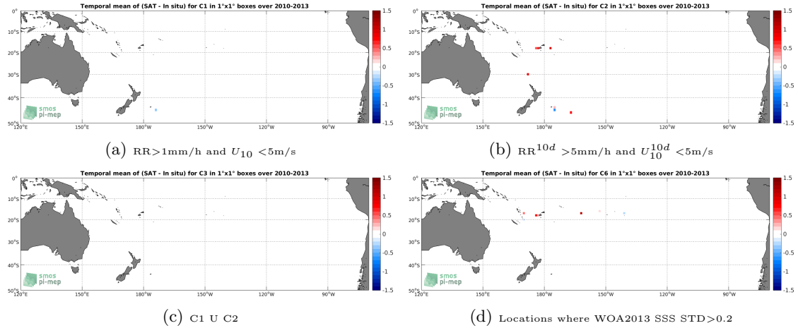
Figure 12: Temporal mean gridded over spatial boxes of size 1^\circ \times 1^\circ of \Delta SSS (SMOS-L3-CATDS-CECOS-IFREMER-V2-1DAY-0.5DEG - TSG-GOSUD-Sailing-ship) for 4 different subdatasets corresponding to: RR > 1\text{mm/h} and U_{10} < 5\text{m/s} (a), RR^{10d} > 5\text{mm/h} and U_{10}^{10d} < 5\text{m/s} (b), C1 U C2 (c), Locations where WOA2013 SSS STD > 0.2 (d).
