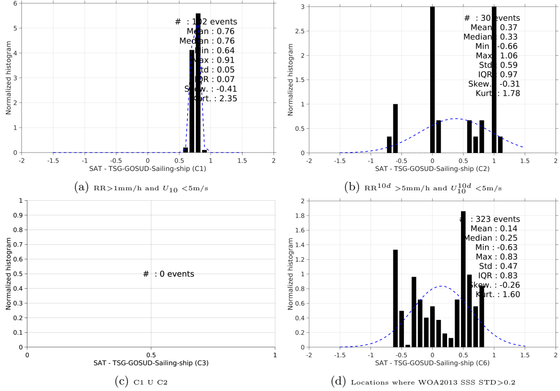
Figure 13: Normalized histogram of \Delta SSS (SMOS-L3-CATDS-CECOS-IFREMER-V2-1DAY-0.5deg - TSG-GOSUD-Sailing-ship) for 6 different subdatasets corresponding to: RR>1mm/h and U_{10} < 5\text{m/s} (a), RR^{10d} > 5\text{mm/h} and U_{10}^{10d} < 5\text{m/s} (b), C1 U C2 (c), Locations where WOA2013 SSS STD>0.2 (d).
