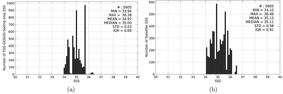
Figure 2: Histograms of SSS from TSG-GOSUD-Sailing-ship (a) and SMOS-L3-CATDS-CECOS-IFREMER-V2-1DAY-0.5deg (b) considering all match-up pairs per bins of 0.1 over the South Pacific Ocean Pi-MEP region and for the full satellite product period.
