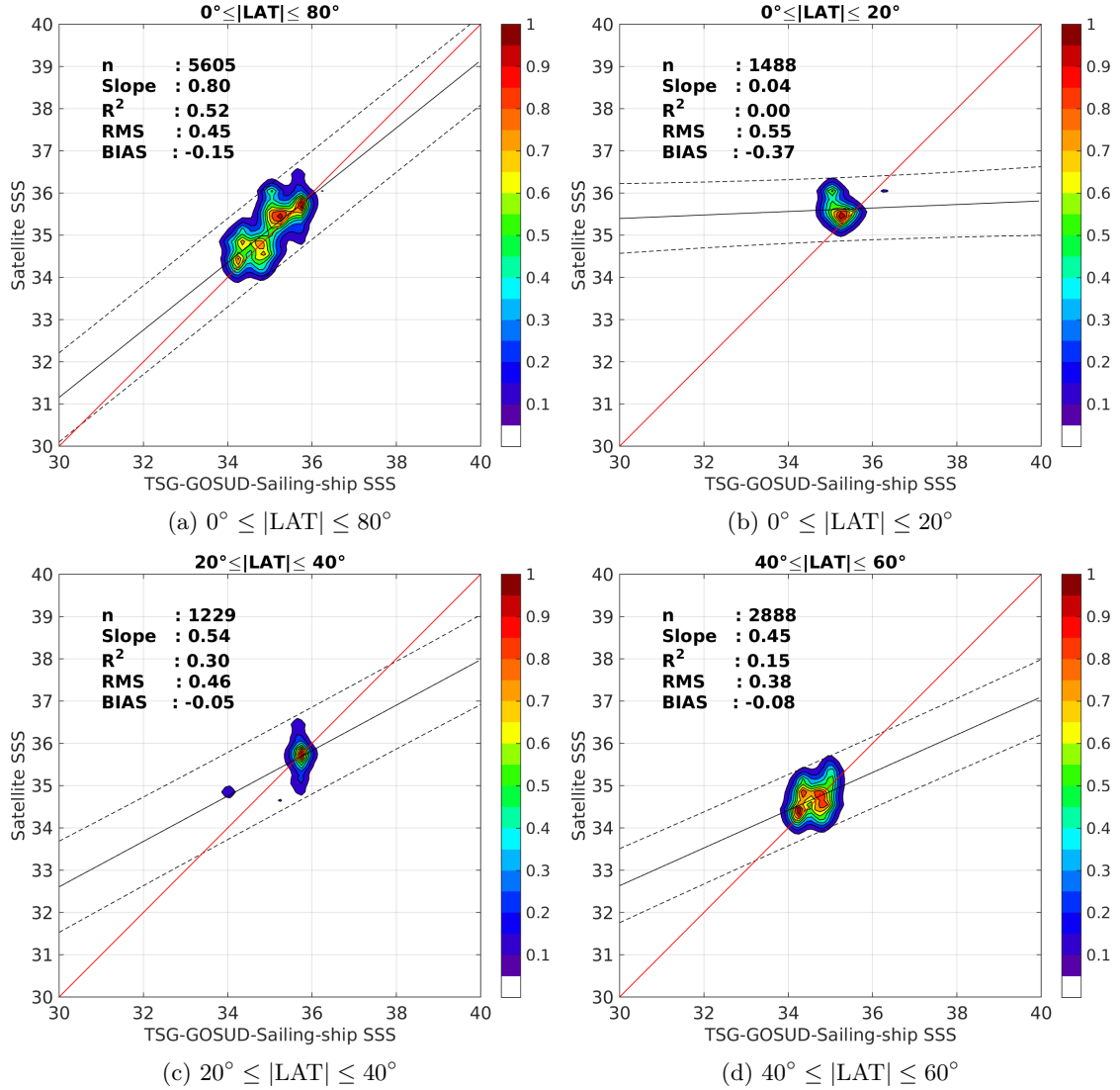
Figure 9: Contour maps of the concentration of SMOS-L3-CATDS-CECOS-IFREMER-V2-1DAY-0.5deg SSS (y-axis) versus TSG-GOSUD-Sailing-ship SSS (x-axis) at match-up pairs for different latitude bands. For each plot, the red line shows x=y . The black thin and dashed lines indicate a linear fit through the data cloud and the \pm 95\% confidence levels, respectively. The number match-up pairs n , the slope and R^2 coefficient of the linear fit, the root mean square (RMS) and the mean bias between satellite and in situ data are indicated for each latitude band in each plots.
