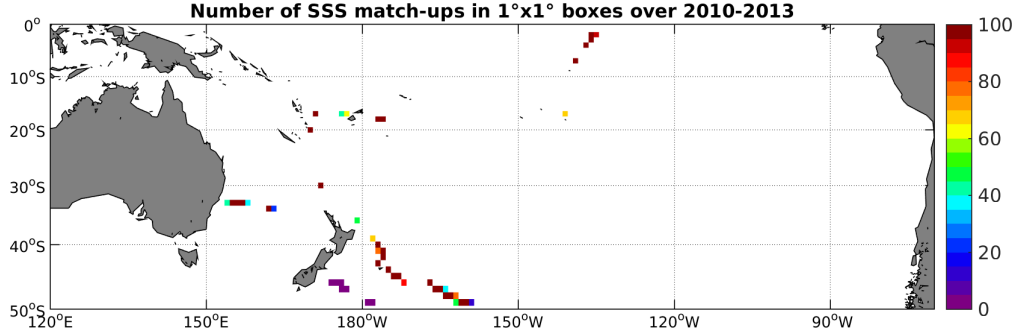
Figure 4: Number of SSS match-ups between TSG-GOSUD-Sailing-ship SSS and the SMOS-L3-CATDS-CECOS-IFREMER-V2-1DAY-0.5deg SSS product for the South Pacific Ocean Pi-MEP region over 1°x1° boxes and for the full satellite product period.
