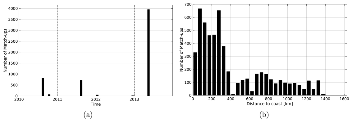
Figure 1: Number of match-ups between TSG-GOSUD-Sailing-ship and SMOS-L3-CATDS-CECOS-IFREMER-V2-1DAY-0.5deg SSS as a function of time (a) and as function of the distance to coast (b) over the South Pacific Ocean Pi-MEP region and for the full satellite product period.
