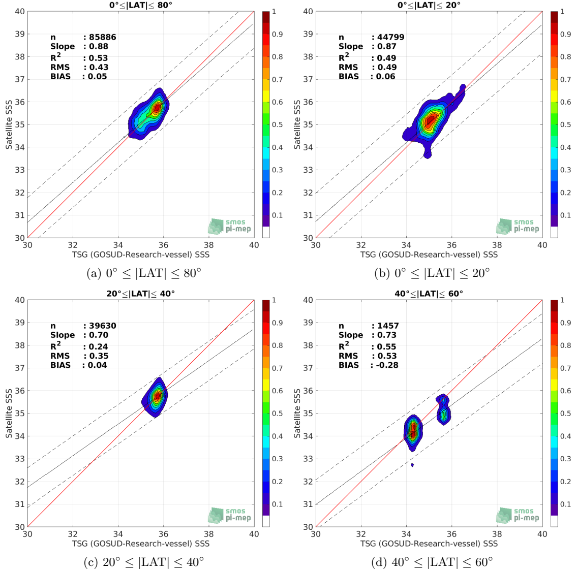
Figure 9: Contour maps of the concentration of SMOS SSS L3 v2 - Daily - 0.5 Deg (CATDS-CECOS-IFREMER) SSS (y-axis) versus TSG (GOSUD-Research-vessel) SSS (x-axis) at match-up pairs for different latitude bands. For each plot, the red line shows x=y . The black thin and dashed lines indicate a linear fit through the data cloud and the \pm 95\% confidence levels, respectively. The number match-up pairs n , the slope and R^2 coefficient of the linear fit, the root mean square (RMS) and the mean bias between satellite and in situ data are indicated for each latitude band in each plots.
