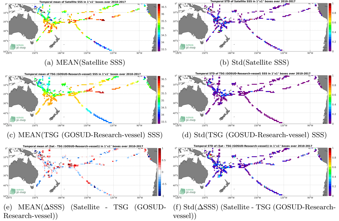
Figure 6: Temporal mean (left) and Std (right) of SSS from SMOS SSS L3 v2 - Daily - 0.5 Deg (CATDS-CECOS-IFREMER) (top), TSG (GOSUD-Research-vessel) (middle), and of \Delta SSS (Satellite - TSG (GOSUD-Research-vessel)). Only match-up pairs are used to generate these maps.
