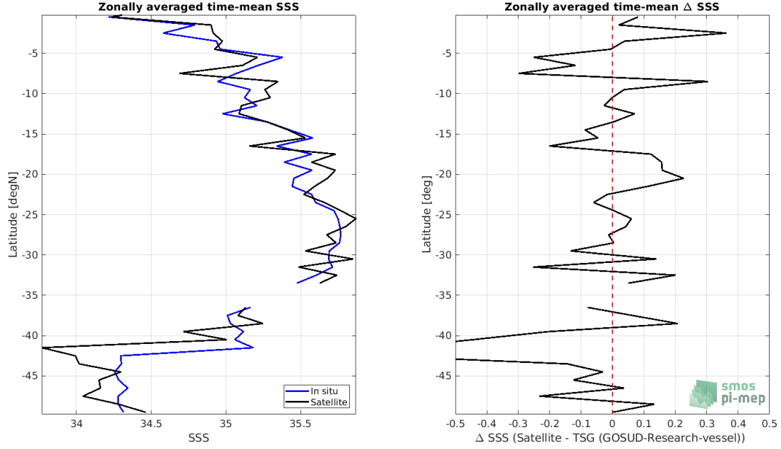
Figure 8: Left panel: Zonal mean SSS from SMOS SSS L3 v2 - Daily - 0.5 Deg (CATDS-CECOS-IFREMER) satellite product (black) and from TSG (GOSUD-Research-vessel) (blue). Right panel: Zonal mean of \Delta SSS (Satellite - TSG (GOSUD-Research-vessel)) for all the collected Pi-MEP match-up pairs estimated over the full satellite product period.
