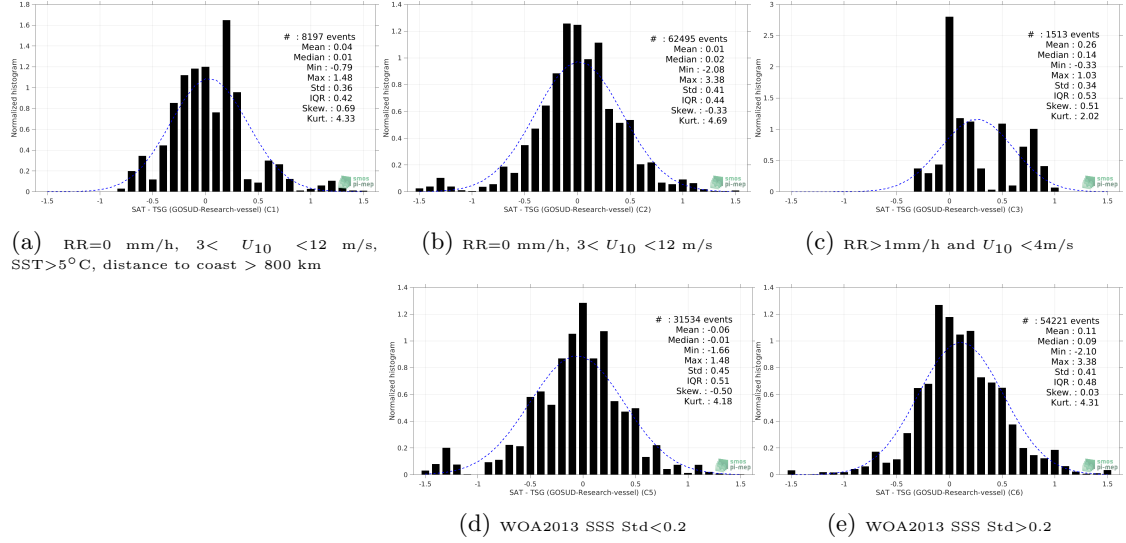
Figure 13: Normalized histogram of \Delta SSS (SMOS SSS L3 v2 - Daily - 0.5 Deg (CATDS-CECOS-IFREMER) - TSG (GOSUD-Research-vessel)) for 5 different subdatasets corresponding to: RR=0 mm/h, 3 < U_{10} < 12 m/s, SST > 5°C, distance to coast > 800 km (a), RR=0 mm/h, 3 < U_{10} < 12 m/s (b), RR > 1mm/h and U_{10} < 4 m/s (c), WOA2013 SSS Std < 0.2 (d), WOA2013 SSS Std > 0.2 (e).
