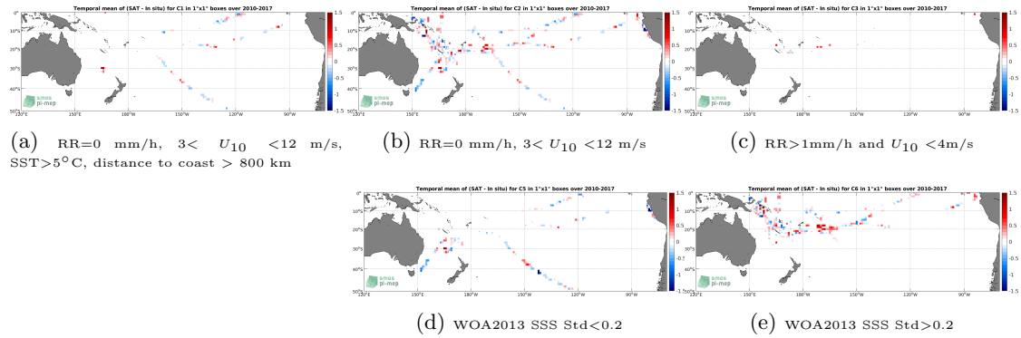
Figure 12: Temporal mean gridded over spatial boxes of size 1^\circ \times 1^\circ of \Delta SSS (SMOS SSS L3 v2 - Daily - 0.5 Deg (CATDS-CECOS-IFREMER) - TSG (GOSUD-Research-vessel)) for 5 different subdatasets corresponding to: RR=0 mm/h, 3 < U_{10} < 12 m/s, SST > 5^\circ\text{C} , distance to coast > 800 km (a), RR=0 mm/h, 3 < U_{10} < 12 m/s (b), RR > 1 mm/h and U_{10} < 4 m/s (c), WOA2013 SSS Std < 0.2 (d), WOA2013 SSS Std > 0.2 (e).
