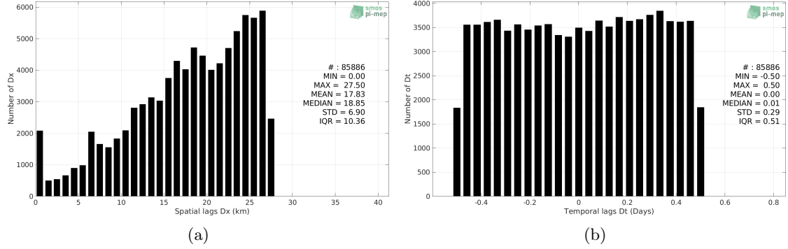
Figure 5: Histograms of the spatial (a) and temporal (b) lags between the location/time of the TSG (GOSUD-Research-vessel) measurement and the date of the corresponding SMOS SSS L3 v2 - Daily - 0.5 Deg (CATDS-CECOS-IFREMER) SSS pixel.
