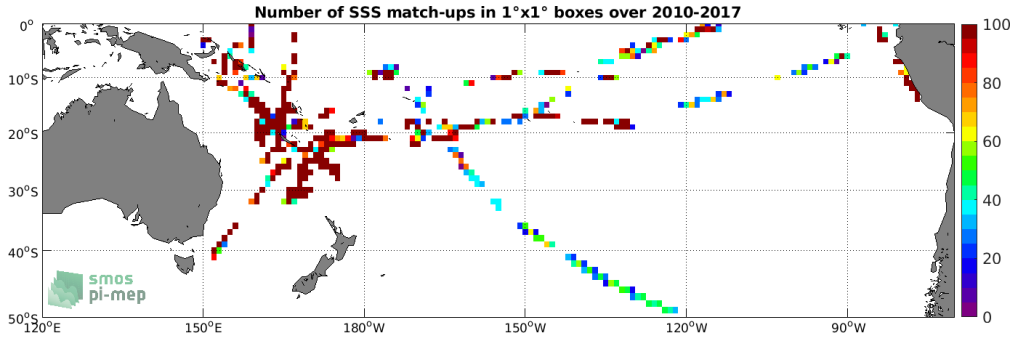
Figure 4: Number of SSS match-ups between TSG (GOSUD-Research-vessel) SSS and the SMOS SSS L3 v2 - Daily - 0.5 Deg (CATDS-CECOS-IFREMER) SSS product for the South Pacific Ocean Pi-MEP region over 1^\circ \times 1^\circ boxes and for the full satellite product period.
