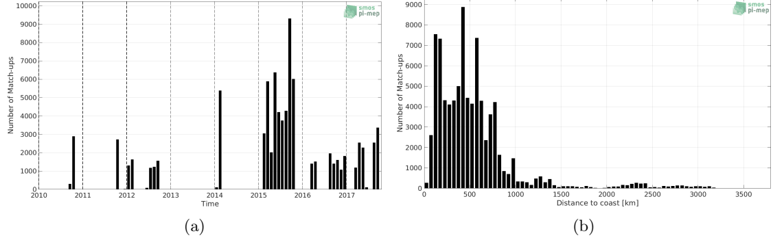
Figure 1: Number of match-ups between TSG (GOSUD-Research-vessel) and SMOS SSS L3 v2 - Daily - 0.5 Deg (CATDS-CECOS-IFREMER) SSS as a function of time (a) and as function of the distance to coast (b) over the South Pacific Ocean Pi-MEP region and for the full satellite product period.
