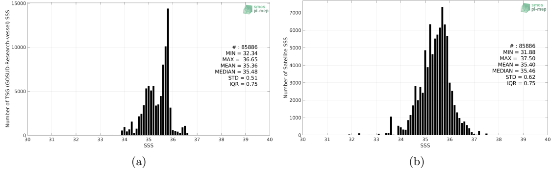
Figure 2: Histograms of SSS from TSG (GOSUD-Research-vessel) (a) and SMOS SSS L3 v2 - Daily - 0.5 Deg (CATDS-CECOS-IFREMER) (b) considering all match-up pairs per bins of 0.1 over the South Pacific Ocean Pi-MEP region and for the full satellite product period.
