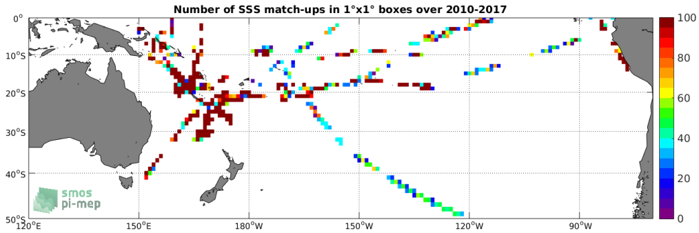
Figure 4: Number of SSS match-ups between TSG-GOSUD-Research-vessel SSS and the SMOS L3 v2 - Daily - 0.5 Deg (CATDS-CECOS-IFREMER) SSS product for the South Pacific Ocean Pi-MEP region over 1°x1° boxes and for the full satellite product period.
