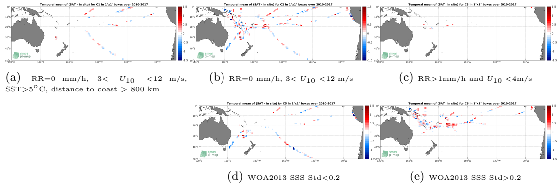
Figure 12: Temporal mean gridded over spatial boxes of size 1^\circ \times 1^\circ of \Delta SSS (SMOS L3 v2 - Daily - 0.5^\circ Deg (CATDS-CECOS-IFREMER) - TSG-GOSUD-Research-vessel) for 5 different subdatasets corresponding to: RR=0 mm/h, 3 < U_{10} < 12 m/s, SST > 5^\circ\text{C} , distance to coast > 800 km (a), RR=0 mm/h, 3 < U_{10} < 12 m/s (b), RR > 1 mm/h and U_{10} < 4 m/s (c), WOA2013 SSS Std < 0.2 (d), WOA2013 SSS Std > 0.2 (e).
