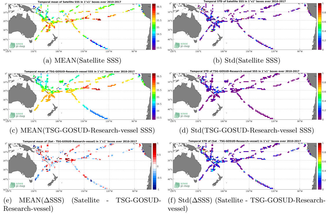
Figure 6: Temporal mean (left) and Std (right) of SSS from SMOS L3 v2 - Daily - 0.5 Deg (CATDS-CECOS-IFREMER) (top), TSG-GOSUD-Research-vessel (middle), and of \Delta SSS (Satellite - TSG-GOSUD-Research-vessel). Only match-up pairs are used to generate these maps.
