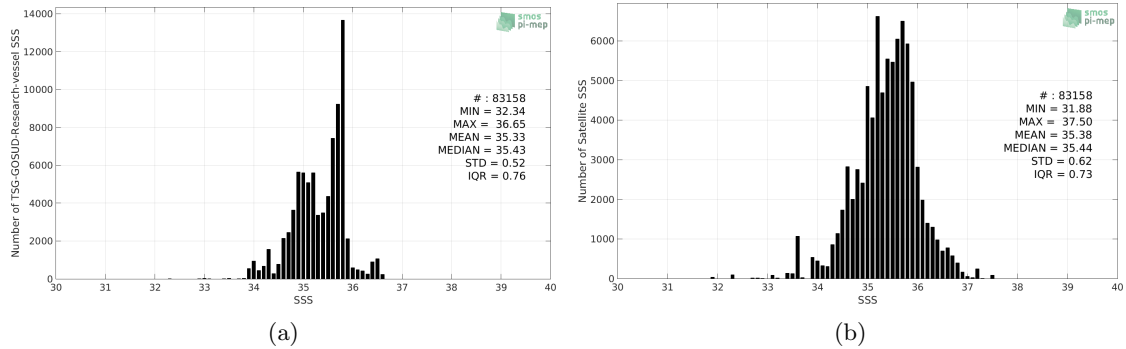
Figure 2: Histograms of SSS from TSG-GOSUD-Research-vessel (a) and SMOS L3 v2 - Daily - 0.5 Deg (CATDS-CECOS-IFREMER) (b) considering all match-up pairs per bins of 0.1 over the South Pacific Ocean Pi-MEP region and for the full satellite product period.
