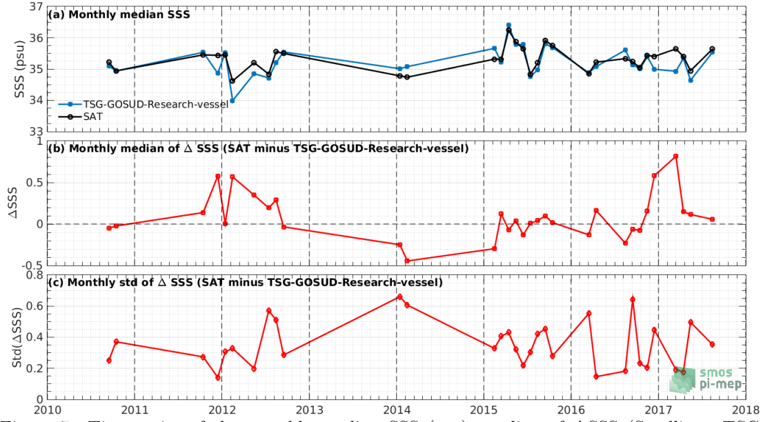
Figure 7: Time series of the monthly median SSS (top), median of \Delta\text{SSS} (Satellite - TSG-GOSUD-Research-vessel) and Std of \Delta\text{SSS} (Satellite - TSG-GOSUD-Research-vessel) over the South Pacific Ocean Pi-MEP region considering all match-ups collected by the Pi-MEP.
