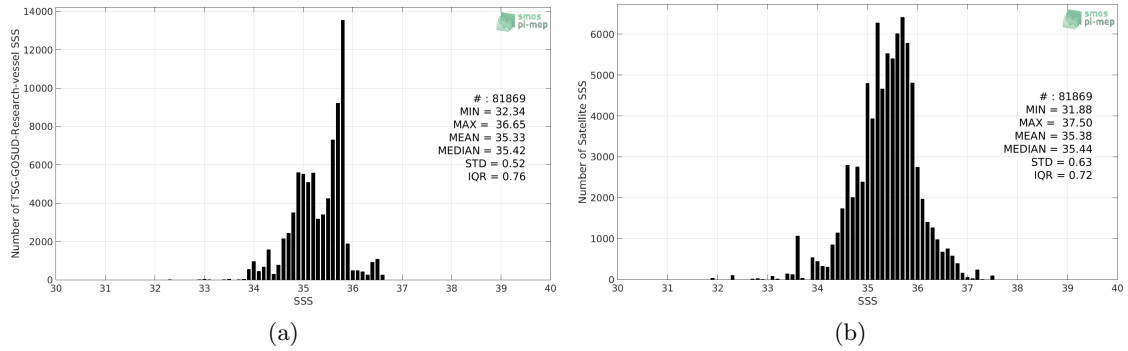
Figure 2: Histograms of SSS from TSG-GOSUD-Research-vessel (a) and SMOS-L3-CATDS-CECOS-IFREMER-V2-1DAY-0.5DEG (b) considering all match-up pairs per bins of 0.1 over the South Pacific Ocean Pi-MEP region and for the full satellite product period.
