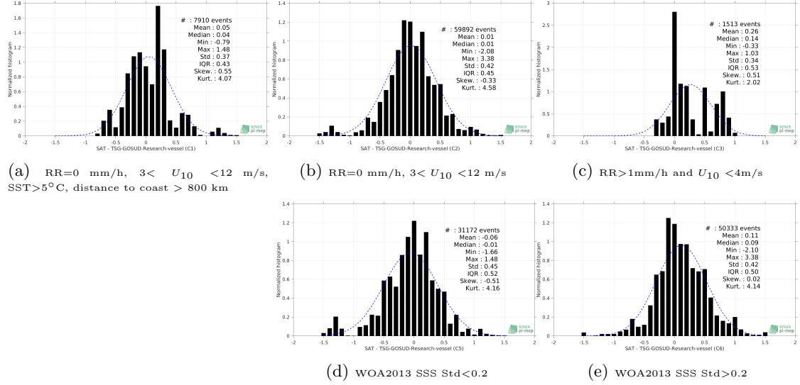
Figure 13: Normalized histogram of \Delta SSS (SMOS-L3-CATDS-CECOS-IFREMER-V2-1DAY-0.5DEG - TSG-GOSUD-Research-vessel) for 5 different subdatasets corresponding to: RR=0 mm/h, 3 < U_{10} < 12 m/s, SST > 5°C, distance to coast > 800 km (a), RR=0 mm/h, 3 < U_{10} < 12 m/s (b), RR > 1 mm/h and U_{10} < 4 m/s (c), WOA2013 SSS Std < 0.2 (d), WOA2013 SSS Std > 0.2 (e).
