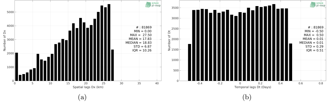
Figure 5: Histograms of the spatial (a) and temporal (b) lags between the time of the TSG-GOSUD-Research-vessel measurements and the date of the corresponding SMOS-L3-CATDS-CECOS-IFREMER-V2-1DAY-0.5DEG SSS product.
