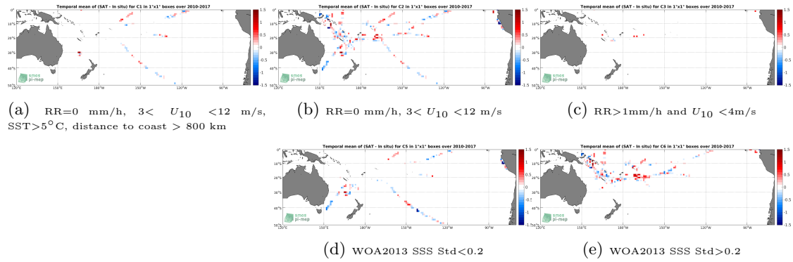
Figure 12: Temporal mean gridded over spatial boxes of size 1^\circ \times 1^\circ of \Delta SSS (SMOS-L3-CATDS-CECOS-IFREMER-V2-1DAY-0.5DEG - TSG-GOSUD-Research-vessel) for 5 different subdatasets corresponding to:RR=0 mm/h, 3 < U_{10} < 12 m/s, SST >5^\circ\text{C} , distance to coast > 800 km (a), RR=0 mm/h, 3 < U_{10} < 12 m/s (b), RR >1 mm/h and U_{10} < 4 m/s (c), WOA2013 SSS Std <0.2 (d), WOA2013 SSS Std >0.2 (e).
