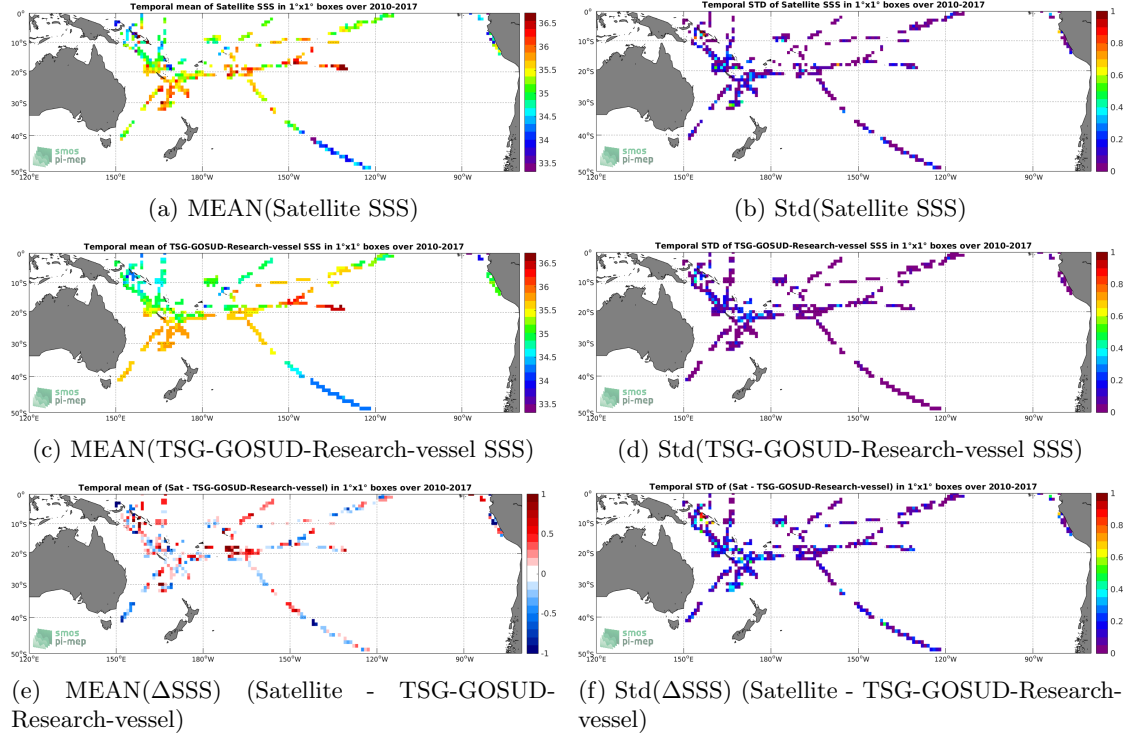
Figure 6: Temporal mean (left) and Std (right) of SSS from SMOS-L3-CATDS-CECOS-IFREMER-V2-1DAY-0.5DEG (top), TSG-GOSUD-Research-vessel (middle), and of \Delta SSS (Satellite - TSG-GOSUD-Research-vessel). Only match-up pairs are used to generate these maps.
