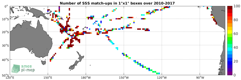
Figure 4: Number of SSS match-ups between TSG-GOSUD-Research-vessel SSS and the SMOS-L3-CATDS-CECOS-IFREMER-V2-1DAY-0.5DEG SSS product for the South Pacific Ocean Pi-MEP region over 1^\circ \times 1^\circ boxes and for the full satellite product period.
