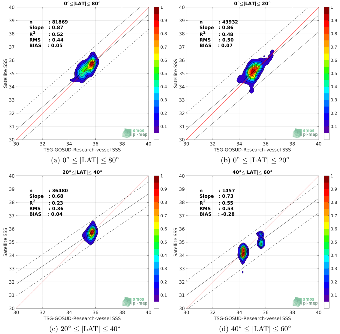
Figure 9: Contour maps of the concentration of SMOS-L3-CATDS-CECOS-IFREMER-V2-1DAY-0.5DEG SSS (y-axis) versus TSG-GOSUD-Research-vessel SSS (x-axis) at match-up pairs for different latitude bands. For each plot, the red line shows x=y . The black thin and dashed lines indicate a linear fit through the data cloud and the \pm 95\% confidence levels, respectively. The number match-up pairs n , the slope and R^2 coefficient of the linear fit, the root mean square (RMS) and the mean bias between satellite and in situ data are indicated for each latitude band in each plots.
