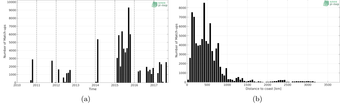
Figure 1: Number of match-ups between TSG-GOSUD-Research-vessel and SMOS-L3-CATDS-CECOS-IFREMER-V2-1DAY-0.5DEG SSS as a function of time (a) and as function of the distance to coast (b) over the South Pacific Ocean Pi-MEP region and for the full satellite product period.
