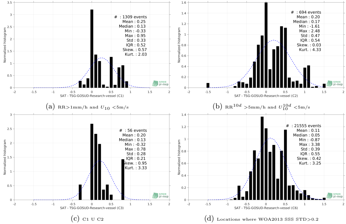
Figure 13: Normalized histogram of \Delta SSS (SMOS-L3-CATDS-CECOS-IFREMER-V2-1DAY-0.5DEG - TSG-GOSUD-Research-vessel) for 6 different subdatasets corresponding to: RR > 1\text{mm/h} and U_{10} < 5\text{m/s} (a), RR^{10d} > 5\text{mm/h} and U_{10}^{10d} < 5\text{m/s} (b), C1 U C2 (c), Locations where WOA2013 SSS STD > 0.2 (d).
