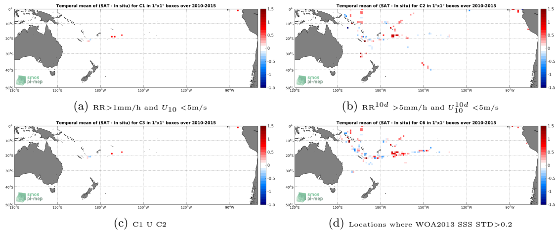
Figure 12: Temporal mean gridded over spatial boxes of size 1^\circ \times 1^\circ of \Delta SSS (SMOS-L3-CATDS-CECOS-IFREMER-V2-1DAY-0.5DEG - TSG-GOSUD-Research-vessel) for 4 different subdatasets corresponding to: RR > 1\text{mm/h} and U_{10} < 5\text{m/s} (a), RR^{10d} > 5\text{mm/h} and U_{10}^{10d} < 5\text{m/s} (b), C1 U C2 (c), Locations where WOA2013 SSS STD > 0.2 (d).
